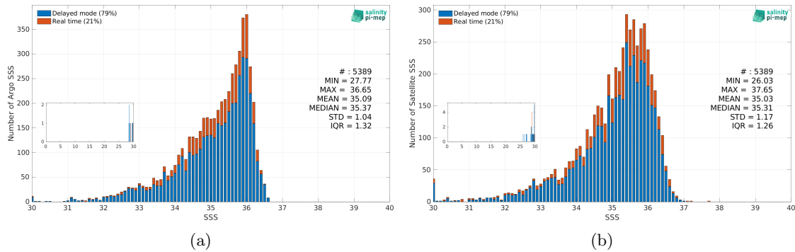
Figure 2: Histograms of SSS from Argo (a) and SMOS SSS L3 v9 - 9 Days (CATDS-CEC-LOCEAN) (b) considering all match-up pairs per bins of 0.1 over the Congo river plume Pi-MEP region and for the full satellite product period.
