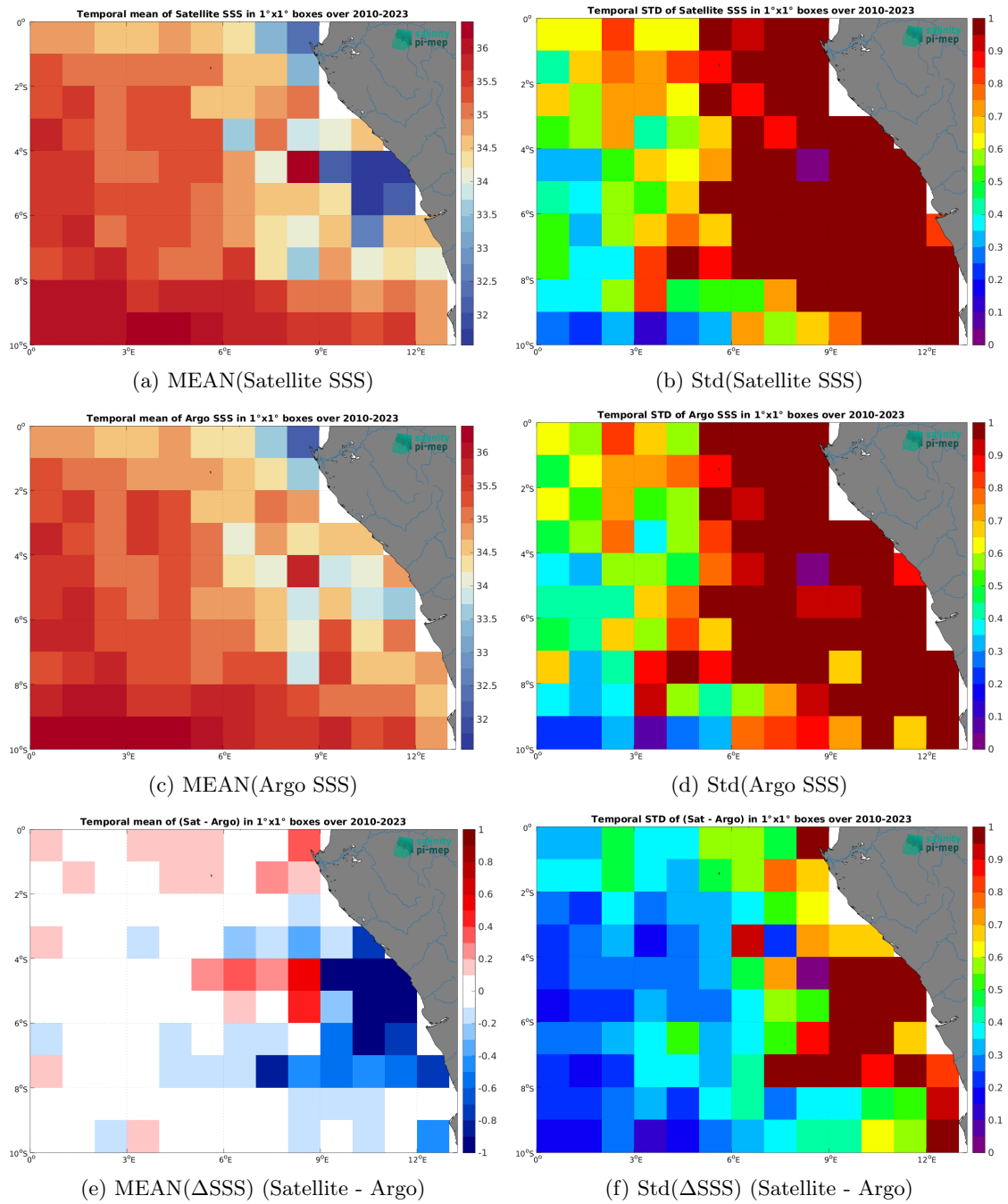
Figure 6: Temporal mean (left) and Std (right) of SSS from SMOS SSS L3 v9 - 9 Days (CATDS-CEC-LOCEAN) (top), Argo (middle), and of \Delta SSS (Satellite - Argo). Only match-up pairs are used to generate these maps.
