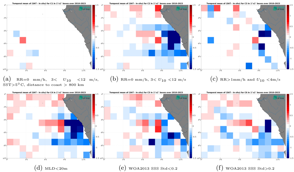
Figure 12: Temporal mean gridded over spatial boxes of size 1^\circ \times 1^\circ of \Delta SSS (SMOS SSS L3 v9 - 9 Days (CATDS-CEC-LOCEAN) - Argo) for 6 different subdatasets corresponding to:RR=0 mm/h, 3 < U_{10} < 12 m/s, SST > 5^\circ\text{C} , distance to coast > 800 km (a), RR=0 mm/h, 3 < U_{10} < 12 m/s (b), RR > 1 mm/h and U_{10} < 4 m/s (c),MLD < 20 m (d),WOA2013 SSS Std < 0.2 (e),WOA2013 SSS Std > 0.2 (f).
