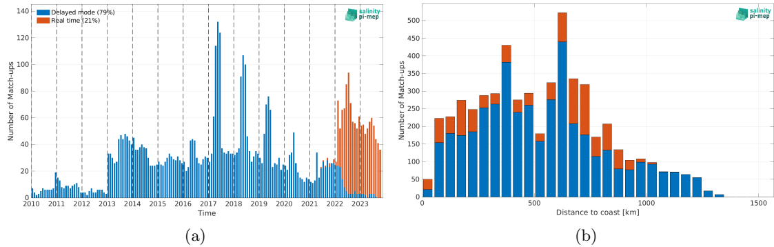
Figure 1: Number of match-ups between Argo and SMOS SSS L3 v9 - 9 Days (CATDS-CEC-LOCEAN) SSS as a function of time (a) and as function of the distance to coast (b) over the Congo river plume Pi-MEP region and for the full satellite product period.
