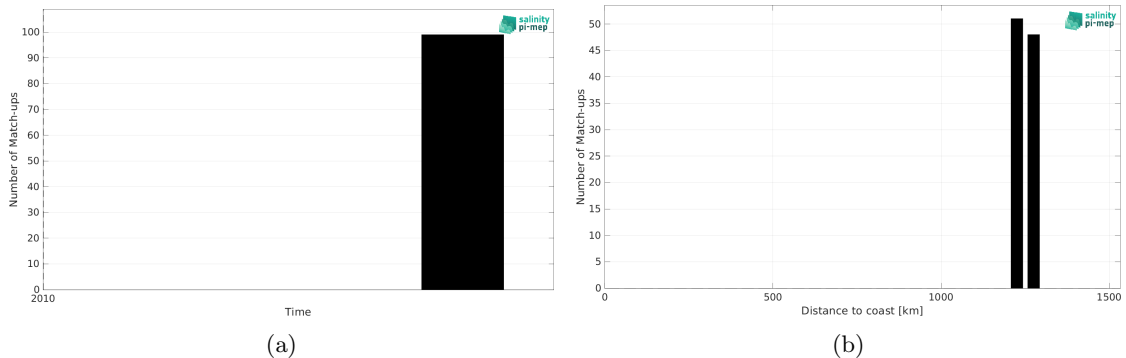
Figure 2: Number of match-ups between TSG (SAMOS) and SMOS SSS L3 v9 - 18 Days (CATDS-CEC-LOCEAN) SSS as a function of time (a) and as function of the distance to coast (b) over the Congo river plume Pi-MEP region and for the full satellite product period.
