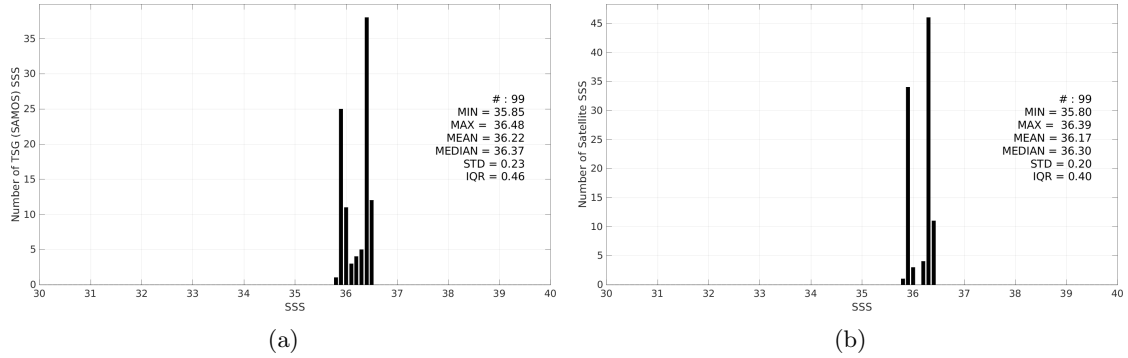
Figure 3: Histograms of SSS from TSG (SAMOS) (a) and SMOS SSS L3 v9 - 18 Days (CATDS-CEC-LOCEAN) (b) considering all match-up pairs per bins of 0.1 over the Congo river plume Pi-MEP region and for the full satellite product period.
