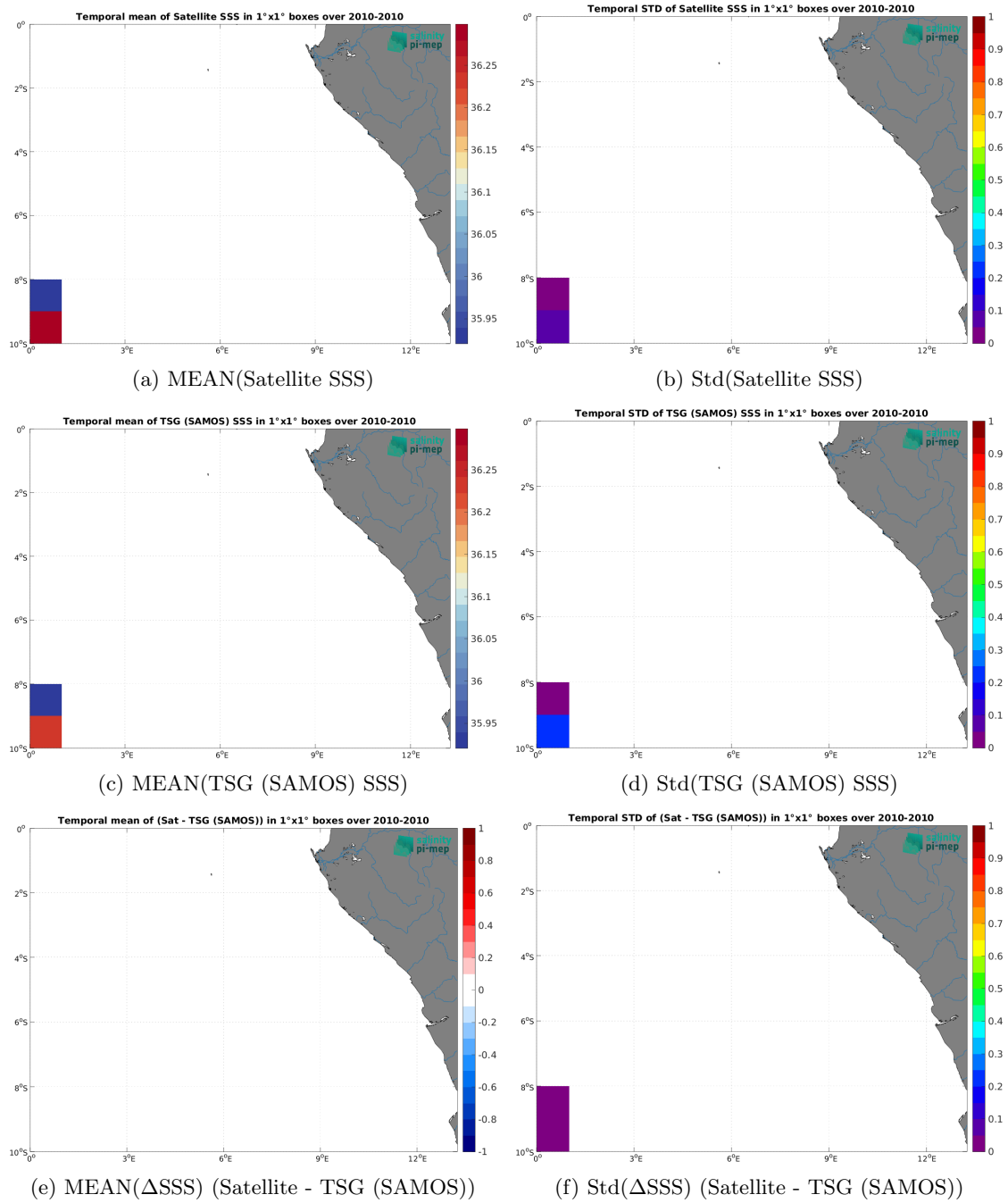
Figure 7: Temporal mean (left) and Std (right) of SSS from SMOS SSS L3 v9 - 18 Days (CATDS-CEC-LOCEAN) (top), TSG (SAMOS) (middle), and of \Delta SSS (Satellite - TSG (SAMOS)). Only match-up pairs are used to generate these maps.
