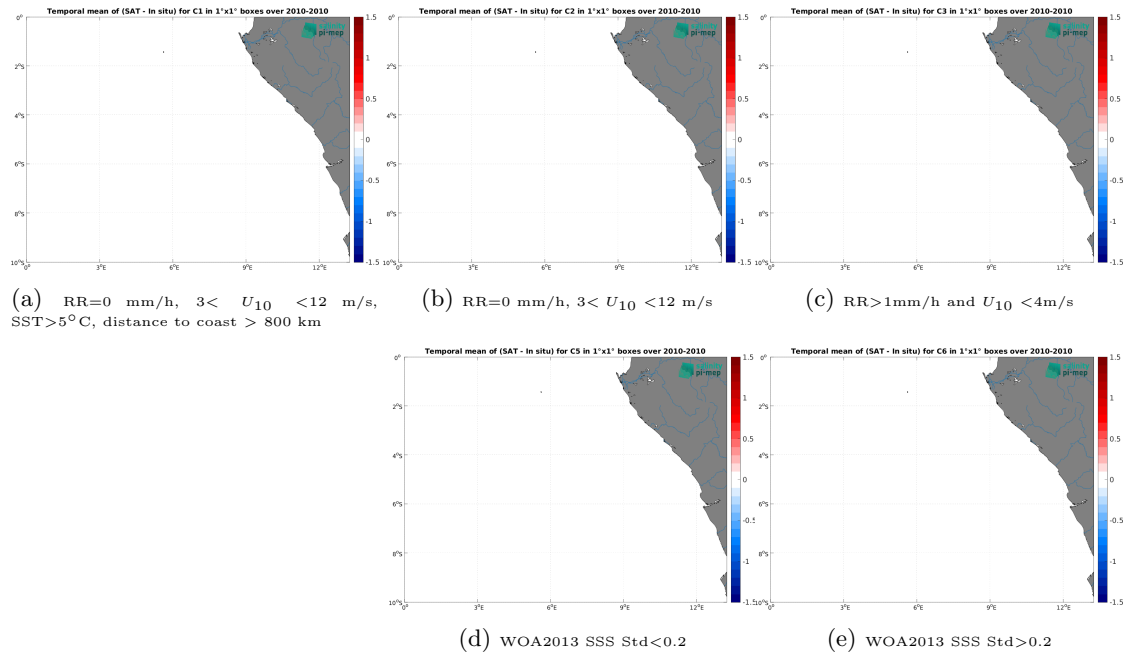
Figure 12: Temporal mean gridded over spatial boxes of size 1^{\circ}\times 1^{\circ} of \Delta\text{SSS} (SMOS SSS L3 v9 - 18 Days (CATDS-CEC-LOCEAN) - TSG (SAMOS)) for 5 different subdatasets corresponding to:RR=0 mm/h, 3 < U_{10} < 12 m/s, SST >5^{\circ}\text{C} , distance to coast > 800 km (a), RR=0 mm/h, 3 < U_{10} < 12 m/s (b), RR >1 mm/h and U_{10} < 4 m/s (c), WOA2013 SSS Std <0.2 (d), WOA2013 SSS Std >0.2 (e).
