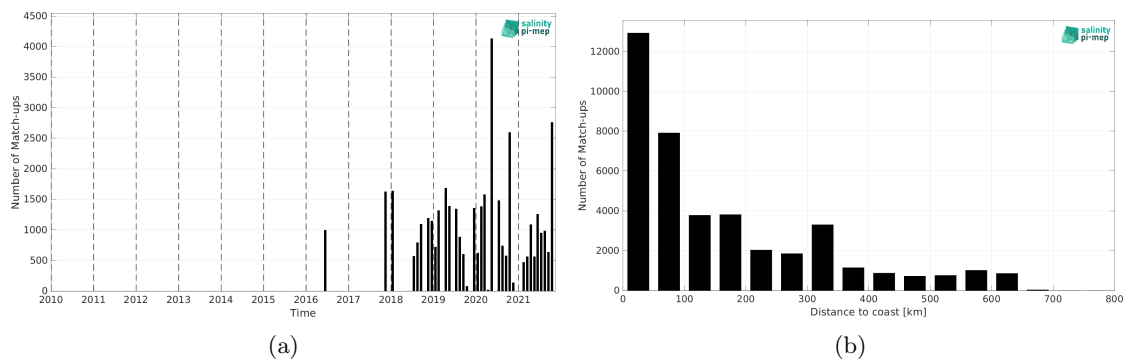
Figure 2: Number of match-ups between TSG (LEGOS-DM) and SMOS SSS L3 v9 - 18 Days (CATDS-CEC-LOCEAN) SSS as a function of time (a) and as function of the distance to coast (b) over the Congo river plume Pi-MEP region and for the full satellite product period.
