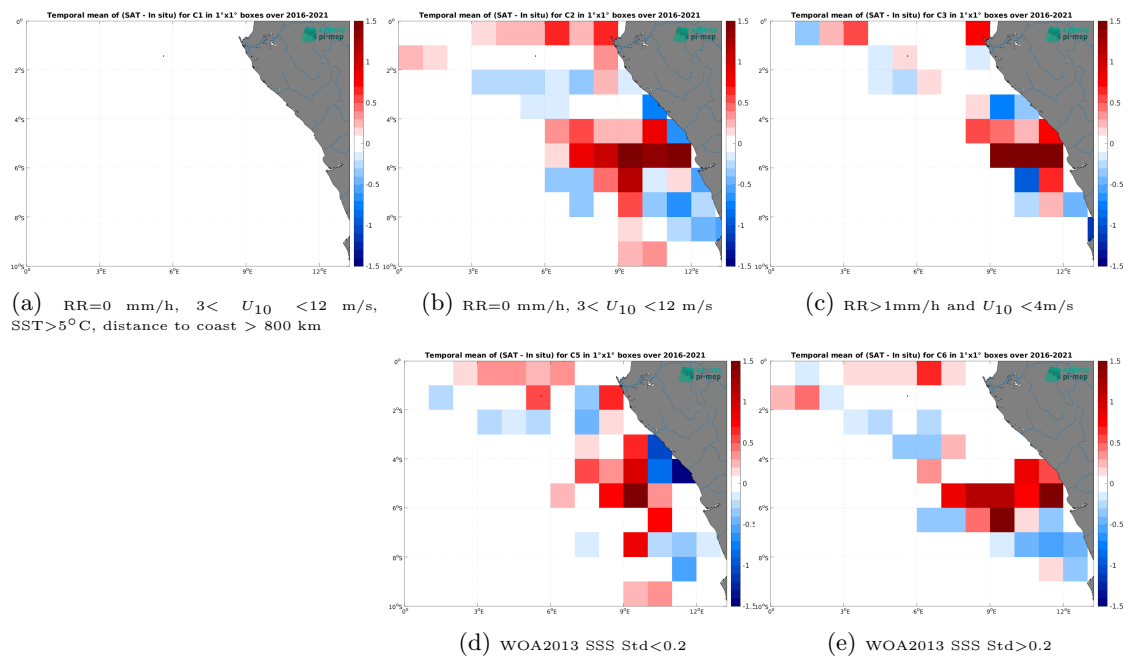
Figure 14: Temporal mean gridded over spatial boxes of size 1^\circ \times 1^\circ of \Delta SSS (SMOS SSS L3 v9 - 18 Days (CATDS-CEC-LOCEAN) - TSG (LEGOS-DM)) for 5 different subdatasets corresponding to: RR=0 mm/h, 3 < U_{10} < 12 m/s, SST > 5°C, distance to coast > 800 km (a), RR=0 mm/h, 3 < U_{10} < 12 m/s (b), RR > 1mm/h and U_{10} < 4 m/s (c), WOA2013 SSS Std < 0.2 (d), WOA2013 SSS Std > 0.2 (e).
