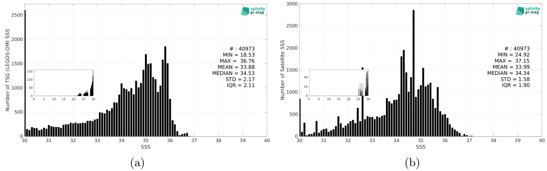
Figure 3: Histograms of SSS from TSG (LEGOS-DM) (a) and SMOS SSS L3 v9 - 18 Days (CATDS-CEC-LOCEAN) (b) considering all match-up pairs per bins of 0.1 over the Congo river plume Pi-MEP region and for the full satellite product period.
