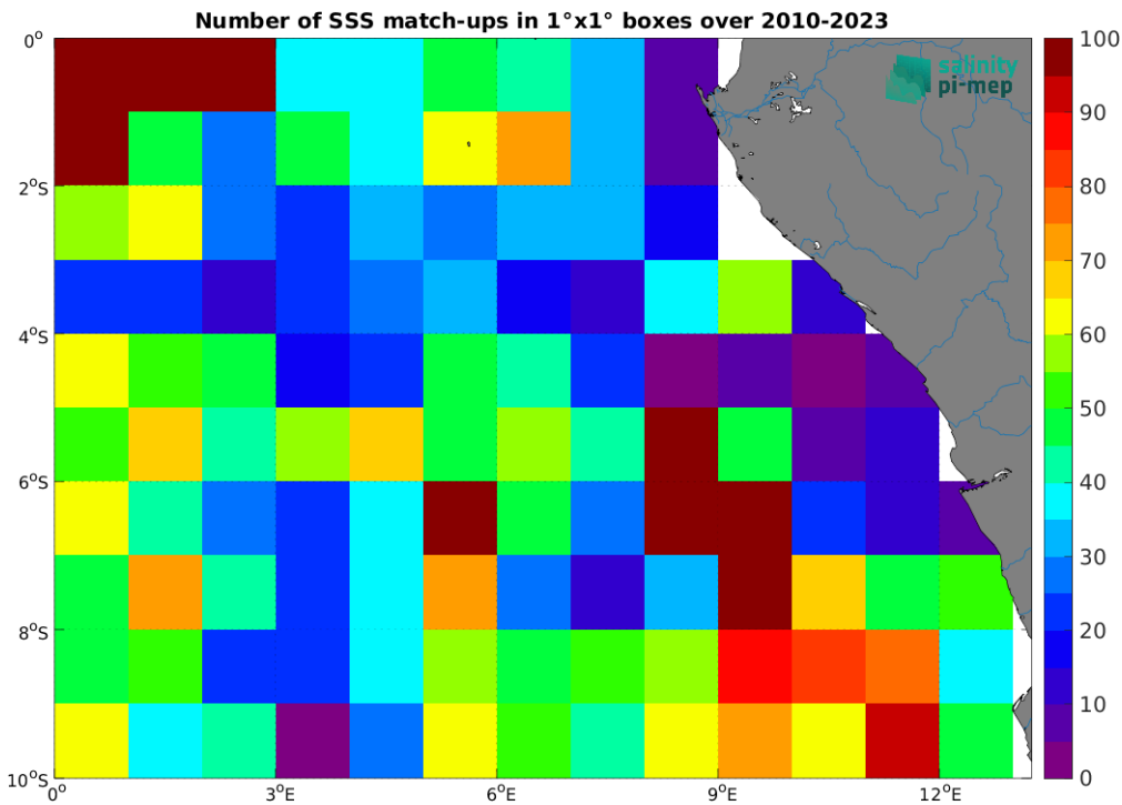
Figure 4: Number of SSS match-ups between Argo SSS and the SMOS SSS L3 v9 - 18 Days (CATDS-CEC-LOCEAN) SSS product for the Congo river plume Pi-MEP region over 1^\circ \times 1^\circ boxes and for the full satellite product period.
