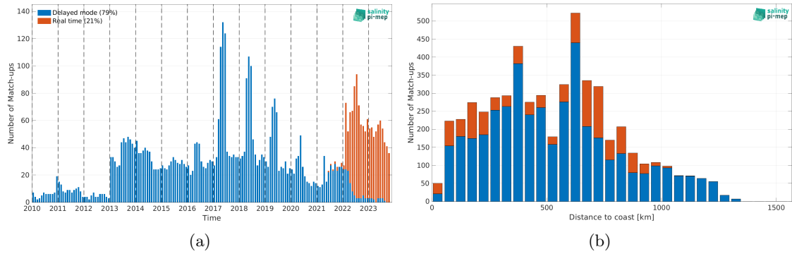
Figure 1: Number of match-ups between Argo and SMOS SSS L3 v9 - 18 Days (CATDS-CEC-LOCEAN) SSS as a function of time (a) and as function of the distance to coast (b) over the Congo river plume Pi-MEP region and for the full satellite product period.
