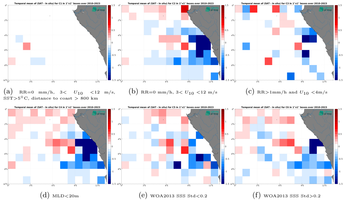
Figure 12: Temporal mean gridded over spatial boxes of size 1^\circ \times 1^\circ of \Delta SSS (SMOS SSS L3 v9 - 18 Days (CATDS-CEC-LOCEAN) - Argo) for 6 different subdatasets corresponding to:RR=0 mm/h, 3 < U_{10} < 12 m/s, SST >5^\circ C, distance to coast > 800 km (a), RR=0 mm/h, 3 < U_{10} < 12 m/s (b), RR >1 mm/h and U_{10} < 4 m/s (c),MLD <20 m (d),WOA2013 SSS Std <0.2 (e),WOA2013 SSS Std >0.2 (f).
