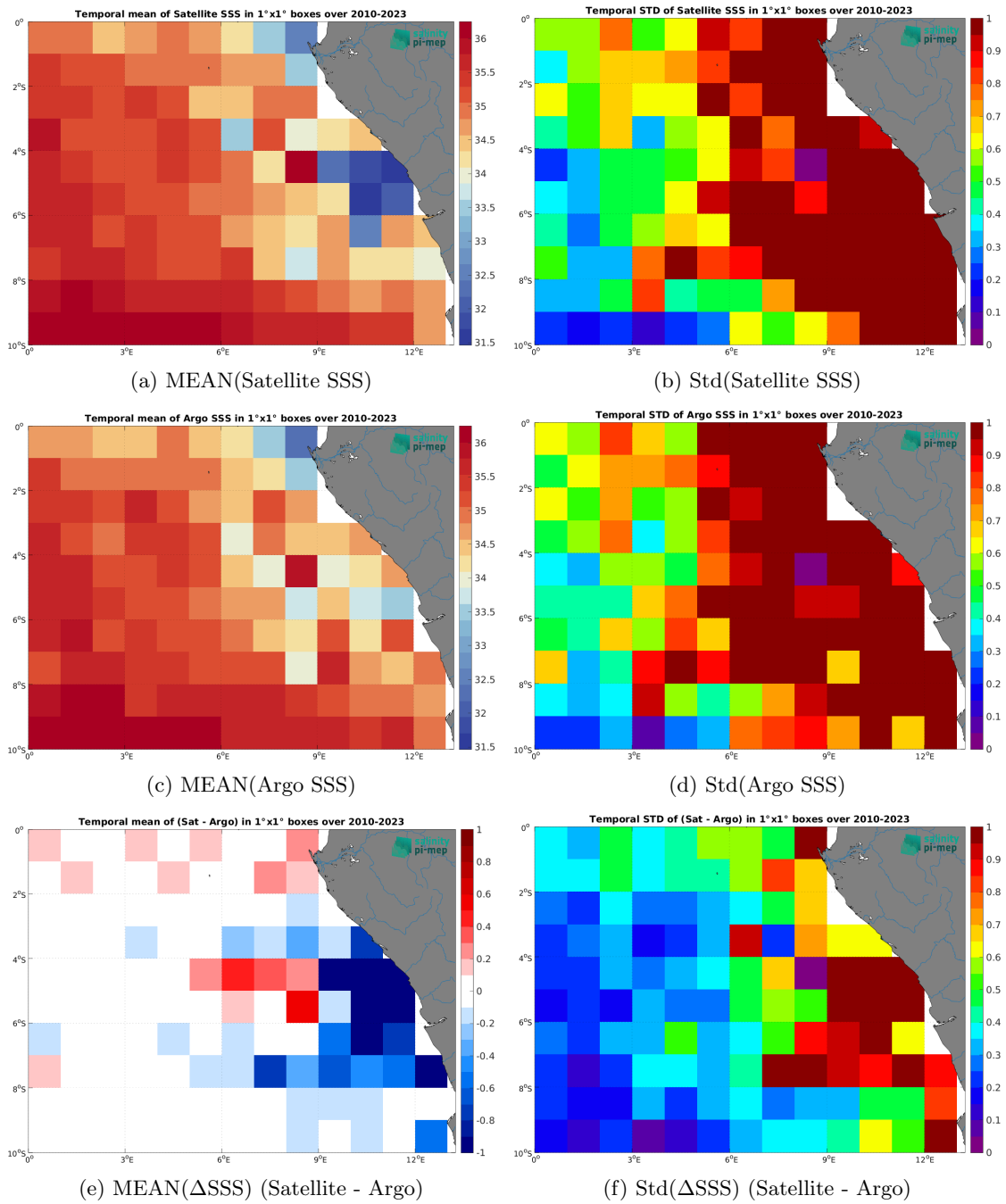
Figure 6: Temporal mean (left) and Std (right) of SSS from SMOS SSS L3 v9 - 18 Days (CATDS-CEC-LOCEAN) (top), Argo (middle), and of \Delta SSS (Satellite - Argo). Only match-up pairs are used to generate these maps.
