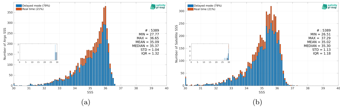
Figure 2: Histograms of SSS from Argo (a) and SMOS SSS L3 v9 - 18 Days (CATDS-CEC-LOCEAN) (b) considering all match-up pairs per bins of 0.1 over the Congo river plume Pi-MEP region and for the full satellite product period.
