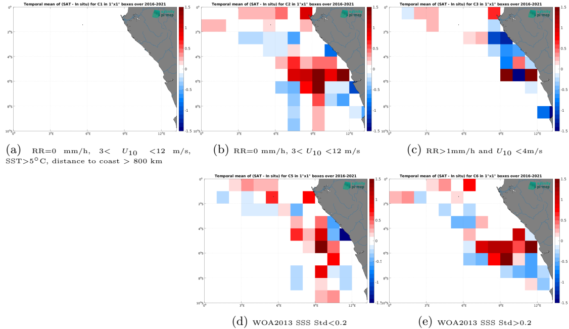
Figure 12: Temporal mean gridded over spatial boxes of size 1^{\circ}\times 1^{\circ} of \Delta\text{SSS} (SMOS SSS L3 v8 - 9 Days (CATDS-CEC-LOCEAN) - TSG (LEGOS-DM)) for 5 different subdatasets corresponding to:RR=0 mm/h, 3 < U_{10} < 12 m/s, SST >5^{\circ}\text{C} , distance to coast > 800 km (a), RR=0 mm/h, 3 < U_{10} < 12 m/s (b), RR >1 mm/h and U_{10} < 4 m/s (c), WOA2013 SSS Std <0.2 (d), WOA2013 SSS Std >0.2 (e).
