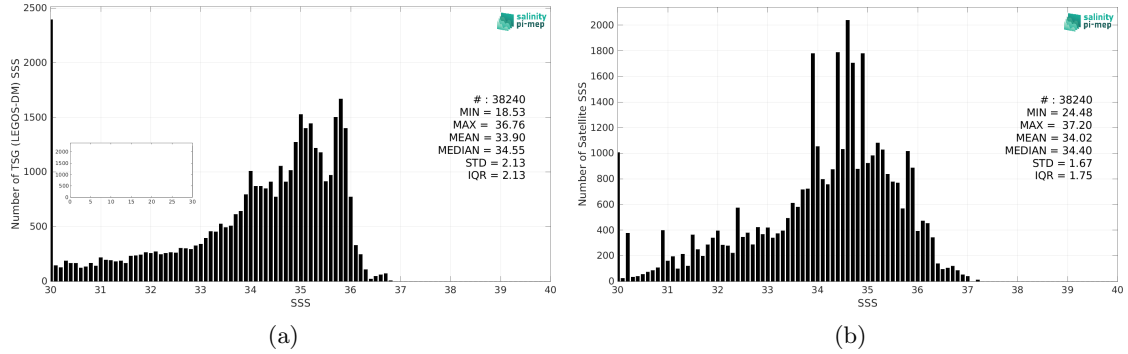
Figure 2: Histograms of SSS from TSG (LEGOS-DM) (a) and SMOS SSS L3 v8 - 9 Days (CATDS-CEC-LOCEAN) (b) considering all match-up pairs per bins of 0.1 over the Congo river plume Pi-MEP region and for the full satellite product period.
