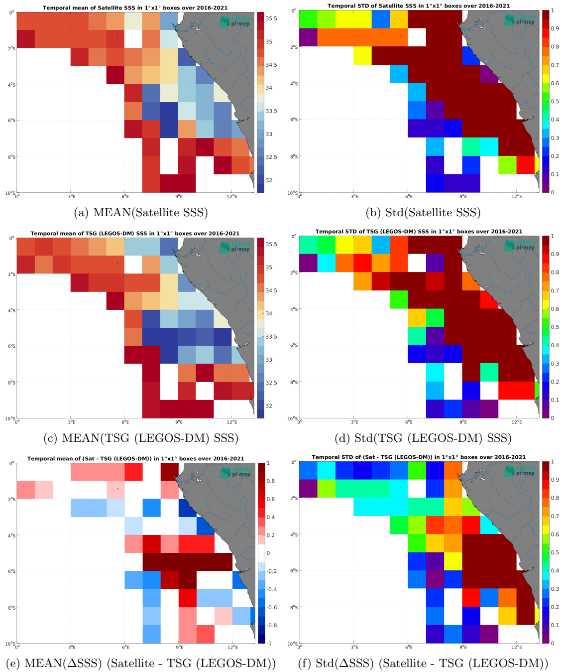
Figure 6: Temporal mean (left) and Std (right) of SSS from SMOS SSS L3 v8 - 9 Days (CATDS-CEC-LOCEAN) (top), TSG (LEGOS-DM) (middle), and of \Delta SSS (Satellite - TSG (LEGOS-DM)). Only match-up pairs are used to generate these maps.
