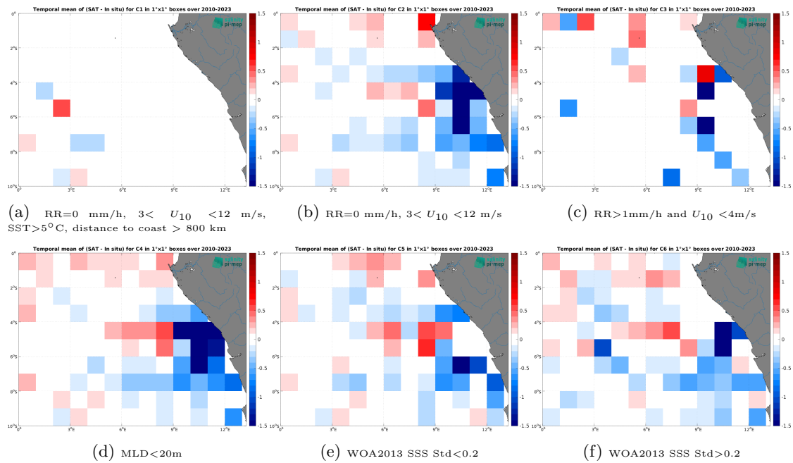
Figure 12: Temporal mean gridded over spatial boxes of size 1^\circ \times 1^\circ of \Delta SSS (SMOS SSS L3 v8 - 9 Days (CATDS-CEC-LOCEAN) - Argo) for 6 different subdatasets corresponding to:RR=0 mm/h, 3 < U_{10} < 12 m/s, SST > 5^\circ\text{C} , distance to coast > 800 km (a), RR=0 mm/h, 3 < U_{10} < 12 m/s (b), RR > 1 mm/h and U_{10} < 4 m/s (c),MLD < 20 m (d),WOA2013 SSS Std < 0.2 (e),WOA2013 SSS Std > 0.2 (f).
