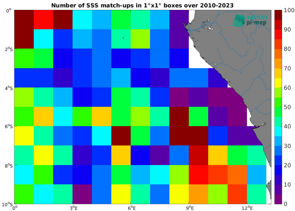
Figure 4: Number of SSS match-ups between Argo SSS and the SMOS SSS L3 v8 - 9 Days (CATDS-CEC-LOCEAN) SSS product for the Congo river plume Pi-MEP region over 1^\circ \times 1^\circ boxes and for the full satellite product period.
