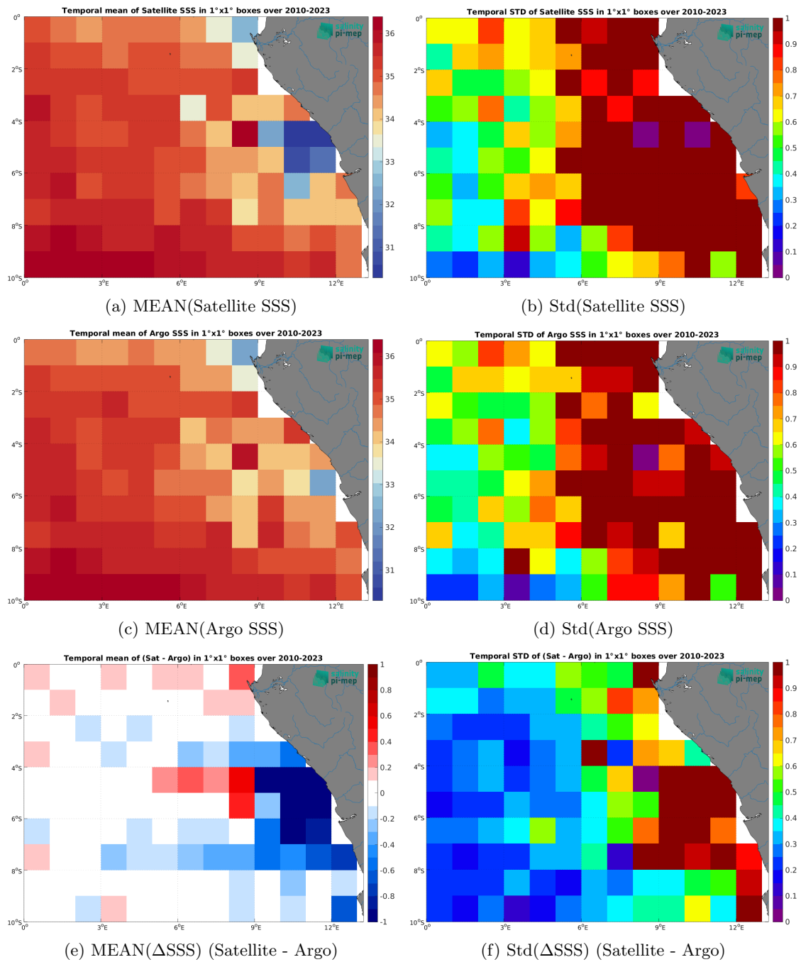
Figure 6: Temporal mean (left) and Std (right) of SSS from SMOS SSS L3 v8 - 9 Days (CATDS-CEC-LOCEAN) (top), Argo (middle), and of \Delta SSS (Satellite - Argo). Only match-up pairs are used to generate these maps.
