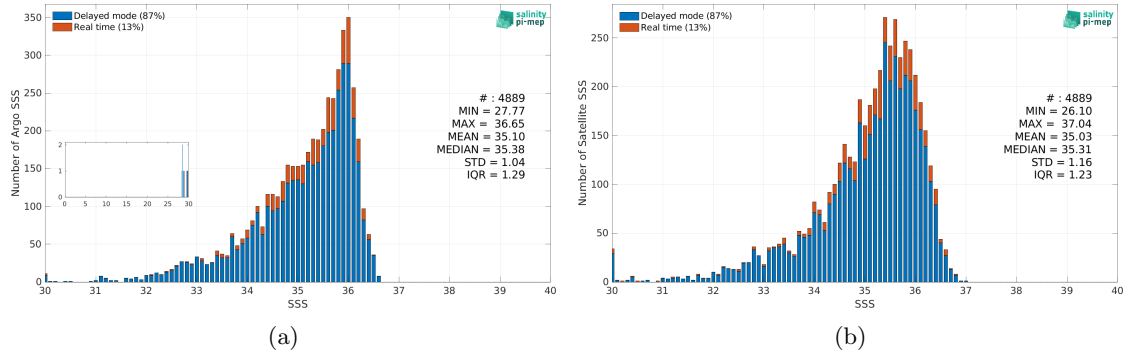
Figure 2: Histograms of SSS from Argo (a) and SMOS SSS L3 v8 - 9 Days (CATDS-CEC-LOCEAN) (b) considering all match-up pairs per bins of 0.1 over the Congo river plume Pi-MEP region and for the full satellite product period.
