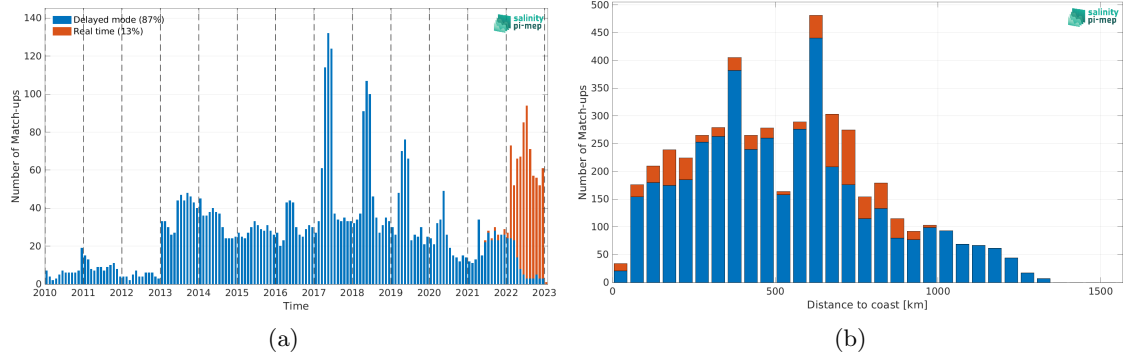
Figure 1: Number of match-ups between Argo and SMOS SSS L3 v8 - 9 Days (CATDS-CEC-LOCEAN) SSS as a function of time (a) and as function of the distance to coast (b) over the Congo river plume Pi-MEP region and for the full satellite product period.
