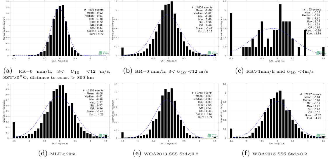
Figure 13: Normalized histogram of \Delta\text{SSS} (SMOS SSS L3 v8 - 9 Days (CATDS-CECOS-LOCEAN) - Argo) for 6 different subdatasets corresponding to: RR=0 mm/h, 3 < U_{10} < 12 m/s, SST>5°C, distance to coast > 800 km (a), RR=0 mm/h, 3 < U_{10} < 12 m/s (b), RR>1mm/h and U_{10} < 4 m/s (c), MLD<20m (d), WOA2013 SSS Std<0.2 (e), WOA2013 SSS Std>0.2 (f).
