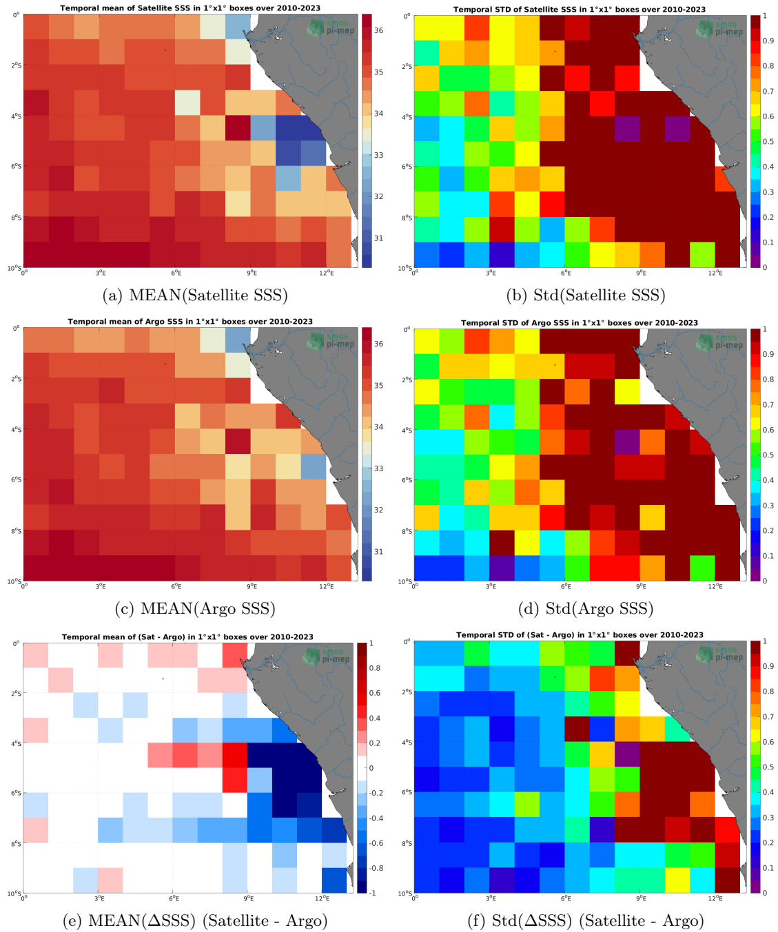
Figure 6: Temporal mean (left) and Std (right) of SSS from SMOS SSS L3 v8 - 9 Days (CATDS-CECOS-LOCEAN) (top), Argo (middle), and of \Delta SSS (Satellite - Argo). Only match-up pairs are used to generate these maps.
