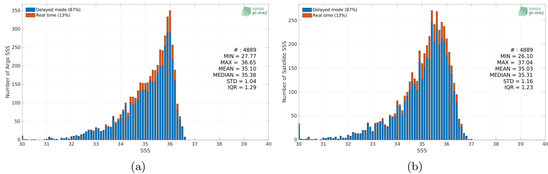
Figure 2: Histograms of SSS from Argo (a) and SMOS SSS L3 v8 - 9 Days (CATDS-CECOS-LOCEAN) (b) considering all match-up pairs per bins of 0.1 over the Congo river plume Pi-MEP region and for the full satellite product period.
