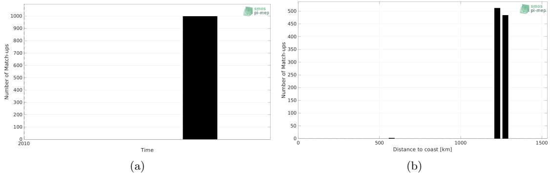
Figure 1: Number of match-ups between TSG (SAMOS) and SMOS SSS L3 v8 - 18 Days (CATDS-CECOS-LOCEAN) SSS as a function of time (a) and as function of the distance to coast (b) over the Congo river plume Pi-MEP region and for the full satellite product period.
