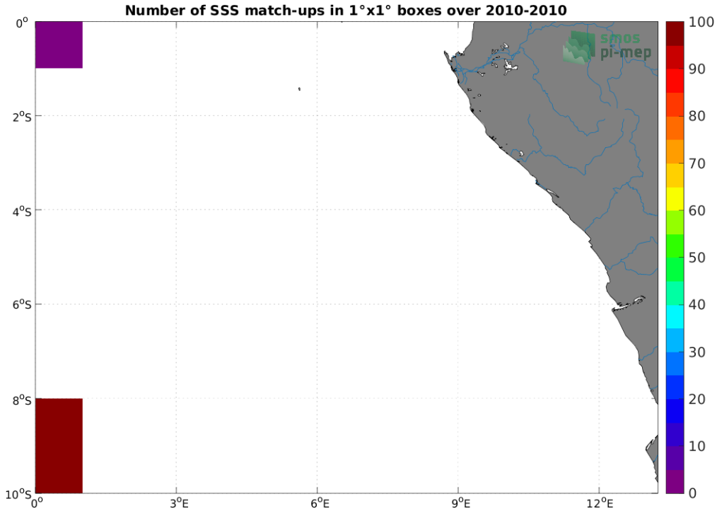
Figure 4: Number of SSS match-ups between TSG (SAMOS) SSS and the SMOS SSS L3 v8 - 18 Days (CATDS-CECOS-LOCEAN) SSS product for the Congo river plume Pi-MEP region over 1^\circ \times 1^\circ boxes and for the full satellite product period.
