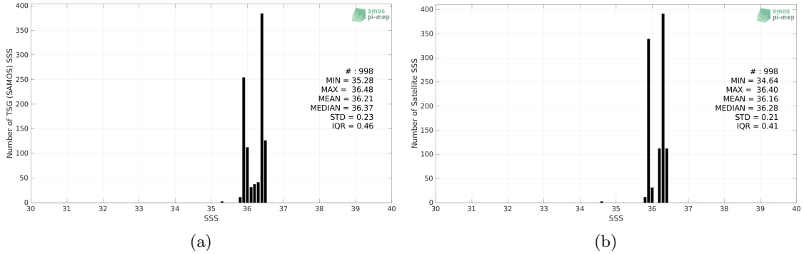
Figure 2: Histograms of SSS from TSG (SAMOS) (a) and SMOS SSS L3 v8 - 18 Days (CATDS-CECOS-LOCEAN) (b) considering all match-up pairs per bins of 0.1 over the Congo river plume Pi-MEP region and for the full satellite product period.
