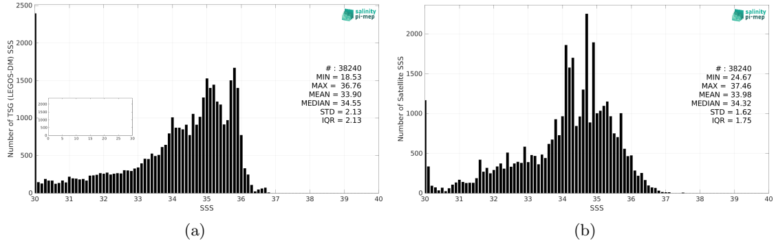
Figure 2: Histograms of SSS from TSG (LEGOS-DM) (a) and SMOS SSS L3 v8 - 18 Days (CATDS-CEC-LOCEAN) (b) considering all match-up pairs per bins of 0.1 over the Congo river plume Pi-MEP region and for the full satellite product period.
