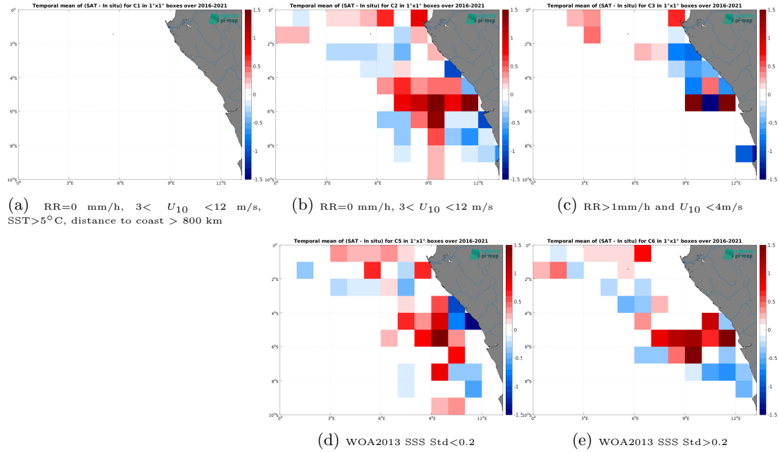
Figure 12: Temporal mean gridded over spatial boxes of size 1^{\circ}\times 1^{\circ} of \Delta\text{SSS} (SMOS SSS L3 v8 - 18 Days (CATDS-CEC-LOCEAN) - TSG (LEGOS-DM)) for 5 different subdatasets corresponding to:RR=0 mm/h, 3 < U_{10} < 12 m/s, SST >5^{\circ}\text{C} , distance to coast > 800 km (a), RR=0 mm/h, 3 < U_{10} < 12 m/s (b), RR >1 mm/h and U_{10} < 4 m/s (c), WOA2013 SSS Std <0.2 (d), WOA2013 SSS Std >0.2 (e).
