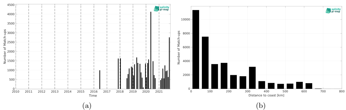
Figure 1: Number of match-ups between TSG (LEGOS-DM) and SMOS SSS L3 v8 - 18 Days (CATDS-CEC-LOCEAN) SSS as a function of time (a) and as function of the distance to coast (b) over the Congo river plume Pi-MEP region and for the full satellite product period.
