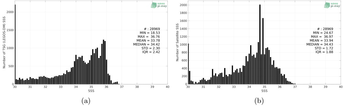
Figure 2: Histograms of SSS from TSG (LEGOS-DM) (a) and SMOS SSS L3 v8 - 18 Days (CATDS-CECOS-LOCEAN) (b) considering all match-up pairs per bins of 0.1 over the Congo river plume Pi-MEP region and for the full satellite product period.
