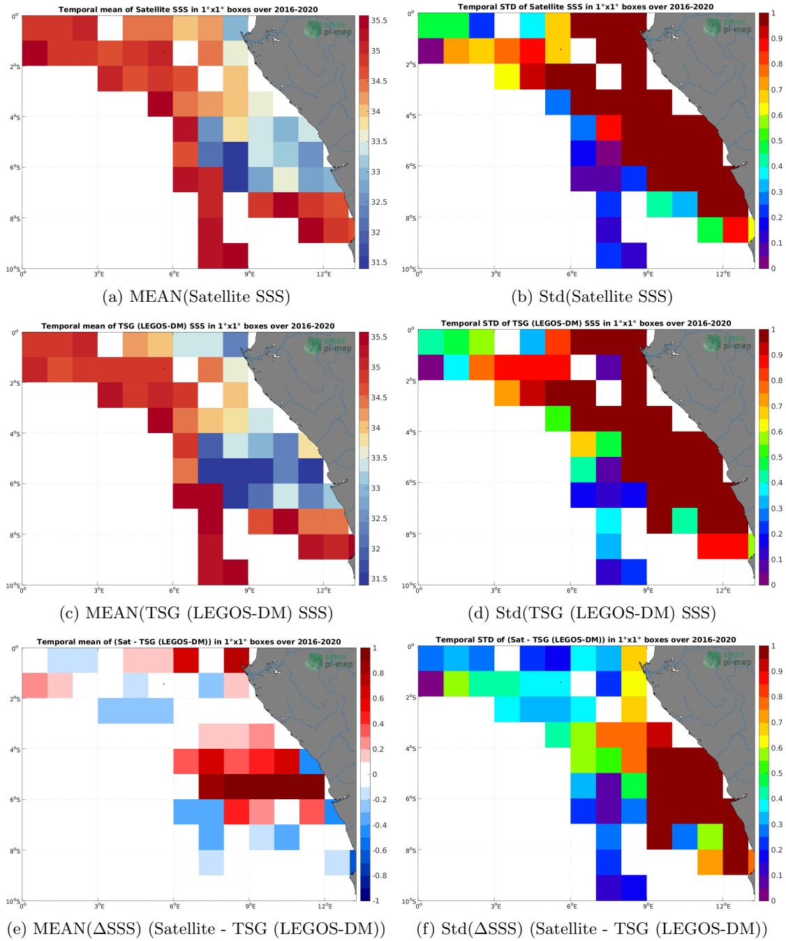
Figure 6: Temporal mean (left) and Std (right) of SSS from SMOS SSS L3 v8 - 18 Days (CATDS-CECOS-LOCEAN) (top), TSG (LEGOS-DM) (middle), and of \Delta SSS (Satellite - TSG (LEGOS-DM)). Only match-up pairs are used to generate these maps.
