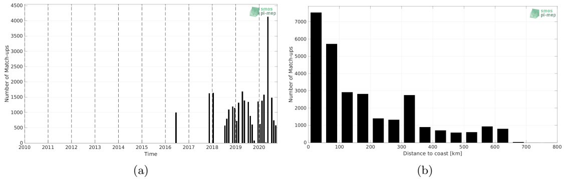
Figure 1: Number of match-ups between TSG (LEGOS-DM) and SMOS SSS L3 v8 - 18 Days (CATDS-CECOS-LOCEAN) SSS as a function of time (a) and as function of the distance to coast (b) over the Congo river plume Pi-MEP region and for the full satellite product period.
