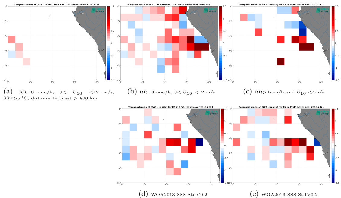
Figure 12: Temporal mean gridded over spatial boxes of size 1^\circ \times 1^\circ of \Delta SSS (SMOS SSS L3 v8 - 18 Days (CATDS-CEC-LOCEAN) - TSG (GOSUD-Research-vessel)) for 5 different subdatasets corresponding to:RR=0 mm/h, 3 < U_{10} < 12 m/s, SST>5°C, distance to coast > 800 km (a), RR=0 mm/h, 3 < U_{10} < 12 m/s (b), RR>1mm/h and U_{10} < 4 m/s (c), WOA2013 SSS Std<0.2 (d), WOA2013 SSS Std>0.2 (e).
