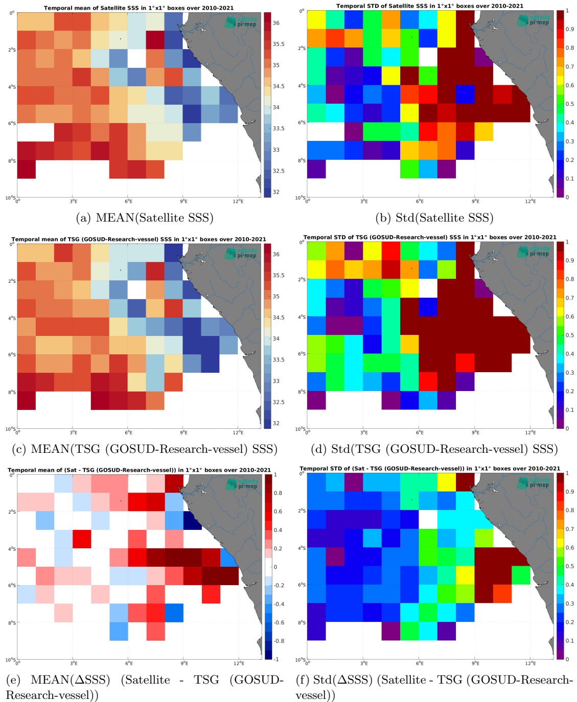
Figure 6: Temporal mean (left) and Std (right) of SSS from SMOS SSS L3 v8 - 18 Days (CATDS-CEC-LOCEAN) (top), TSG (GOSUD-Research-vessel) (middle), and of \Delta SSS (Satellite - TSG (GOSUD-Research-vessel)). Only match-up pairs are used to generate these maps.
