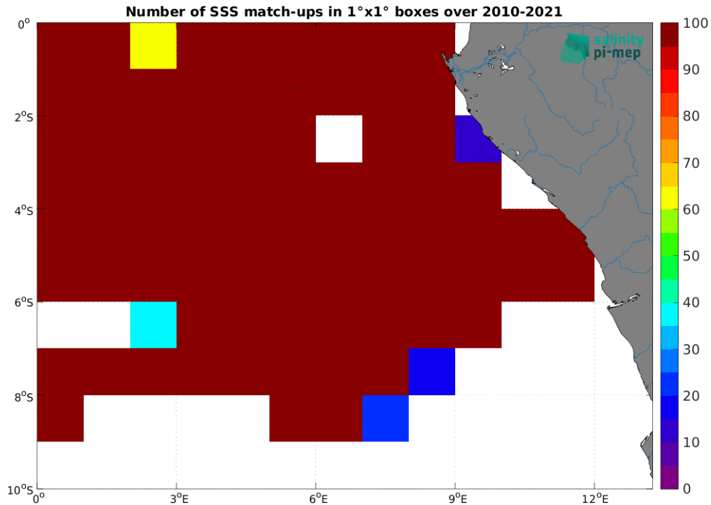
Figure 4: Number of SSS match-ups between TSG (GOSUD-Research-vessel) SSS and the SMOS SSS L3 v8 - 18 Days (CATDS-CEC-LOCEAN) SSS product for the Congo river plume Pi-MEP region over 1^\circ \times 1^\circ boxes and for the full satellite product period.
