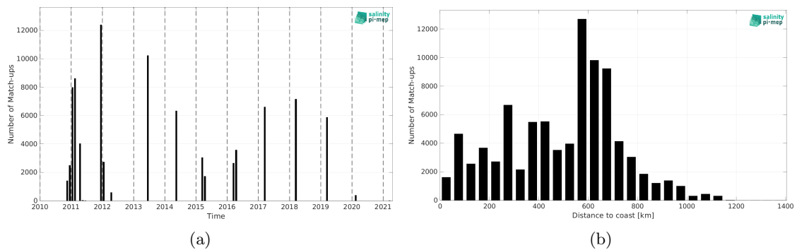
Figure 1: Number of match-ups between TSG (GOSUD-Research-vessel) and SMOS SSS L3 v8 - 18 Days (CATDS-CEC-LOCEAN) SSS as a function of time (a) and as function of the distance to coast (b) over the Congo river plume Pi-MEP region and for the full satellite product period.
