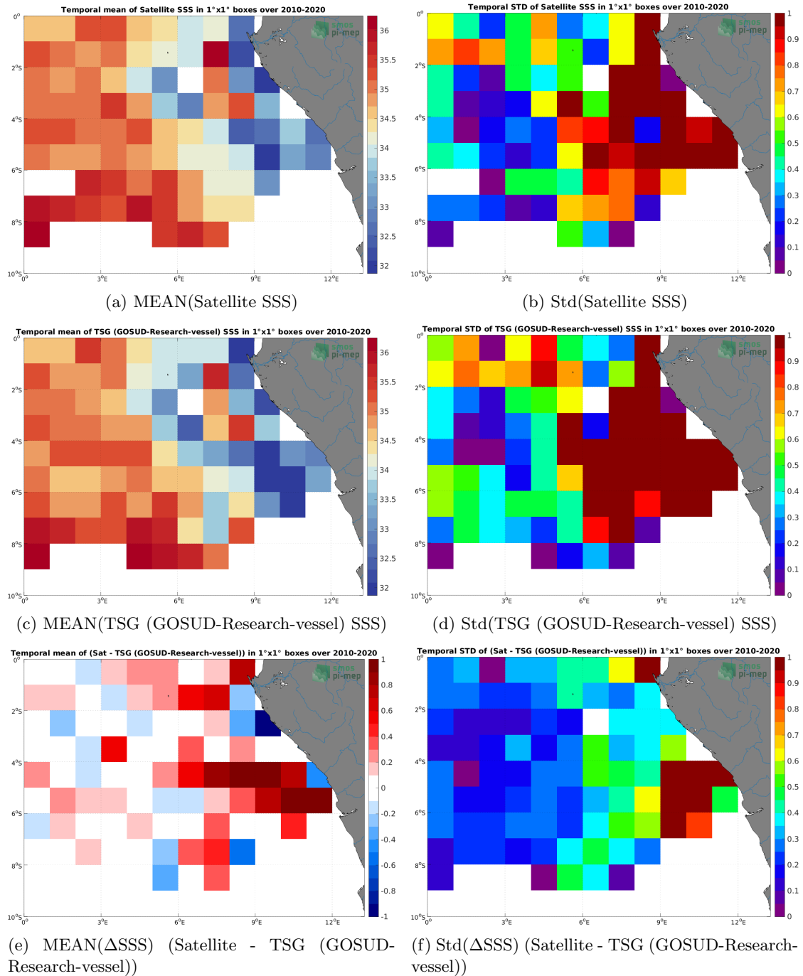
Figure 6: Temporal mean (left) and Std (right) of SSS from SMOS SSS L3 v8 - 18 Days (CATDS-CECOS-LOCEAN) (top), TSG (GOSUD-Research-vessel) (middle), and of \Delta SSS (Satellite - TSG (GOSUD-Research-vessel)). Only match-up pairs are used to generate these maps.
