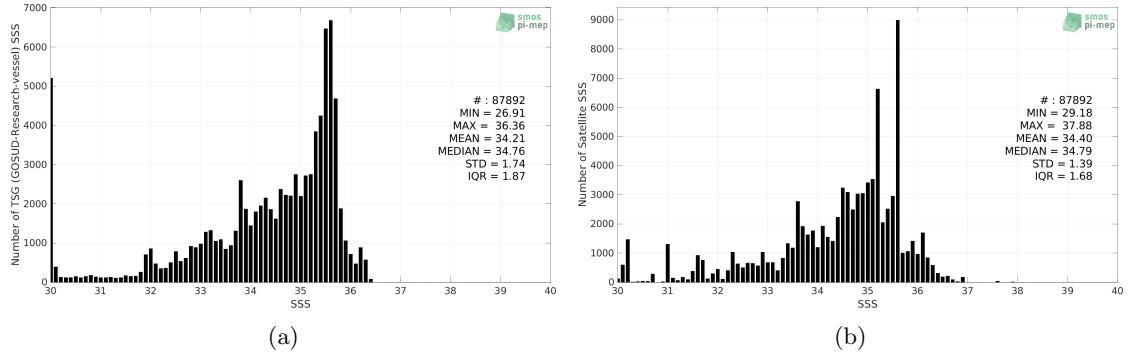
Figure 2: Histograms of SSS from TSG (GOSUD-Research-vessel) (a) and SMOS SSS L3 v8 - 18 Days (CATDS-CECOS-LOCEAN) (b) considering all match-up pairs per bins of 0.1 over the Congo river plume Pi-MEP region and for the full satellite product period.
