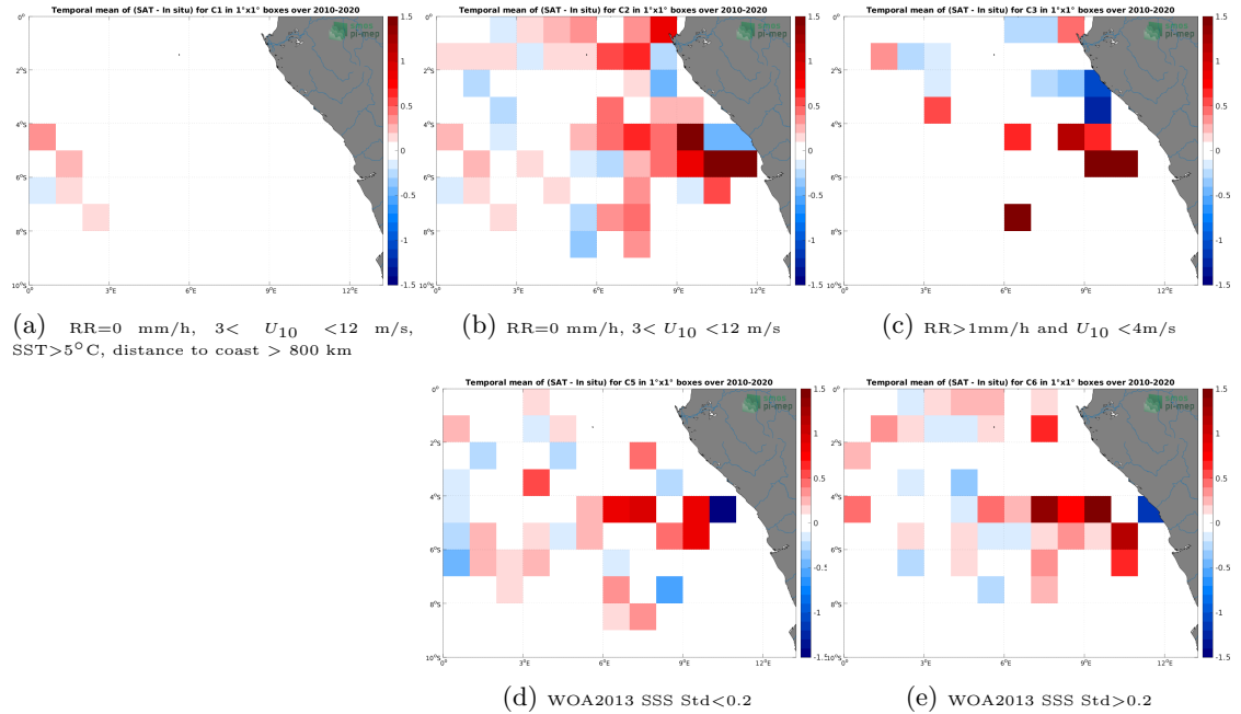
Figure 12: Temporal mean gridded over spatial boxes of size 1^{\circ}\times 1^{\circ} of \Delta SSS (SMOS SSS L3 v8 - 18 Days (CATDS-CECOS-LOCEAN) - TSG (GOSUD-Research-vessel)) for 5 different sub-datasets corresponding to:RR=0 mm/h, 3 < U_{10} < 12 m/s, SST >5^{\circ}\text{C} , distance to coast > 800 km (a), RR=0 mm/h, 3 < U_{10} < 12 m/s (b), RR >1 mm/h and U_{10} < 4 m/s (c), WOA2013 SSS Std <0.2 (d), WOA2013 SSS Std >0.2 (e).
