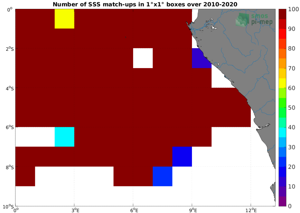
Figure 4: Number of SSS match-ups between TSG (GOSUD-Research-vessel) SSS and the SMOS SSS L3 v8 - 18 Days (CATDS-CECOS-LOCEAN) SSS product for the Congo river plume Pi-MEP region over 1^\circ \times 1^\circ boxes and for the full satellite product period.
