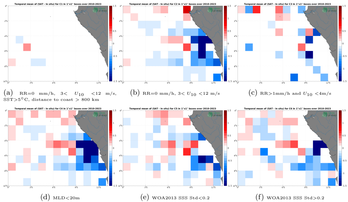
Figure 12: Temporal mean gridded over spatial boxes of size 1^\circ \times 1^\circ of \Delta SSS (SMOS SSS L3 v8 - 18 Days (CATDS-CECOS-LOCEAN) - Argo) for 6 different subdatasets corresponding to:RR=0 mm/h, 3 < U_{10} < 12 m/s, SST >5^\circ C, distance to coast > 800 km (a), RR=0 mm/h, 3 < U_{10} < 12 m/s (b), RR >1 mm/h and U_{10} < 4 m/s (c),MLD <20 m (d),WOA2013 SSS Std <0.2 (e),WOA2013 SSS Std >0.2 (f).
