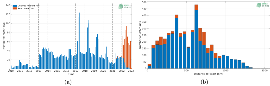
Figure 1: Number of match-ups between Argo and SMOS SSS L3 v8 - 18 Days (CATDS-CECOS-LOCEAN) SSS as a function of time (a) and as function of the distance to coast (b) over the Congo river plume Pi-MEP region and for the full satellite product period.
