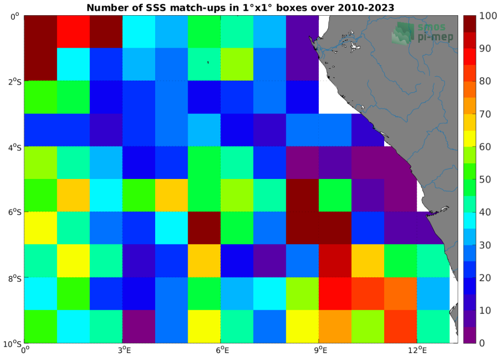
Figure 4: Number of SSS match-ups between Argo SSS and the SMOS SSS L3 v8 - 18 Days (CATDS-CECOS-LOCEAN) SSS product for the Congo river plume Pi-MEP region over 1^\circ \times 1^\circ boxes and for the full satellite product period.
