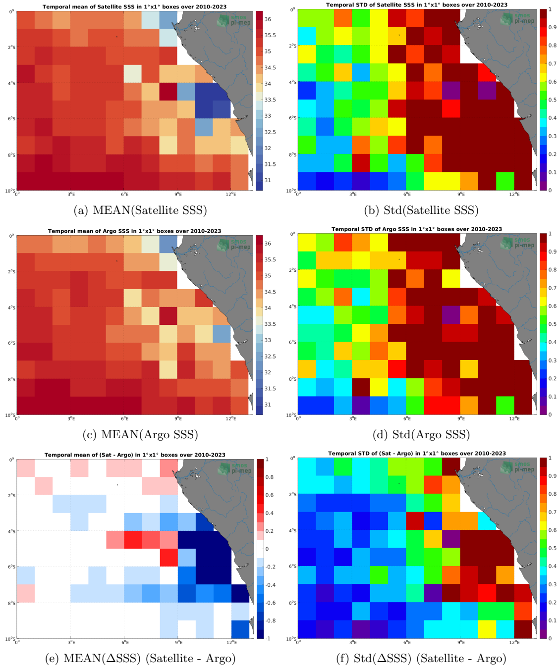
Figure 6: Temporal mean (left) and Std (right) of SSS from SMOS SSS L3 v8 - 18 Days (CATDS-CECOS-LOCEAN) (top), Argo (middle), and of \Delta SSS (Satellite - Argo). Only match-up pairs are used to generate these maps.
