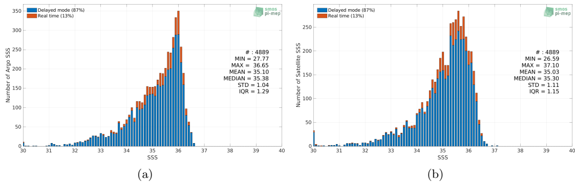
Figure 2: Histograms of SSS from Argo (a) and SMOS SSS L3 v8 - 18 Days (CATDS-CECOS-LOCEAN) (b) considering all match-up pairs per bins of 0.1 over the Congo river plume Pi-MEP region and for the full satellite product period.
