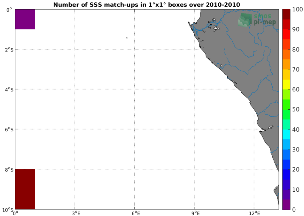
Figure 4: Number of SSS match-ups between TSG (SAMOS) SSS and the SMOS SSS L3 v7 - 9 Days (CATDS-CECOS-LOCEAN) SSS product for the Congo river plume Pi-MEP region over 1^\circ \times 1^\circ boxes and for the full satellite product period.
