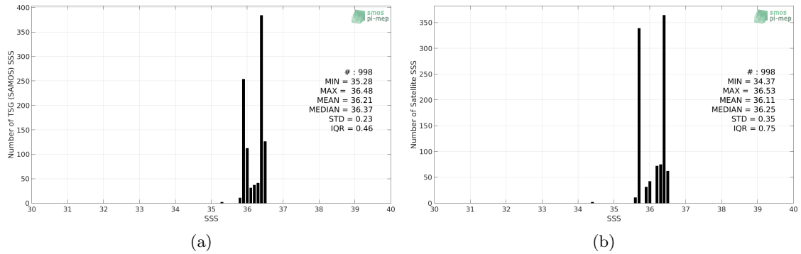
Figure 2: Histograms of SSS from TSG (SAMOS) (a) and SMOS SSS L3 v7 - 9 Days (CATDS-CECOS-LOCEAN) (b) considering all match-up pairs per bins of 0.1 over the Congo river plume Pi-MEP region and for the full satellite product period.
