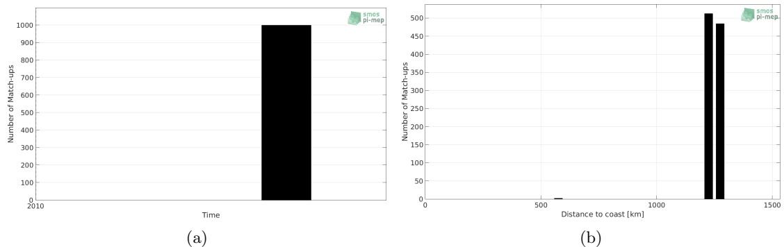
Figure 1: Number of match-ups between TSG (SAMOS) and SMOS SSS L3 v7 - 9 Days (CATDS-CECOS-LOCEAN) SSS as a function of time (a) and as function of the distance to coast (b) over the Congo river plume Pi-MEP region and for the full satellite product period.
