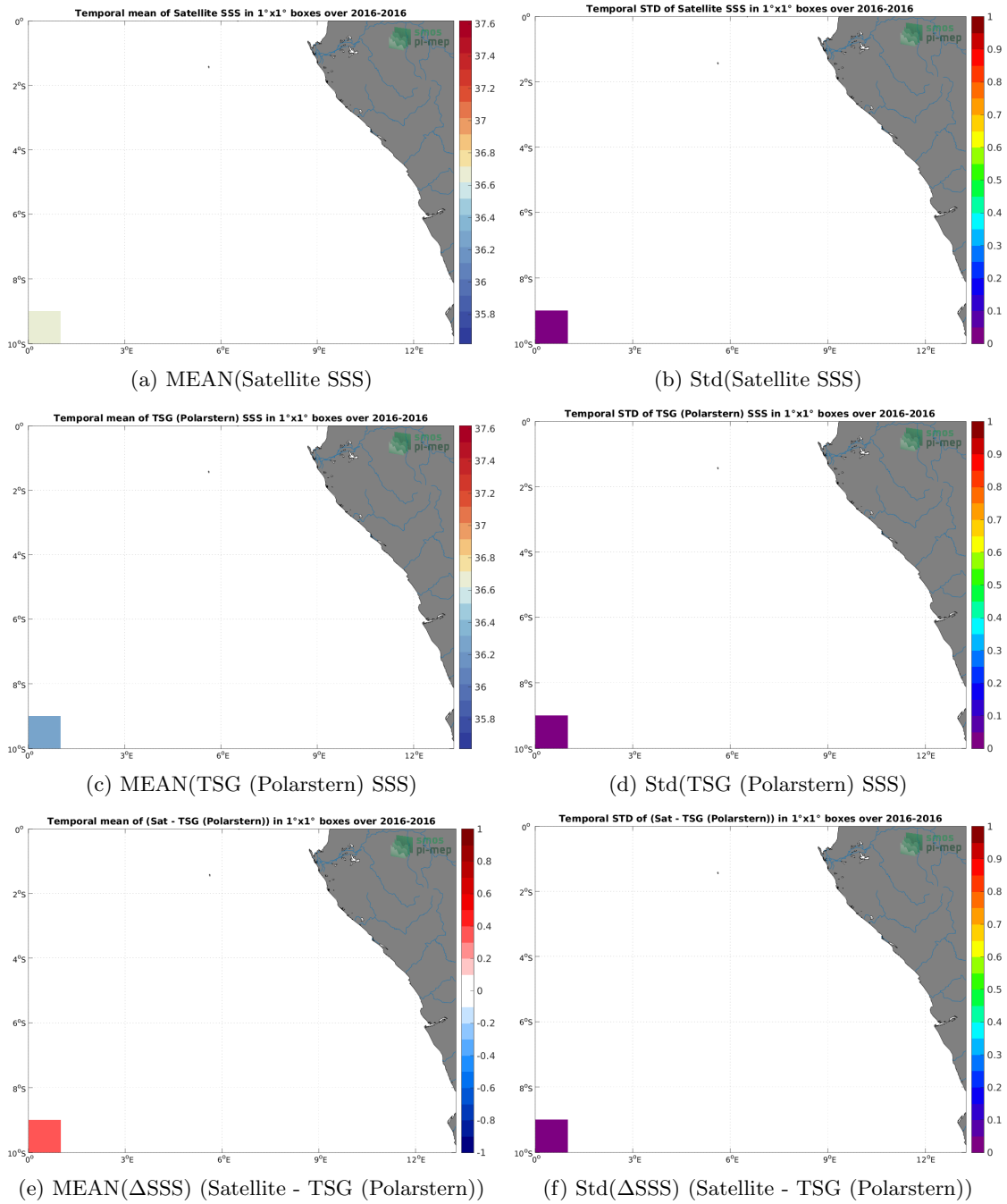
Figure 6: Temporal mean (left) and Std (right) of SSS from SMOS SSS L3 v7 - 9 Days (CATDS-CECOS-LOCEAN) (top), TSG (Polarstern) (middle), and of \Delta SSS (Satellite - TSG (Polarstern)). Only match-up pairs are used to generate these maps.
