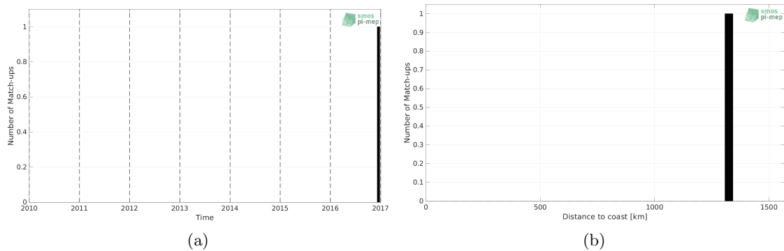
Figure 1: Number of match-ups between TSG (Polarstern) and SMOS SSS L3 v7 - 9 Days (CATDS-CECOS-LOCEAN) SSS as a function of time (a) and as function of the distance to coast (b) over the Congo river plume Pi-MEP region and for the full satellite product period.
