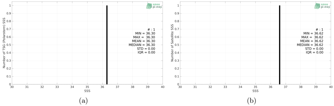
Figure 2: Histograms of SSS from TSG (Polarstern) (a) and SMOS SSS L3 v7 - 9 Days (CATDS-CECOS-LOCEAN) (b) considering all match-up pairs per bins of 0.1 over the Congo river plume Pi-MEP region and for the full satellite product period.
