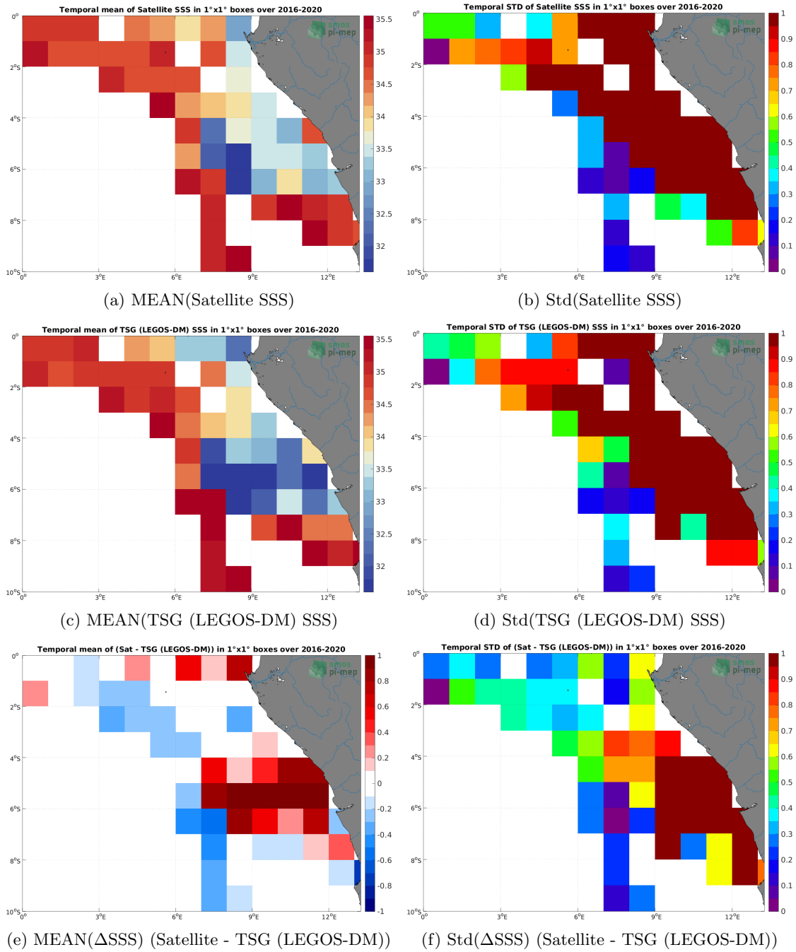
Figure 6: Temporal mean (left) and Std (right) of SSS from SMOS SSS L3 v7 - 9 Days (CATDS-CECOS-LOCEAN) (top), TSG (LEGOS-DM) (middle), and of \Delta SSS (Satellite - TSG (LEGOS-DM)). Only match-up pairs are used to generate these maps.
