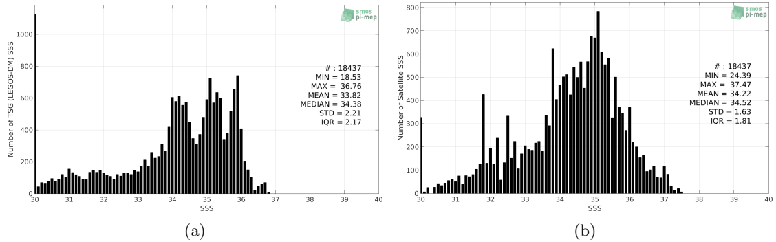
Figure 2: Histograms of SSS from TSG (LEGOS-DM) (a) and SMOS SSS L3 v7 - 9 Days (CATDS-CECOS-LOCEAN) (b) considering all match-up pairs per bins of 0.1 over the Congo river plume Pi-MEP region and for the full satellite product period.
