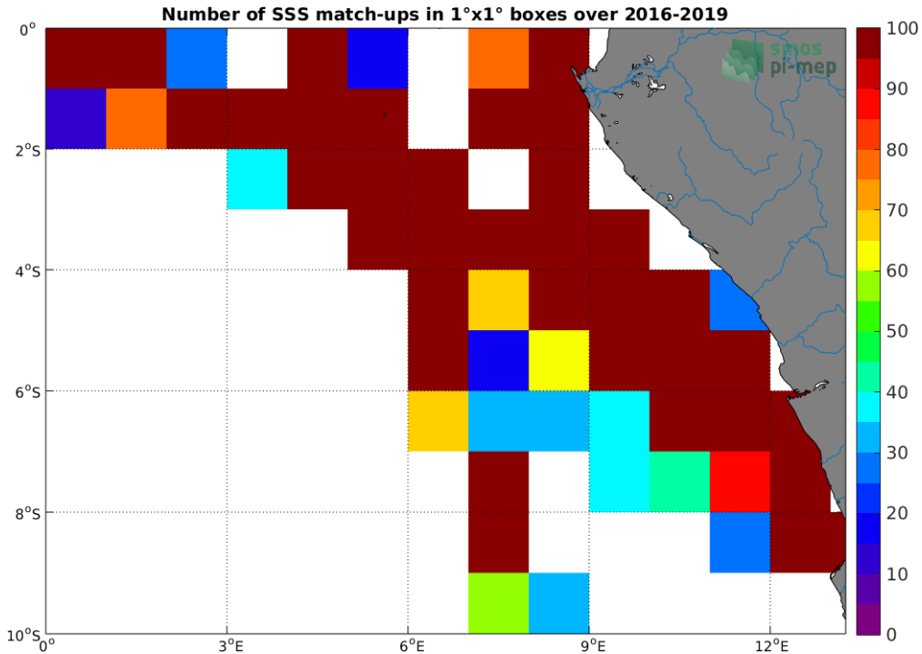
Figure 4: Number of SSS match-ups between TSG (LEGOS-DM) SSS and the SMOS SSS L3 v7 - 9 Days (CATDS-CECOS-LOCEAN) SSS product for the Congo river plume Pi-MEP region over 1^\circ \times 1^\circ boxes and for the full satellite product period.
