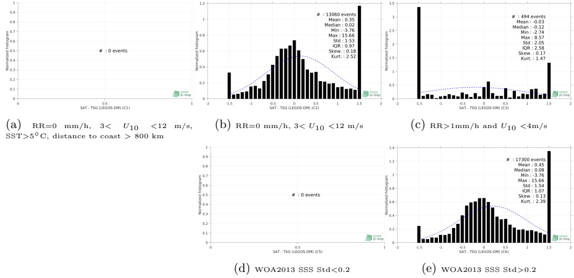
Figure 13: Normalized histogram of \Delta SSS (SMOS SSS L3 v7 - 9 Days (CATDS-CECOS-LOCEAN) - TSG (LEGOS-DM)) for 5 different subdatasets corresponding to: RR=0 mm/h, 3 < U_{10} < 12 m/s, SST > 5°C, distance to coast > 800 km (a), RR=0 mm/h, 3 < U_{10} < 12 m/s (b), RR > 1mm/h and U_{10} < 4 m/s (c), WOA2013 SSS Std < 0.2 (d), WOA2013 SSS Std > 0.2 (e).
