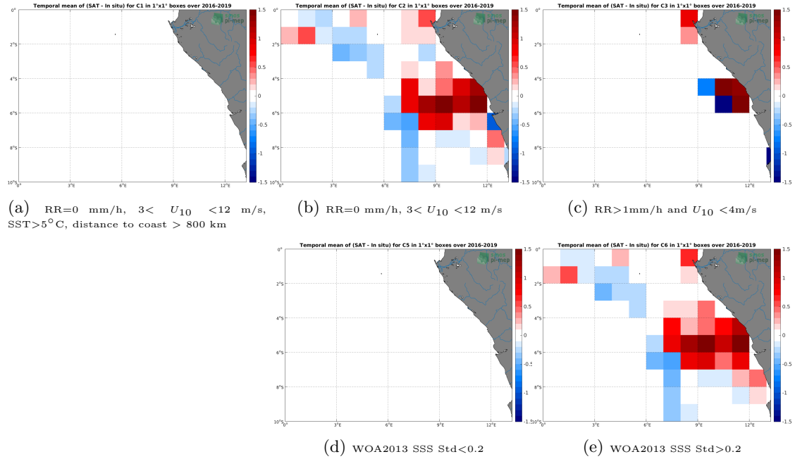
Figure 12: Temporal mean gridded over spatial boxes of size 1^{\circ}\times 1^{\circ} of \Delta\text{SSS} (SMOS SSS L3 v7 - 9 Days (CATDS-CECOS-LOCEAN) - TSG (LEGOS-DM)) for 5 different subdatasets corresponding to:RR=0 mm/h, 3 < U_{10} < 12 m/s, SST >5^{\circ}\text{C} , distance to coast > 800 km (a), RR=0 mm/h, 3 < U_{10} < 12 m/s (b), RR >1 mm/h and U_{10} < 4 m/s (c), WOA2013 SSS Std <0.2 (d), WOA2013 SSS Std >0.2 (e).
