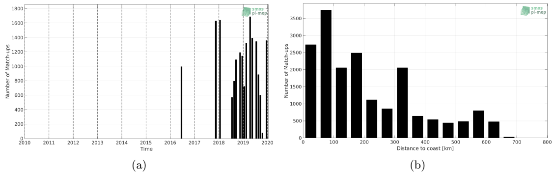
Figure 1: Number of match-ups between TSG (LEGOS-DM) and SMOS SSS L3 v7 - 9 Days (CATDS-CECOS-LOCEAN) SSS as a function of time (a) and as function of the distance to coast (b) over the Congo river plume Pi-MEP region and for the full satellite product period.
