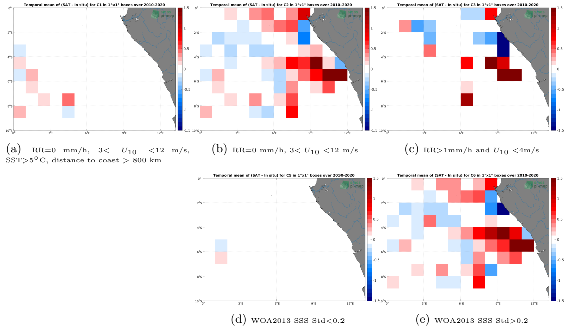
Figure 12: Temporal mean gridded over spatial boxes of size 1^{\circ}\times 1^{\circ} of \Delta SSS (SMOS SSS L3 v7 - 9 Days (CATDS-CECOS-LOCEAN) - TSG (GOSUD-Research-vessel)) for 5 different subdatasets corresponding to:RR=0 mm/h, 3 < U_{10} < 12 m/s, SST >5^{\circ}\text{C} , distance to coast > 800 km (a), RR=0 mm/h, 3 < U_{10} < 12 m/s (b), RR >1 mm/h and U_{10} < 4 m/s (c), WOA2013 SSS Std <0.2 (d), WOA2013 SSS Std >0.2 (e).
