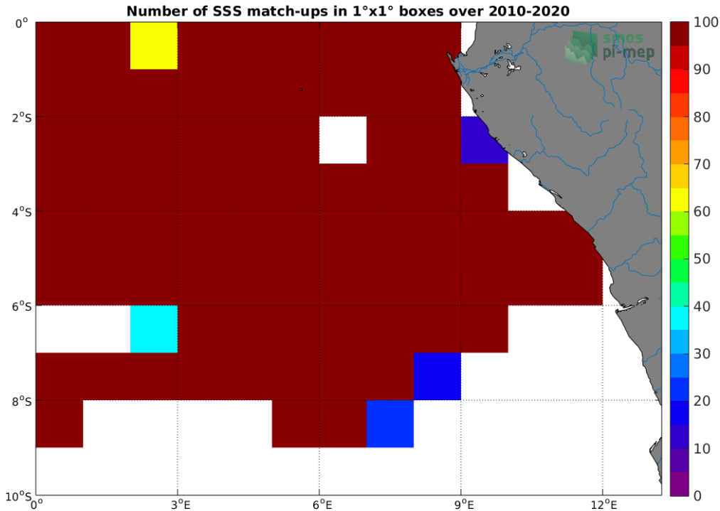
Figure 4: Number of SSS match-ups between TSG (GOSUD-Research-vessel) SSS and the SMOS SSS L3 v7 - 9 Days (CATDS-CECOS-LOCEAN) SSS product for the Congo river plume Pi-MEP region over 1^\circ \times 1^\circ boxes and for the full satellite product period.
