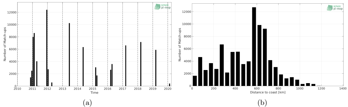
Figure 1: Number of match-ups between TSG (GOSUD-Research-vessel) and SMOS SSS L3 v7 - 9 Days (CATDS-CECOS-LOCEAN) SSS as a function of time (a) and as function of the distance to coast (b) over the Congo river plume Pi-MEP region and for the full satellite product period.
