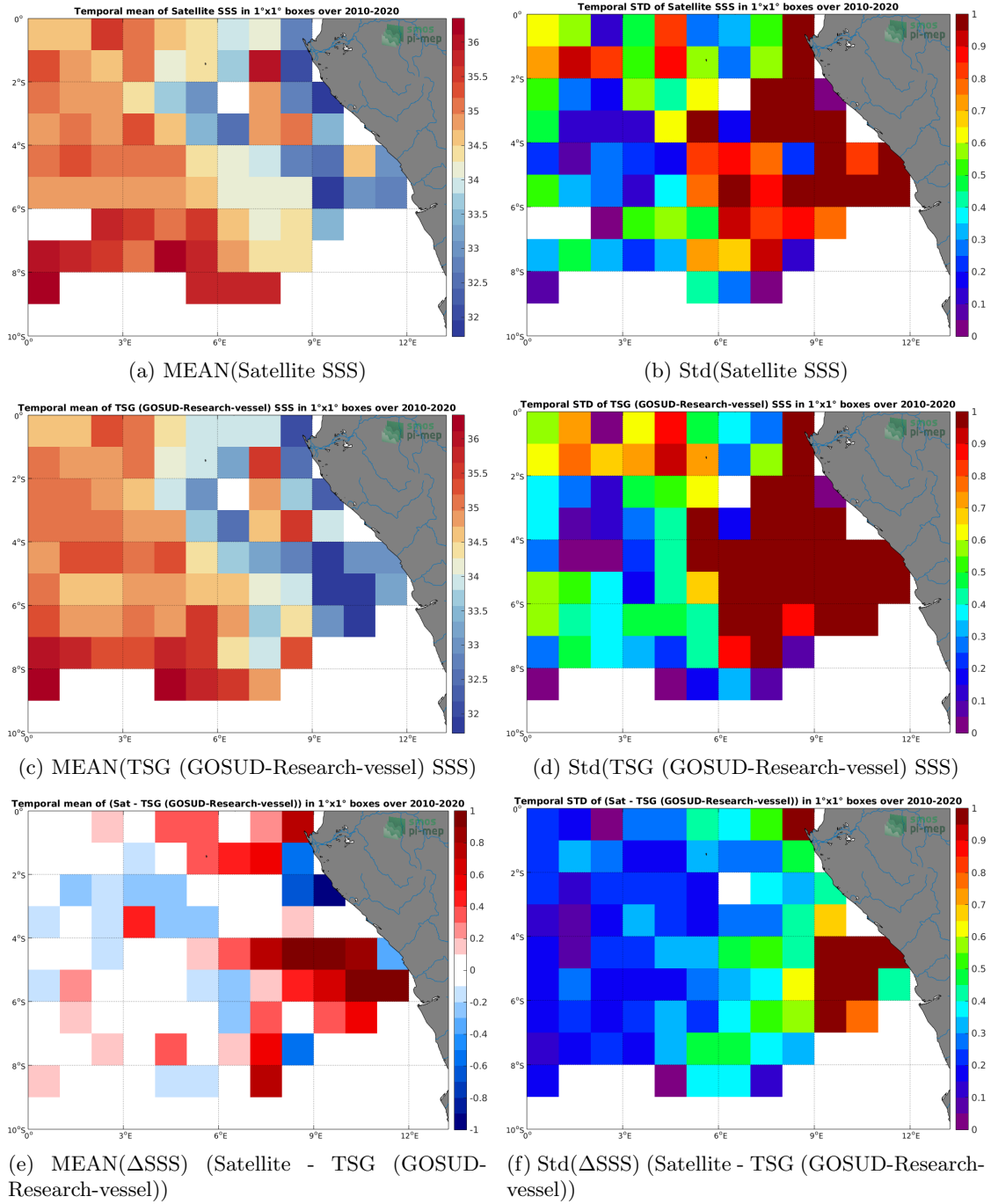
Figure 6: Temporal mean (left) and Std (right) of SSS from SMOS SSS L3 v7 - 9 Days (CATDS-CECOS-LOCEAN) (top), TSG (GOSUD-Research-vessel) (middle), and of \Delta SSS (Satellite - TSG (GOSUD-Research-vessel)). Only match-up pairs are used to generate these maps.
