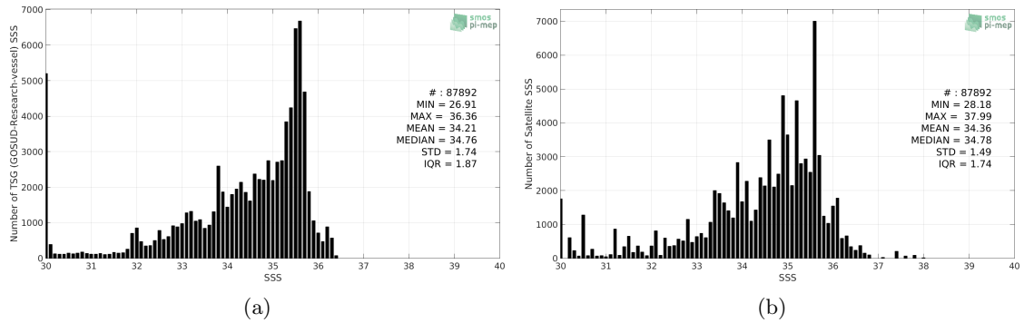
Figure 2: Histograms of SSS from TSG (GOSUD-Research-vessel) (a) and SMOS SSS L3 v7 - 9 Days (CATDS-CECOS-LOCEAN) (b) considering all match-up pairs per bins of 0.1 over the Congo river plume Pi-MEP region and for the full satellite product period.
