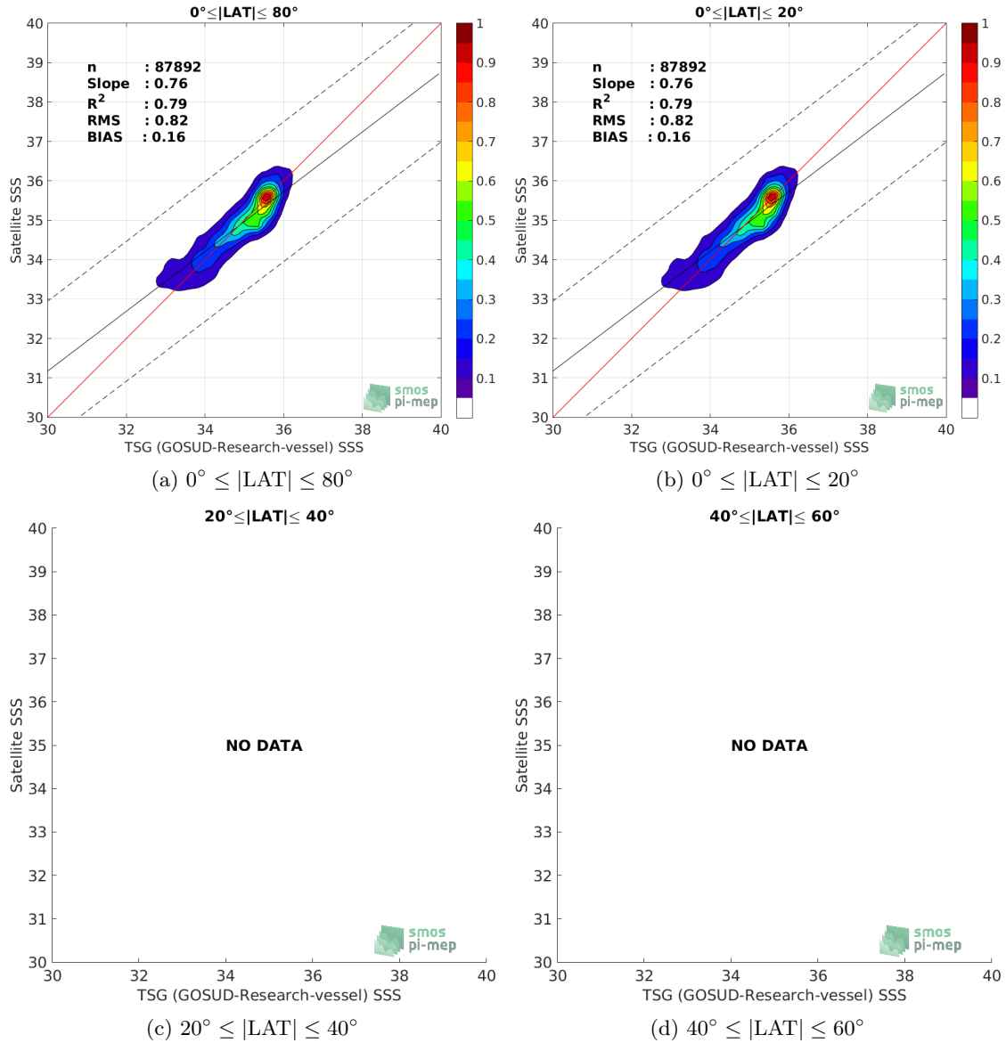
Figure 9: Contour maps of the concentration of SMOS SSS L3 v7 - 9 Days (CATDS-CECOS-LOCEAN) SSS ( y -axis) versus TSG (GOSUD-Research-vessel) SSS ( x -axis) at match-up pairs for different latitude bands. For each plot, the red line shows x=y . The black thin and dashed lines indicate a linear fit through the data cloud and the \pm 95\% confidence levels, respectively. The number match-up pairs n , the slope and R^2 coefficient of the linear fit, the root mean square (RMS) and the mean bias between satellite and in situ data are indicated for each latitude band in each plots.
