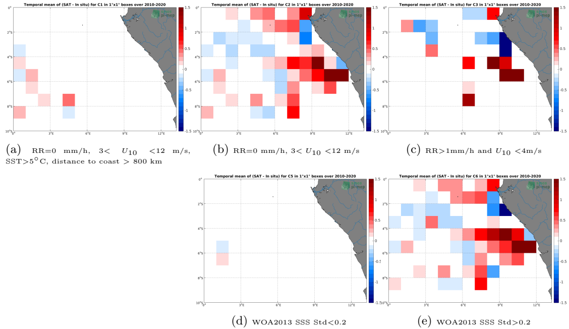
Figure 12: Temporal mean gridded over spatial boxes of size 1^\circ \times 1^\circ of \Delta SSS (SMOS SSS L3 v7 - 9 Days (CATDS-CECOS-LOCEAN) - TSG (GOSUD-Research-vessel)) for 5 different subdatasets corresponding to: RR=0 mm/h, 3 < U_{10} < 12 m/s, SST > 5^\circ\text{C} , distance to coast > 800 km (a), RR=0 mm/h, 3 < U_{10} < 12 m/s (b), RR > 1 mm/h and U_{10} < 4 m/s (c), WOA2013 SSS Std < 0.2 (d), WOA2013 SSS Std > 0.2 (e).
