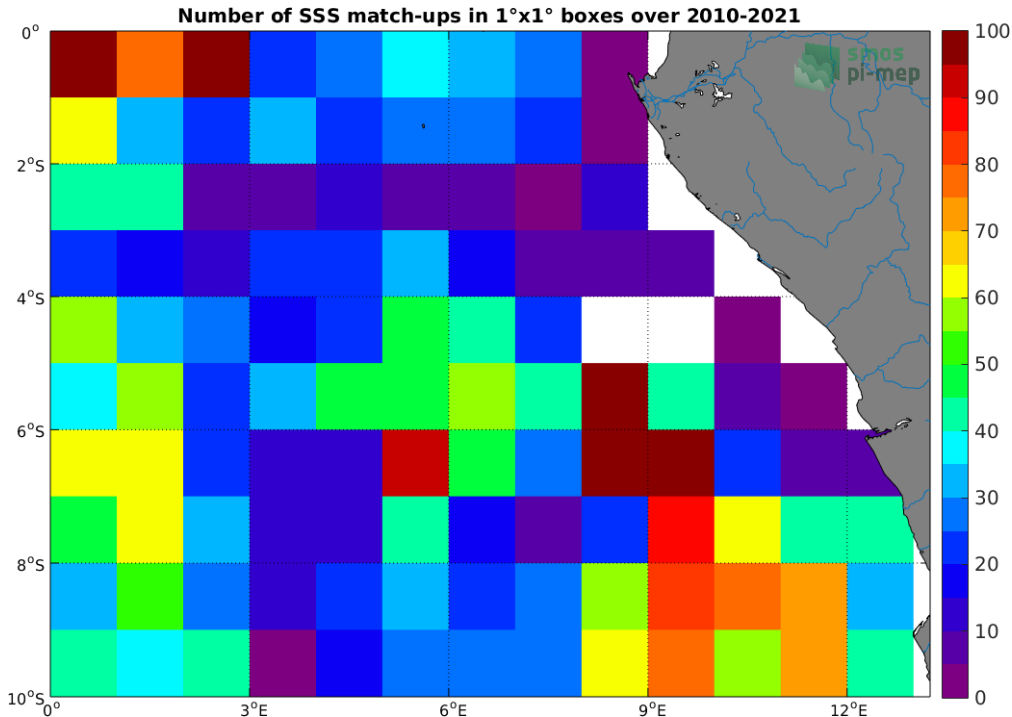
Figure 4: Number of SSS match-ups between Argo SSS and the SMOS SSS L3 v7 - 9 Days (CATDS-CECOS-LOCEAN) SSS product for the Congo river plume Pi-MEP region over 1^\circ \times 1^\circ boxes and for the full satellite product period.
