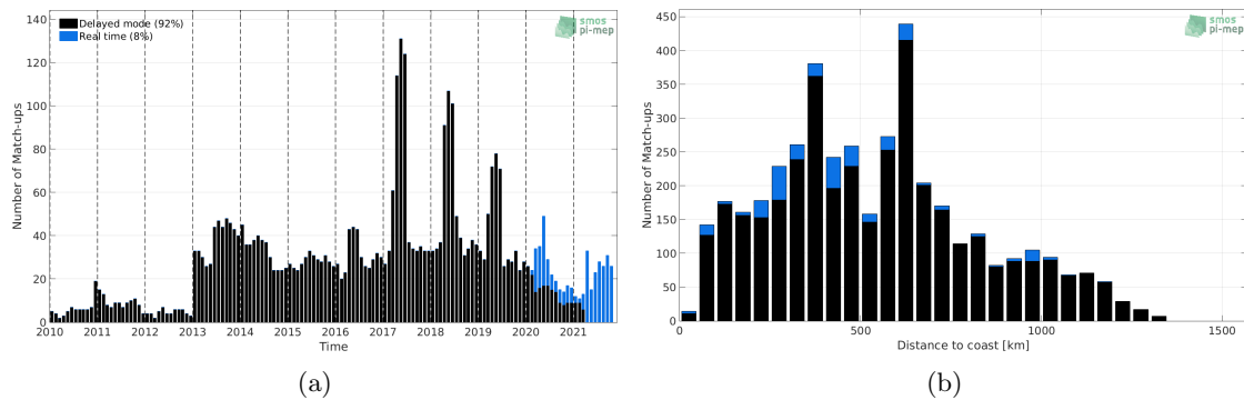
Figure 1: Number of match-ups between Argo and SMOS SSS L3 v7 - 9 Days (CATDS-CECOS-LOCEAN) SSS as a function of time (a) and as function of the distance to coast (b) over the Congo river plume Pi-MEP region and for the full satellite product period.
