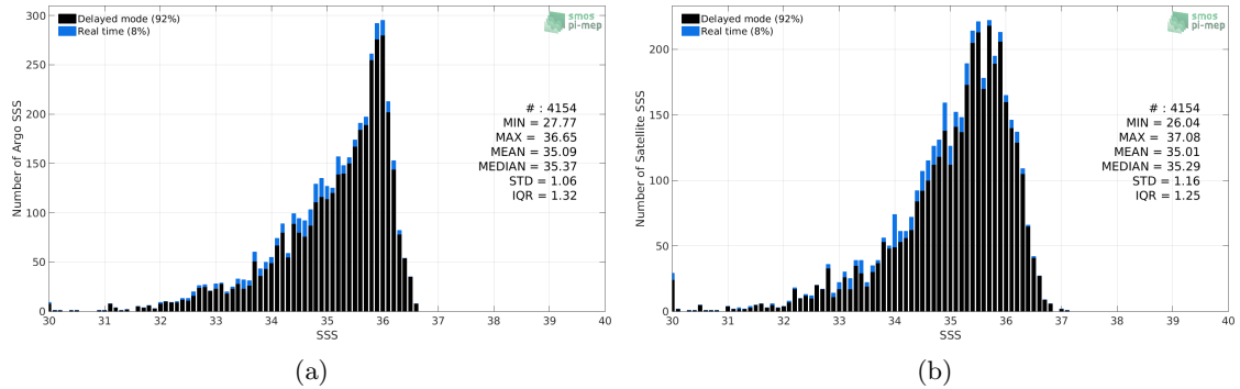
Figure 2: Histograms of SSS from Argo (a) and SMOS SSS L3 v7 - 9 Days (CATDS-CECOS-LOCEAN) (b) considering all match-up pairs per bins of 0.1 over the Congo river plume Pi-MEP region and for the full satellite product period.
