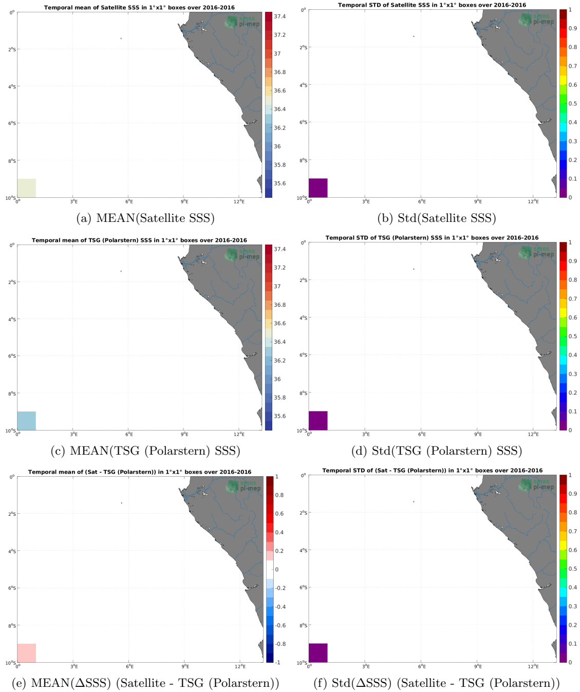
Figure 6: Temporal mean (left) and Std (right) of SSS from SMOS SSS L3 v7 - 18 Days (CATDS-CECOS-LOCEAN) (top), TSG (Polarstern) (middle), and of \Delta SSS (Satellite - TSG (Polarstern)). Only match-up pairs are used to generate these maps.
