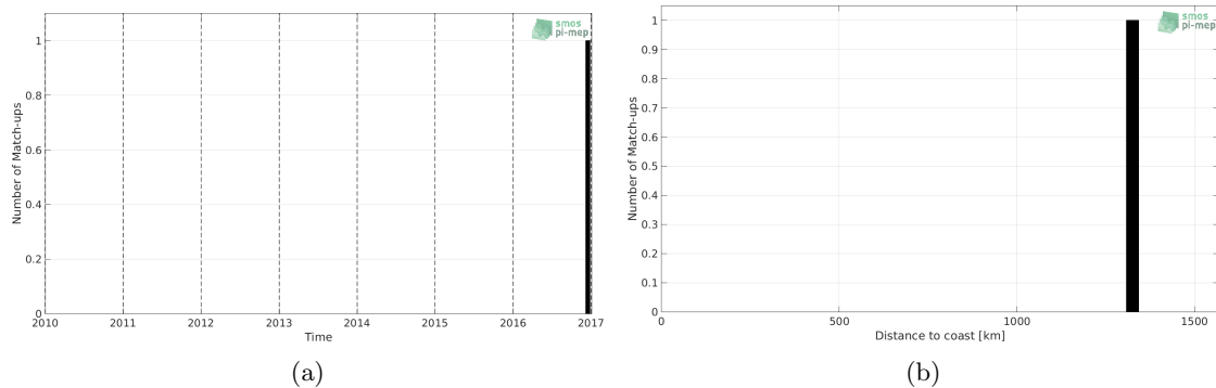
Figure 1: Number of match-ups between TSG (Polarstern) and SMOS SSS L3 v7 - 18 Days (CATDS-CECOS-LOCEAN) SSS as a function of time (a) and as function of the distance to coast (b) over the Congo river plume Pi-MEP region and for the full satellite product period.
