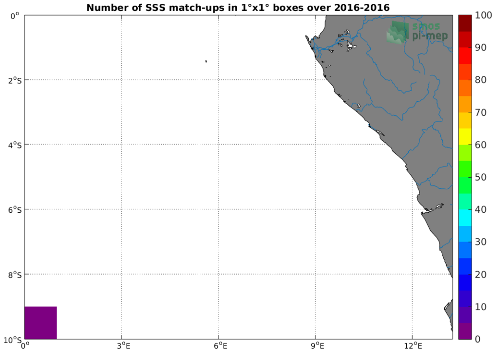
Figure 4: Number of SSS match-ups between TSG (Polarstern) SSS and the SMOS SSS L3 v7 - 18 Days (CATDS-CECOS-LOCEAN) SSS product for the Congo river plume Pi-MEP region over 1^\circ \times 1^\circ boxes and for the full satellite product period.
