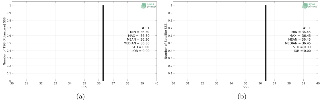
Figure 2: Histograms of SSS from TSG (Polarstern) (a) and SMOS SSS L3 v7 - 18 Days (CATDS-CECOS-LOCEAN) (b) considering all match-up pairs per bins of 0.1 over the Congo river plume Pi-MEP region and for the full satellite product period.
