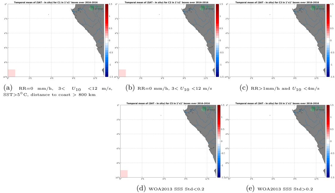
Figure 12: Temporal mean gridded over spatial boxes of size 1^{\circ}\times 1^{\circ} of \Delta\text{SSS} (SMOS SSS L3 v7 - 18 Days (CATDS-CECOS-LOCEAN) - TSG (Polarstern)) for 5 different subdatasets corresponding to:RR=0 mm/h, 3 < U_{10} < 12 m/s, SST >5^{\circ}\text{C} , distance to coast > 800 km (a), RR=0 mm/h, 3 < U_{10} < 12 m/s (b), RR >1 mm/h and U_{10} < 4 m/s (c), WOA2013 SSS Std <0.2 (d), WOA2013 SSS Std >0.2 (e).
