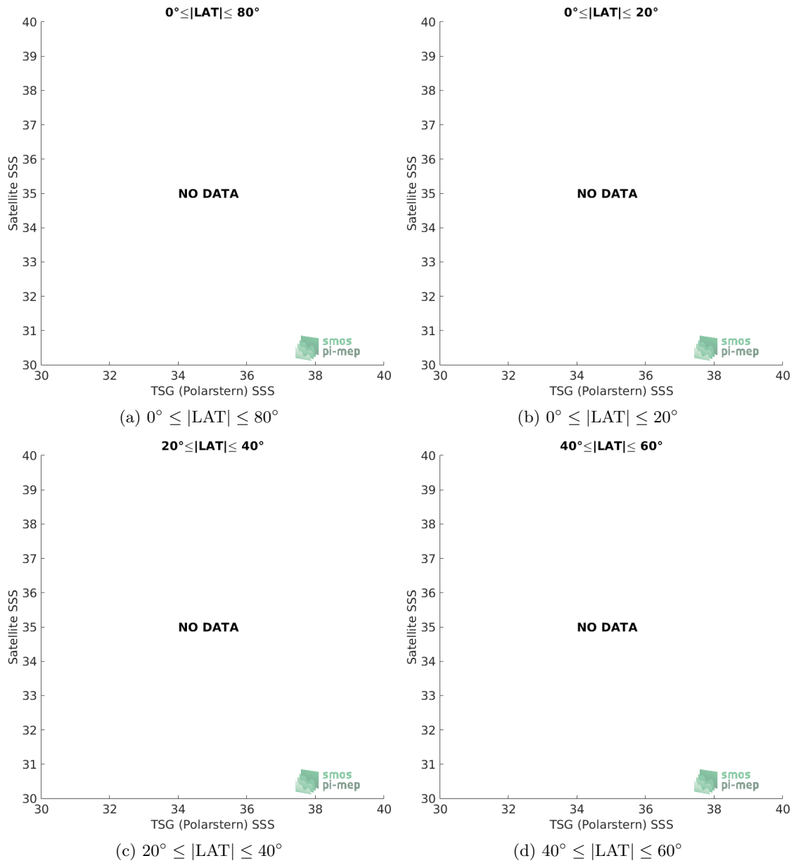
Figure 9: Contour maps of the concentration of SMOS SSS L3 v7 - 18 Days (CATDS-CECOS-LOCEAN) SSS ( y -axis) versus TSG (Polarstern) SSS ( x -axis) at match-up pairs for different latitude bands. For each plot, the red line shows x=y . The black thin and dashed lines indicate a linear fit through the data cloud and the \pm 95\% confidence levels, respectively. The number match-up pairs n , the slope and R^2 coefficient of the linear fit, the root mean square (RMS) and the mean bias between satellite and in situ data are indicated for each latitude band in each plots.
