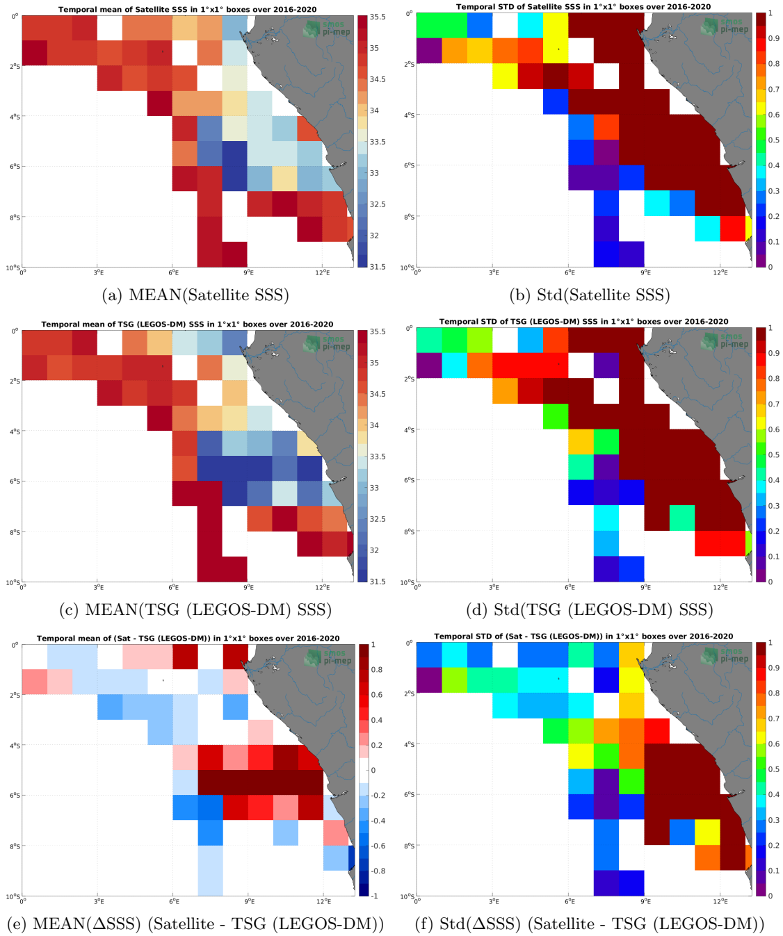
Figure 6: Temporal mean (left) and Std (right) of SSS from SMOS SSS L3 v7 - 18 Days (CATDS-CECOS-LOCEAN) (top), TSG (LEGOS-DM) (middle), and of \Delta SSS (Satellite - TSG (LEGOS-DM)). Only match-up pairs are used to generate these maps.
