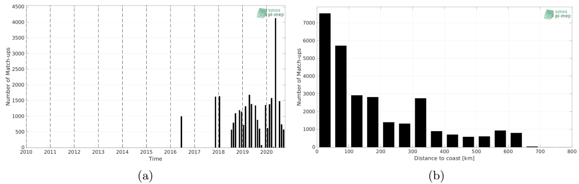
Figure 1: Number of match-ups between TSG (LEGOS-DM) and SMOS SSS L3 v7 - 18 Days (CATDS-CECOS-LOCEAN) SSS as a function of time (a) and as function of the distance to coast (b) over the Congo river plume Pi-MEP region and for the full satellite product period.
