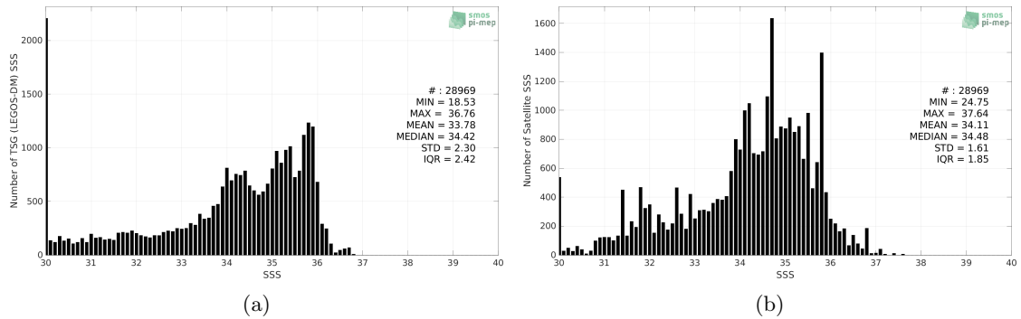
Figure 2: Histograms of SSS from TSG (LEGOS-DM) (a) and SMOS SSS L3 v7 - 18 Days (CATDS-CECOS-LOCEAN) (b) considering all match-up pairs per bins of 0.1 over the Congo river plume Pi-MEP region and for the full satellite product period.
