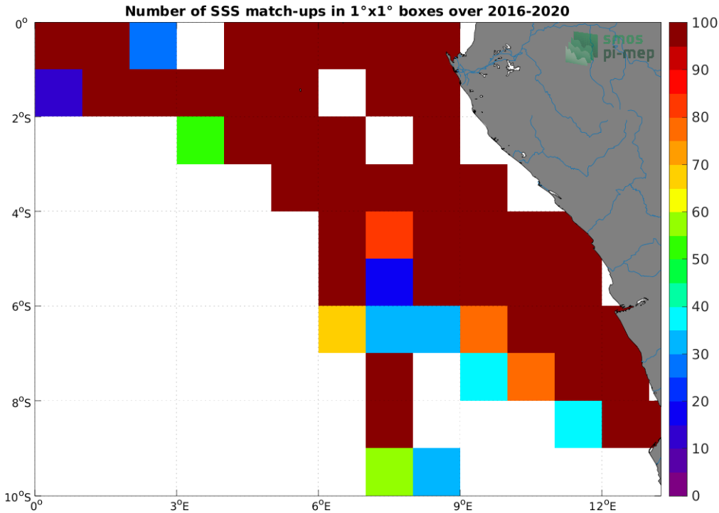
Figure 4: Number of SSS match-ups between TSG (LEGOS-DM) SSS and the SMOS SSS L3 v7 - 18 Days (CATDS-CECOS-LOCEAN) SSS product for the Congo river plume Pi-MEP region over 1^\circ \times 1^\circ boxes and for the full satellite product period.
