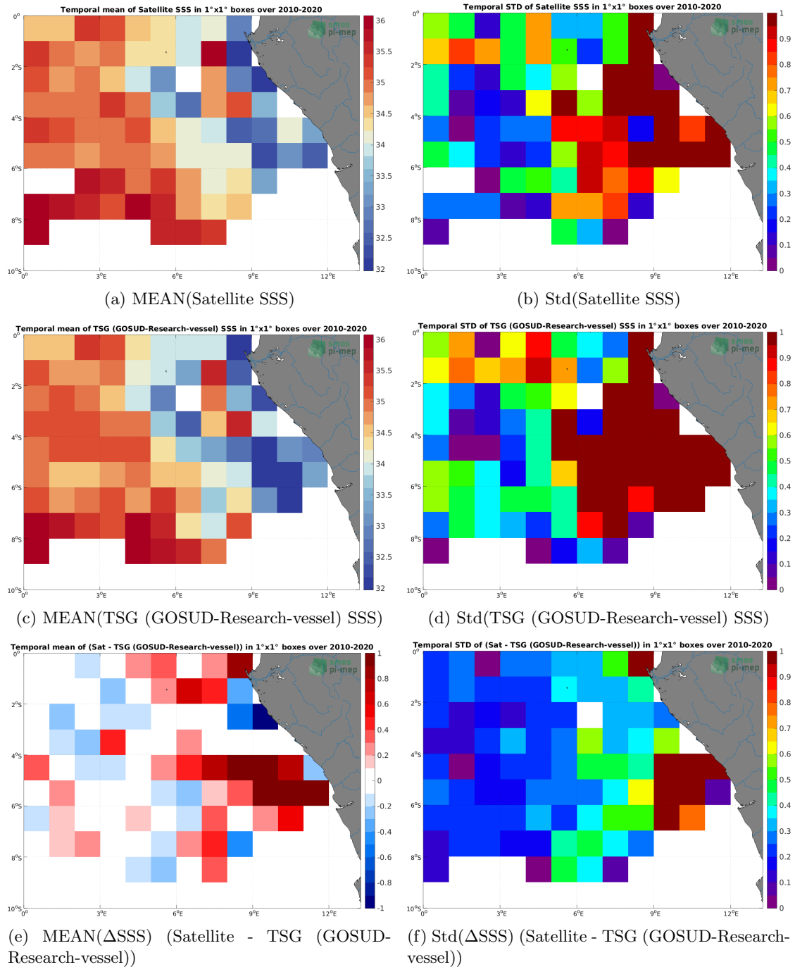
Figure 6: Temporal mean (left) and Std (right) of SSS from SMOS SSS L3 v7 - 18 Days (CATDS-CECOS-LOCEAN) (top), TSG (GOSUD-Research-vessel) (middle), and of \Delta SSS (Satellite - TSG (GOSUD-Research-vessel)). Only match-up pairs are used to generate these maps.
