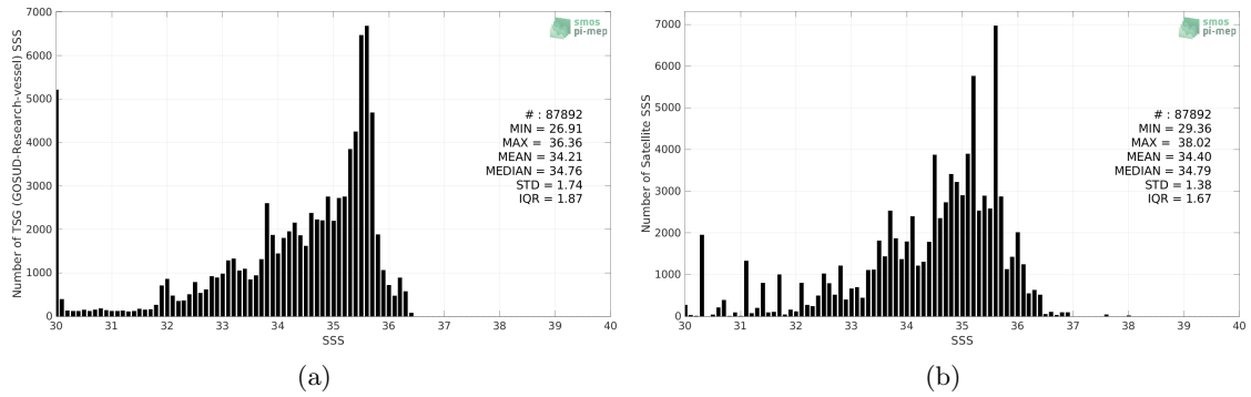
Figure 2: Histograms of SSS from TSG (GOSUD-Research-vessel) (a) and SMOS SSS L3 v7 - 18 Days (CATDS-CECOS-LOCEAN) (b) considering all match-up pairs per bins of 0.1 over the Congo river plume Pi-MEP region and for the full satellite product period.
