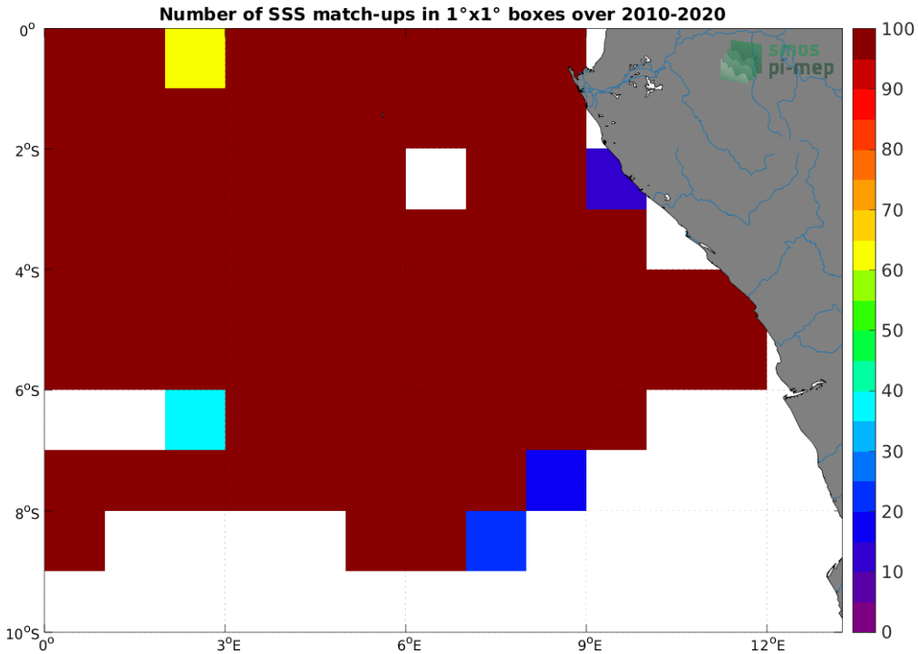
Figure 4: Number of SSS match-ups between TSG (GOSUD-Research-vessel) SSS and the SMOS SSS L3 v7 - 18 Days (CATDS-CECOS-LOCEAN) SSS product for the Congo river plume Pi-MEP region over 1^\circ \times 1^\circ boxes and for the full satellite product period.
