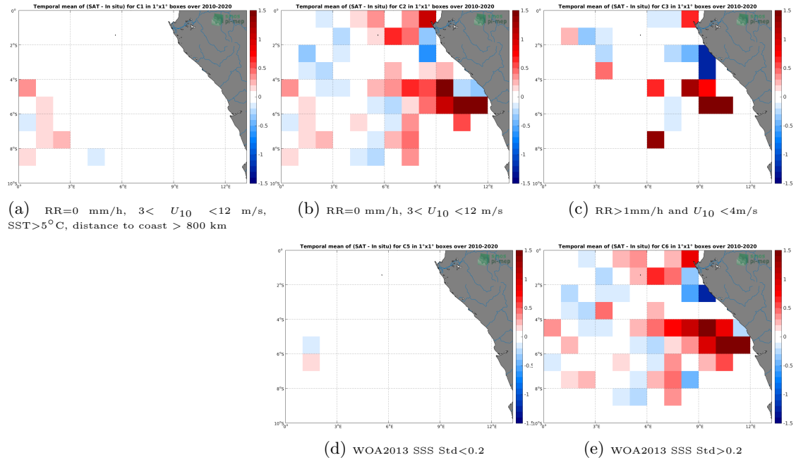
Figure 12: Temporal mean gridded over spatial boxes of size 1^\circ \times 1^\circ of \Delta SSS (SMOS SSS L3 v7 - 18 Days (CATDS-CECOS-LOCEAN) - TSG (GOSUD-Research-vessel)) for 5 different sub-datasets corresponding to:RR=0 mm/h, 3 < U_{10} < 12 m/s, SST >5^\circ\text{C} , distance to coast > 800 km (a), RR=0 mm/h, 3 < U_{10} < 12 m/s (b), RR >1 mm/h and U_{10} < 4 m/s (c), WOA2013 SSS Std <0.2 (d), WOA2013 SSS Std >0.2 (e).
