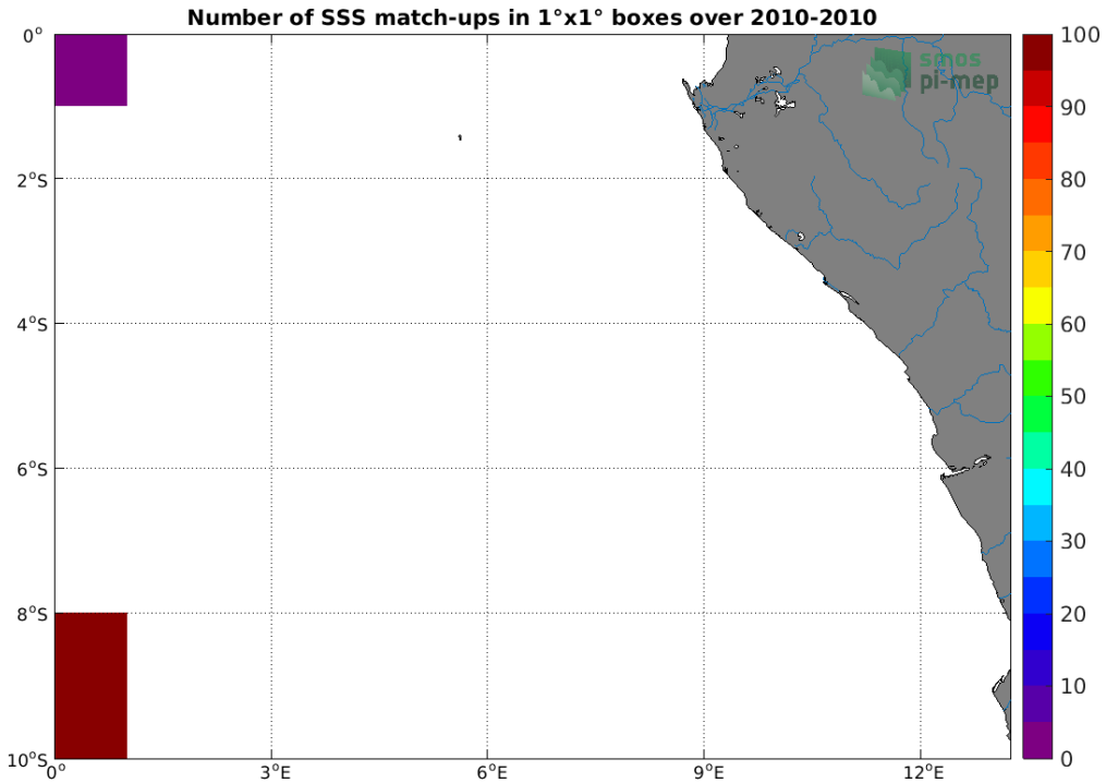
Figure 4: Number of SSS match-ups between TSG (SAMOS) SSS and the SMOS SSS L3 v5 - 9 Days (CATDS-CECOS-LOCEAN) SSS product for the Congo river plume Pi-MEP region over 1°x1° boxes and for the full satellite product period.
