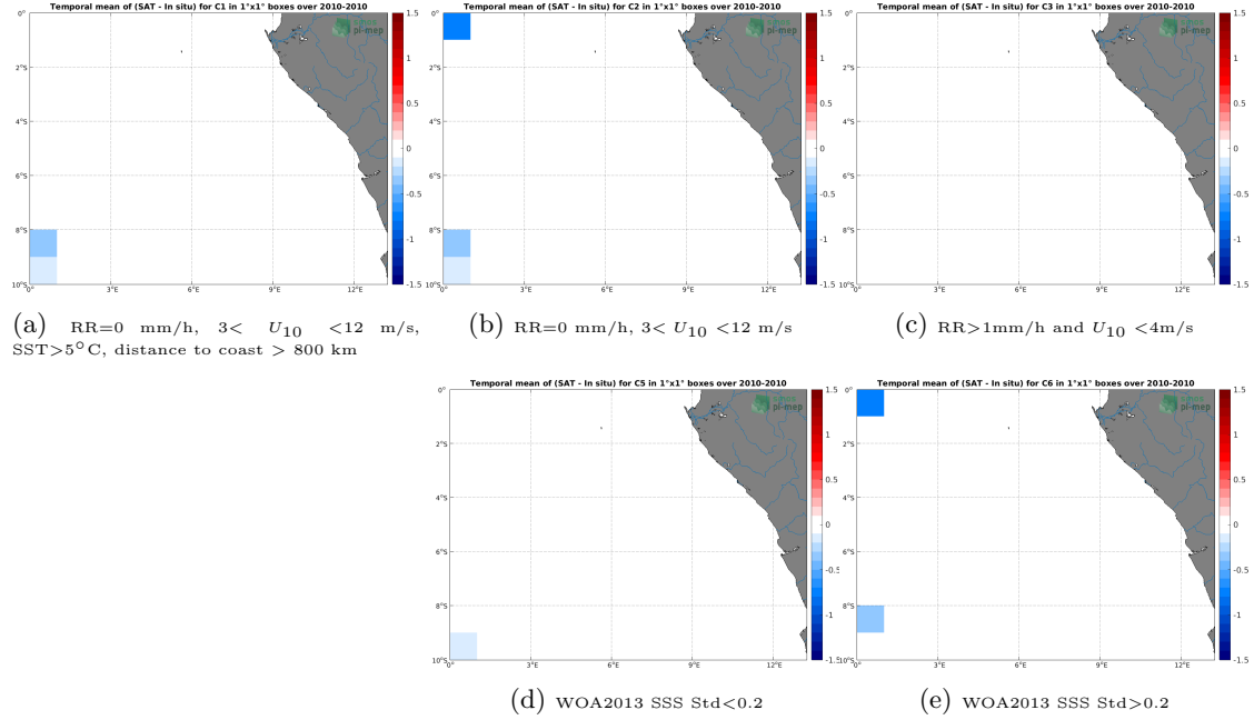
Figure 12: Temporal mean gridded over spatial boxes of size 1^{\circ}\times 1^{\circ} of \Delta\text{SSS} (SMOS SSS L3 v5 - 9 Days (CATDS-CECOS-LOCEAN) - TSG (SAMOS)) for 5 different subdatasets corresponding to:RR=0 mm/h, 3 < U_{10} < 12 m/s, SST >5^{\circ}\text{C} , distance to coast > 800 km (a), RR=0 mm/h, 3 < U_{10} < 12 m/s (b), RR >1 mm/h and U_{10} < 4 m/s (c), WOA2013 SSS Std <0.2 (d), WOA2013 SSS Std >0.2 (e).
