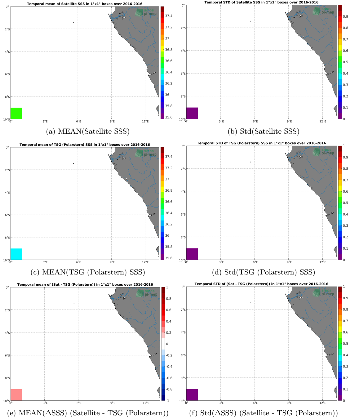
Figure 6: Temporal mean (left) and Std (right) of SSS from SMOS SSS L3 v5 - 9 Days (CATDS-CECOS-LOCEAN) (top), TSG (Polarstern) (middle), and of \Delta SSS (Satellite - TSG (Polarstern)). Only match-up pairs are used to generate these maps.
