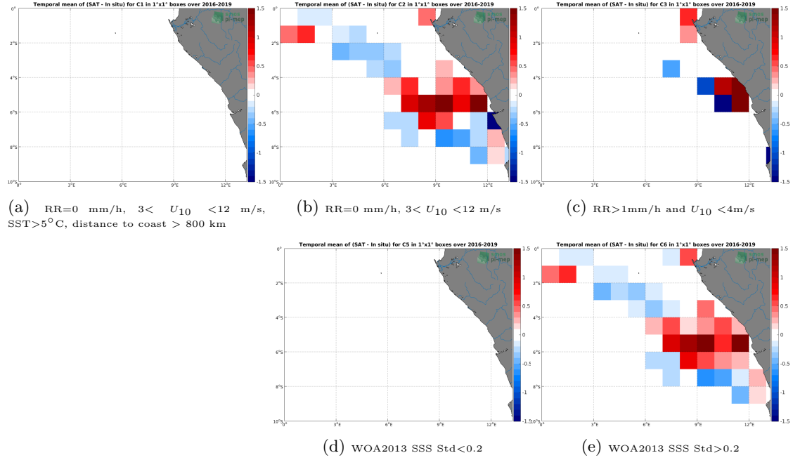
Figure 12: Temporal mean gridded over spatial boxes of size 1^{\circ} \times 1^{\circ} of \Delta\text{SSS} (SMOS SSS L3 v5 - 9 Days (CATDS-CECOS-LOCEAN) - TSG (LEGOS-DM)) for 5 different subdatasets corresponding to: RR=0 mm/h, 3 < U_{10} < 12 m/s, SST >5^{\circ}\text{C} , distance to coast > 800 km (a), RR=0 mm/h, 3 < U_{10} < 12 m/s (b), RR >1 mm/h and U_{10} < 4 m/s (c), WOA2013 SSS Std <0.2 (d), WOA2013 SSS Std >0.2 (e).
