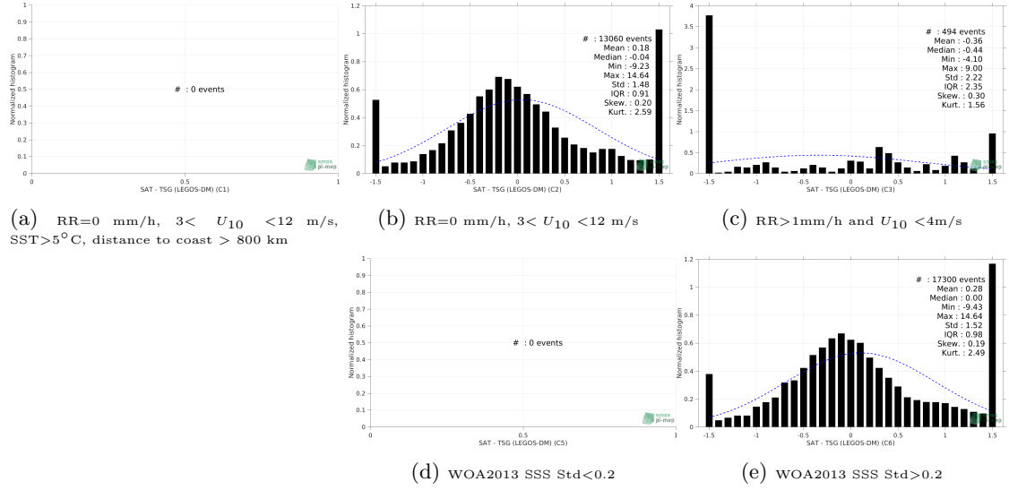
Figure 13: Normalized histogram of \Delta\text{SSS} (SMOS SSS L3 v5 - 9 Days (CATDS-CECOS-LOCEAN) - TSG (LEGOS-DM)) for 5 different subdatasets corresponding to: RR=0 mm/h, 3 < U_{10} < 12 m/s, SST > 5^\circ\text{C} , distance to coast > 800 km (a), RR=0 mm/h, 3 < U_{10} < 12 m/s (b), RR > 1\text{mm/h} and U_{10} < 4\text{m/s} (c), WOA2013 SSS Std < 0.2 (d), WOA2013 SSS Std > 0.2 (e).
