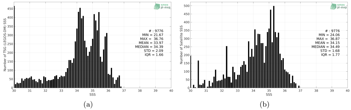
Figure 2: Histograms of SSS from TSG (LEGOS-DM) (a) and SMOS SSS L3 v5 - 9 Days (CATDS-CECOS-LOCEAN) (b) considering all match-up pairs per bins of 0.1 over the Congo river plume Pi-MEP region and for the full satellite product period.
