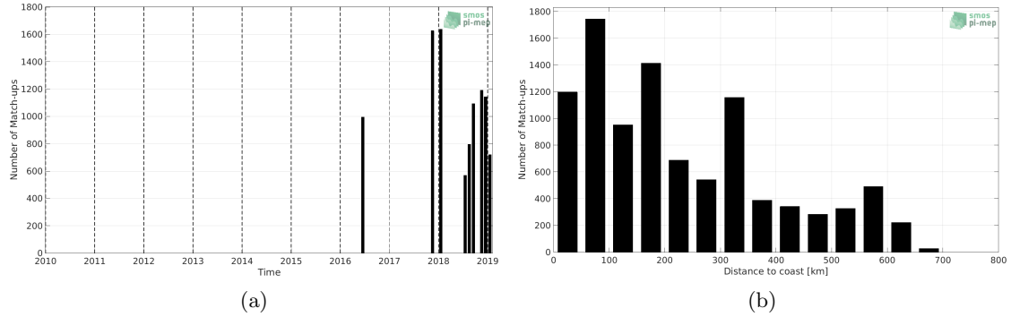
Figure 1: Number of match-ups between TSG (LEGOS-DM) and SMOS SSS L3 v5 - 9 Days (CATDS-CECOS-LOCEAN) SSS as a function of time (a) and as function of the distance to coast (b) over the Congo river plume Pi-MEP region and for the full satellite product period.
