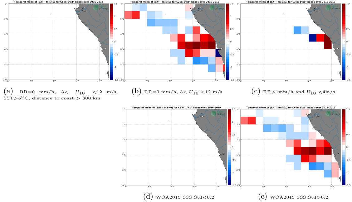
Figure 12: Temporal mean gridded over spatial boxes of size 1^{\circ}\times 1^{\circ} of \Delta\text{SSS} (SMOS SSS L3 v5 - 9 Days (CATDS-CECOS-LOCEAN) - TSG (LEGOS-DM)) for 5 different subdatasets corresponding to:RR=0 mm/h, 3 < U_{10} < 12 m/s, SST >5^{\circ}\text{C} , distance to coast > 800 km (a), RR=0 mm/h, 3 < U_{10} < 12 m/s (b), RR >1 mm/h and U_{10} < 4 m/s (c), WOA2013 SSS Std <0.2 (d), WOA2013 SSS Std >0.2 (e).
