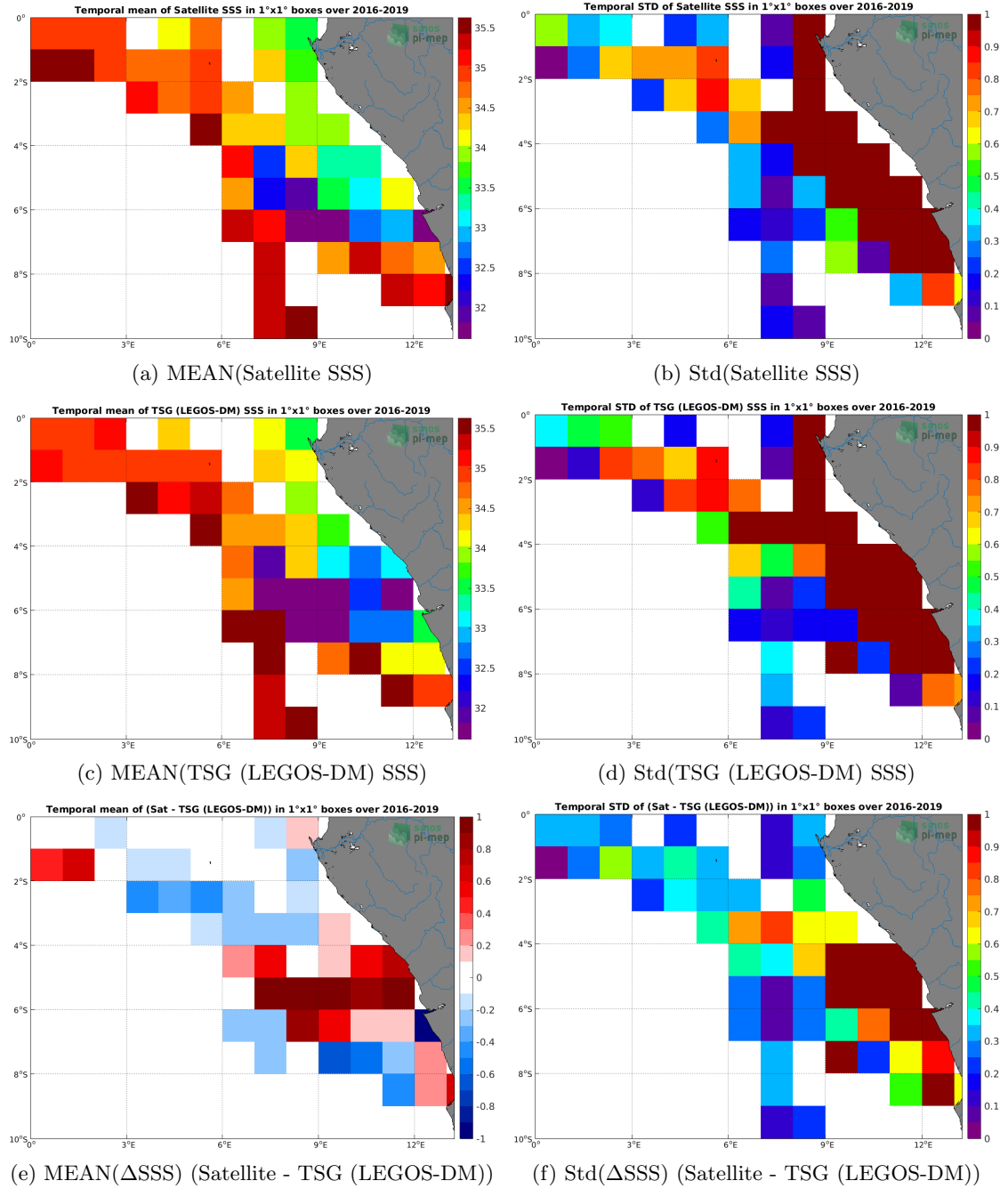
Figure 6: Temporal mean (left) and Std (right) of SSS from SMOS SSS L3 v5 - 9 Days (CATDS-CECOS-LOCEAN) (top), TSG (LEGOS-DM) (middle), and of \Delta SSS (Satellite - TSG (LEGOS-DM)). Only match-up pairs are used to generate these maps.
