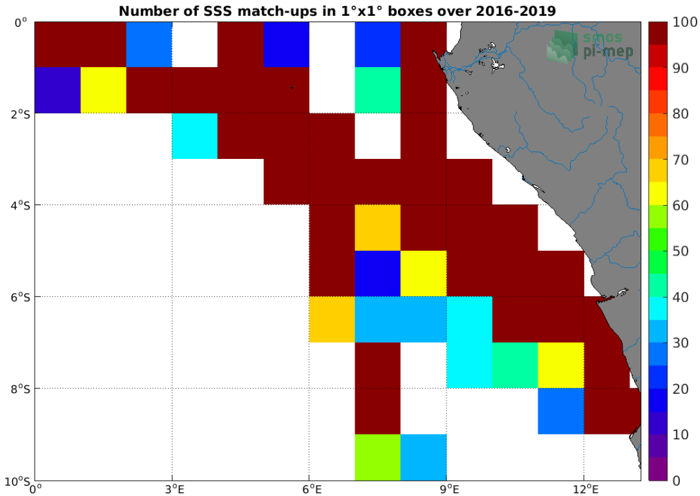
Figure 4: Number of SSS match-ups between TSG (LEGOS-DM) SSS and the SMOS SSS L3 v5 - 9 Days (CATDS-CECOS-LOCEAN) SSS product for the Congo river plume Pi-MEP region over 1^\circ \times 1^\circ boxes and for the full satellite product period.
