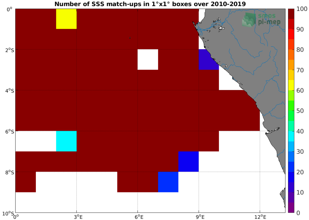
Figure 4: Number of SSS match-ups between TSG (GOSUD-Research-vessel) SSS and the SMOS SSS L3 v5 - 9 Days (CATDS-CECOS-LOCEAN) SSS product for the Congo river plume Pi-MEP region over 1^\circ \times 1^\circ boxes and for the full satellite product period.
