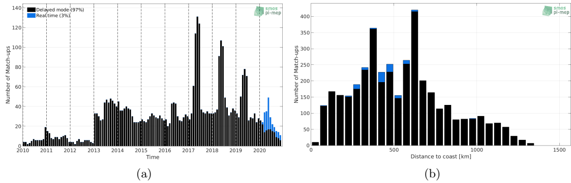
Figure 1: Number of match-ups between Argo and SMOS SSS L3 v5 - 9 Days (CATDS-CECOS-LOCEAN) SSS as a function of time (a) and as function of the distance to coast (b) over the Congo river plume Pi-MEP region and for the full satellite product period.
