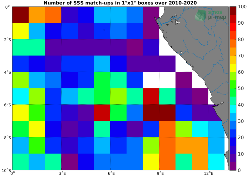
Figure 4: Number of SSS match-ups between Argo SSS and the SMOS SSS L3 v5 - 9 Days (CATDS-CECOS-LOCEAN) SSS product for the Congo river plume Pi-MEP region over 1^\circ \times 1^\circ boxes and for the full satellite product period.
