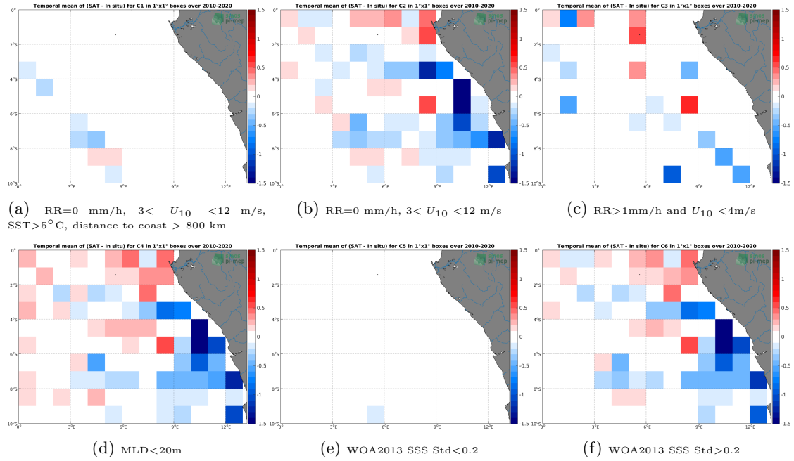
Figure 12: Temporal mean gridded over spatial boxes of size 1^\circ \times 1^\circ of \Delta SSS (SMOS SSS L3 v5 - 9 Days (CATDS-CECOS-LOCEAN) - Argo) for 6 different subdatasets corresponding to:RR=0 mm/h, 3 < U_{10} < 12 m/s, SST >5^\circ C, distance to coast > 800 km (a), RR=0 mm/h, 3 < U_{10} < 12 m/s (b), RR >1 mm/h and U_{10} < 4 m/s (c),MLD <20 m (d),WOA2013 SSS Std <0.2 (e),WOA2013 SSS Std >0.2 (f).
