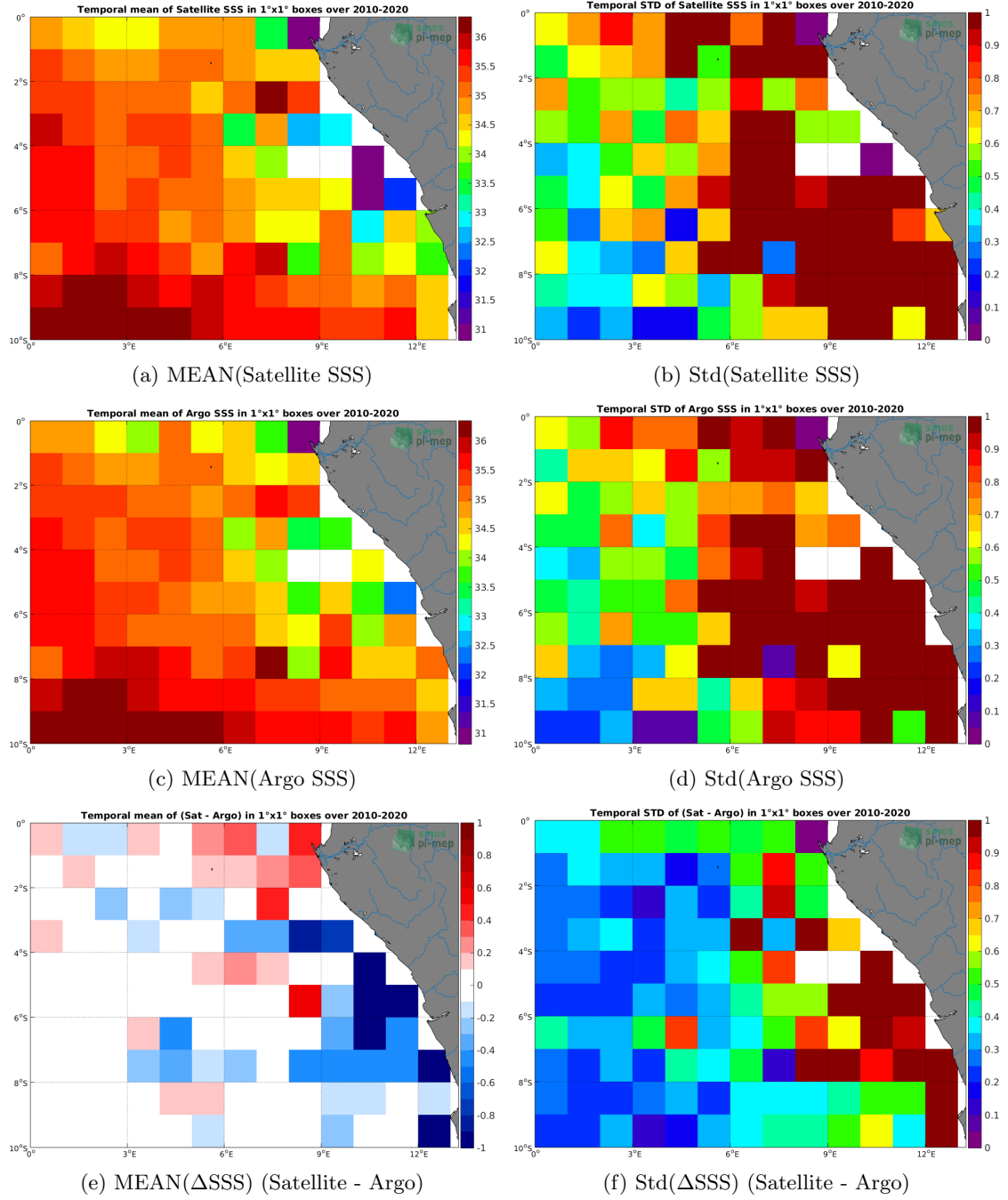
Figure 6: Temporal mean (left) and Std (right) of SSS from SMOS SSS L3 v5 - 9 Days (CATDS-CECOS-LOCEAN) (top), Argo (middle), and of \Delta SSS (Satellite - Argo). Only match-up pairs are used to generate these maps.
