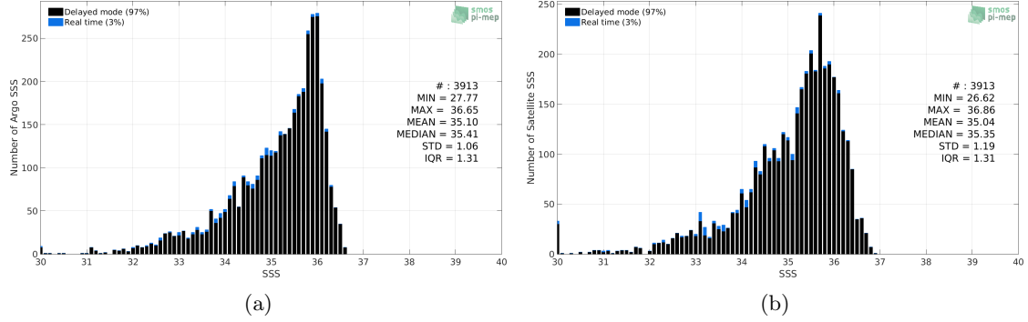
Figure 2: Histograms of SSS from Argo (a) and SMOS SSS L3 v5 - 9 Days (CATDS-CECOS-LOCEAN) (b) considering all match-up pairs per bins of 0.1 over the Congo river plume Pi-MEP region and for the full satellite product period.
