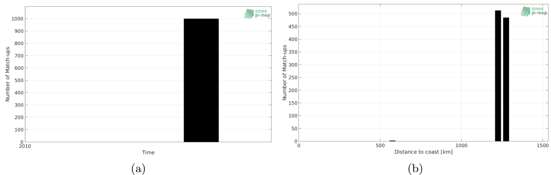
Figure 1: Number of match-ups between TSG (SAMOS) and SMOS SSS L3 v5 - 18 Days (CATDS-CECOS-LOCEAN) SSS as a function of time (a) and as function of the distance to coast (b) over the Congo river plume Pi-MEP region and for the full satellite product period.
