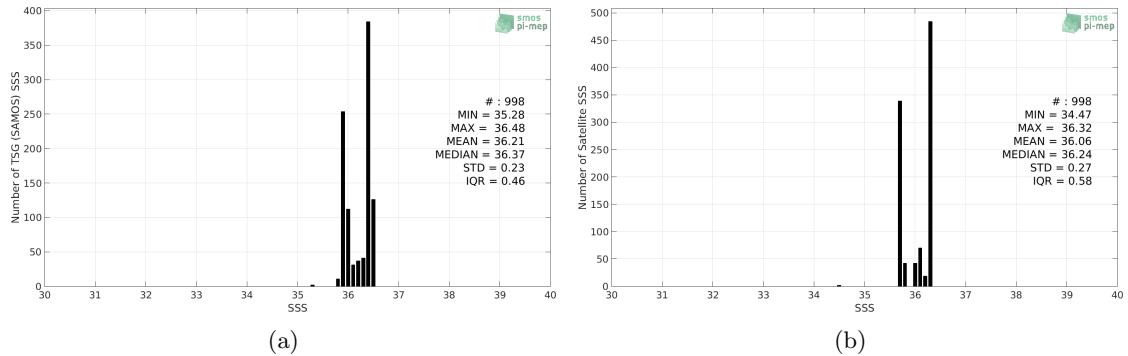
Figure 2: Histograms of SSS from TSG (SAMOS) (a) and SMOS SSS L3 v5 - 18 Days (CATDS-CECOS-LOCEAN) (b) considering all match-up pairs per bins of 0.1 over the Congo river plume Pi-MEP region and for the full satellite product period.
