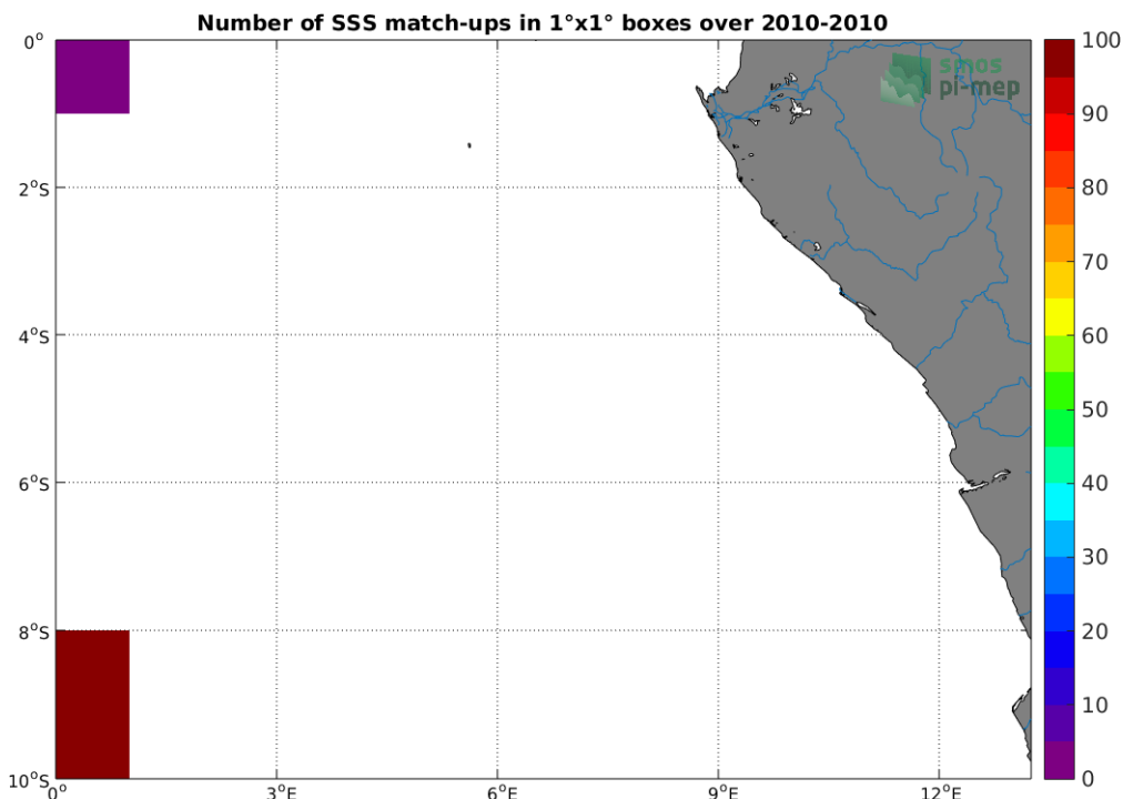
Figure 4: Number of SSS match-ups between TSG (SAMOS) SSS and the SMOS SSS L3 v5 - 18 Days (CATDS-CECOS-LOCEAN) SSS product for the Congo river plume Pi-MEP region over 1^\circ \times 1^\circ boxes and for the full satellite product period.
