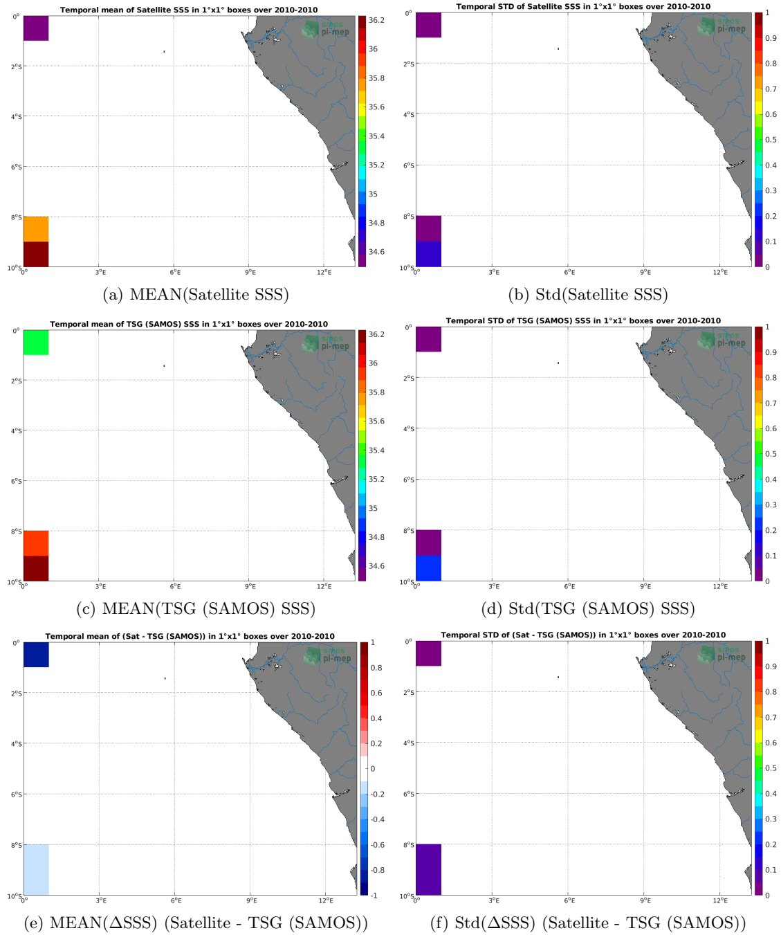
Figure 6: Temporal mean (left) and Std (right) of SSS from SMOS SSS L3 v5 - 18 Days (CATDS-CECOS-LOCEAN) (top), TSG (SAMOS) (middle), and of \Delta SSS (Satellite - TSG (SAMOS)). Only match-up pairs are used to generate these maps.
