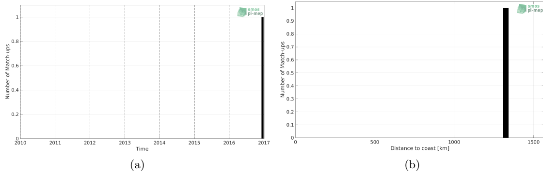
Figure 1: Number of match-ups between TSG (Polarstern) and SMOS SSS L3 v5 - 18 Days (CATDS-CECOS-LOCEAN) SSS as a function of time (a) and as function of the distance to coast (b) over the Congo river plume Pi-MEP region and for the full satellite product period.
