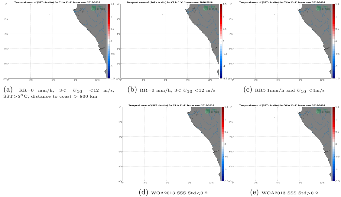
Figure 12: Temporal mean gridded over spatial boxes of size 1^{\circ}\times 1^{\circ} of \Delta\text{SSS} (SMOS SSS L3 v5 - 18 Days (CATDS-CECOS-LOCEAN) - TSG (Polarstern)) for 5 different subdatasets corresponding to:RR=0 mm/h, 3 < U_{10} < 12 m/s, SST >5^{\circ}\text{C} , distance to coast > 800 km (a), RR=0 mm/h, 3 < U_{10} < 12 m/s (b), RR >1 mm/h and U_{10} < 4 m/s (c), WOA2013 SSS Std <0.2 (d), WOA2013 SSS Std >0.2 (e).
