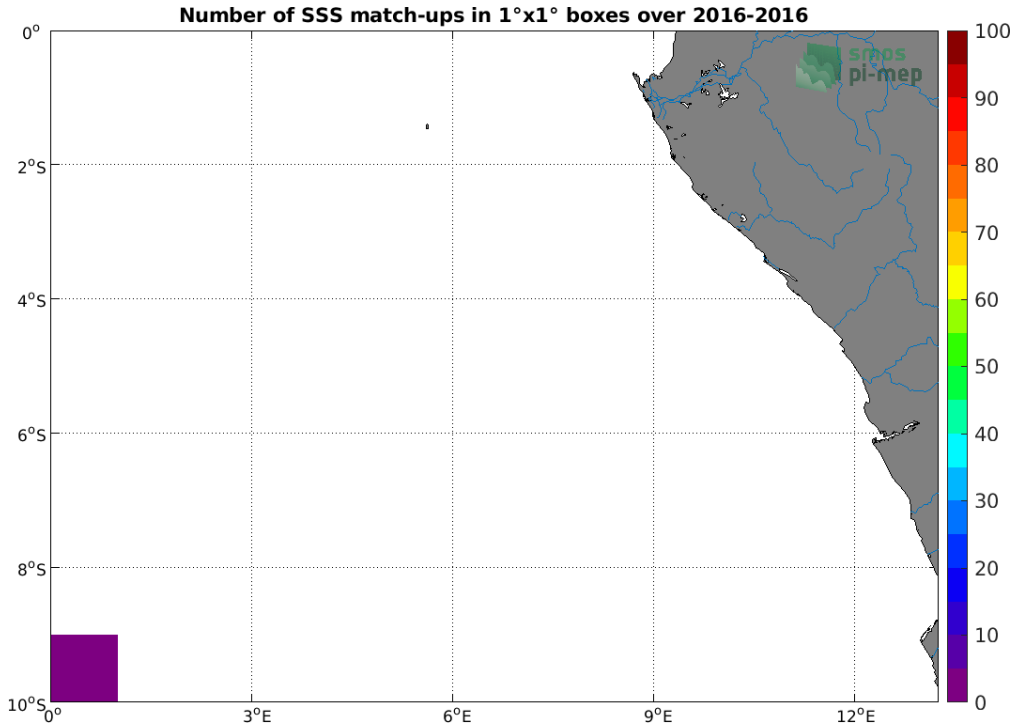
Figure 4: Number of SSS match-ups between TSG (Polarstern) SSS and the SMOS SSS L3 v5 - 18 Days (CATDS-CECOS-LOCEAN) SSS product for the Congo river plume Pi-MEP region over 1°x1° boxes and for the full satellite product period.
