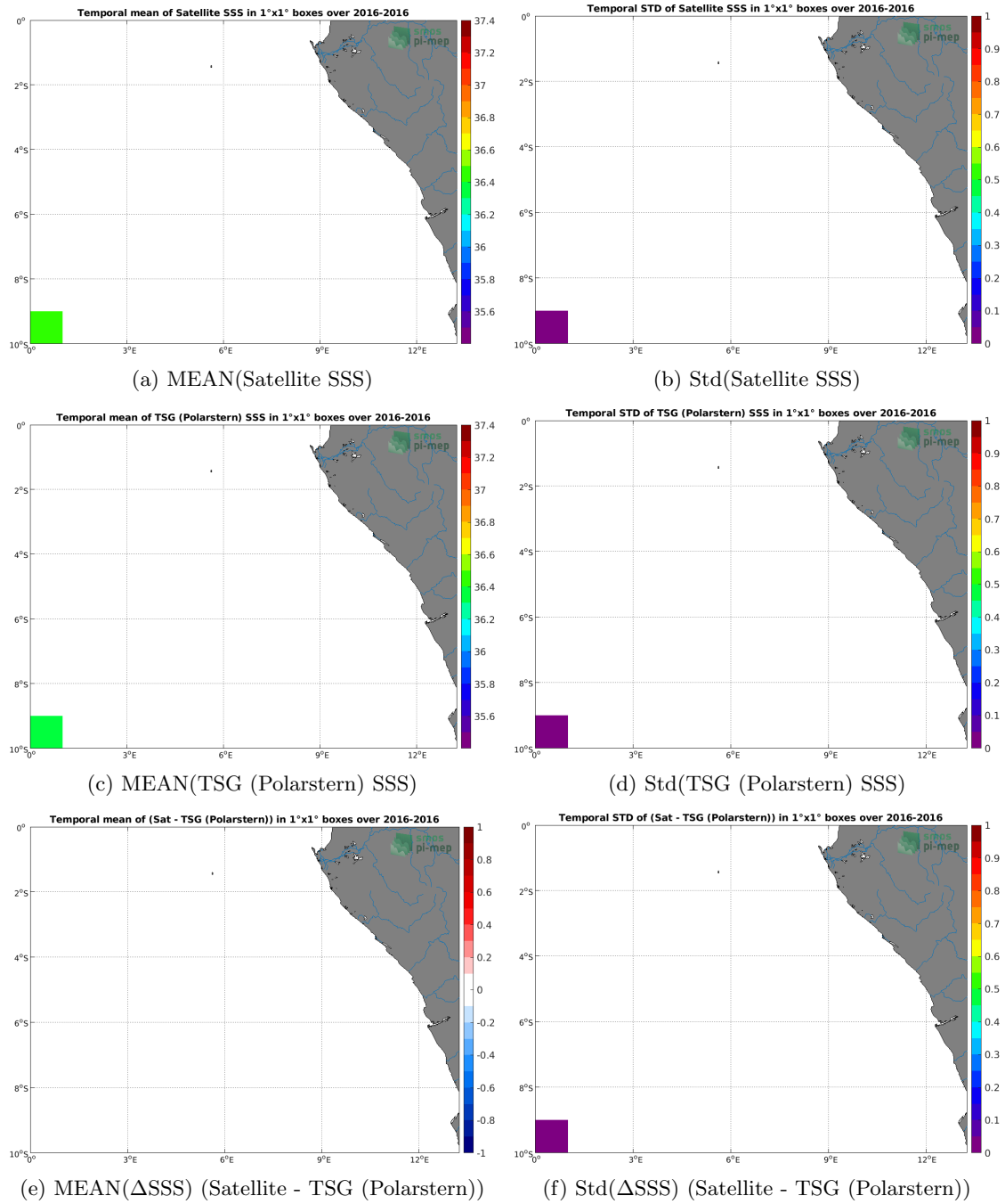
Figure 6: Temporal mean (left) and Std (right) of SSS from SMOS SSS L3 v5 - 18 Days (CATDS-CECOS-LOCEAN) (top), TSG (Polarstern) (middle), and of \Delta SSS (Satellite - TSG (Polarstern)). Only match-up pairs are used to generate these maps.
