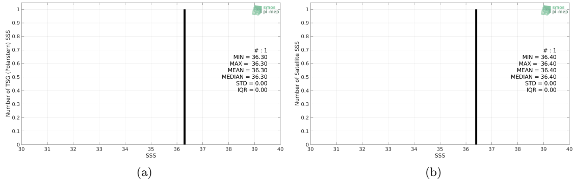
Figure 2: Histograms of SSS from TSG (Polarstern) (a) and SMOS SSS L3 v5 - 18 Days (CATDS-CECOS-LOCEAN) (b) considering all match-up pairs per bins of 0.1 over the Congo river plume Pi-MEP region and for the full satellite product period.
