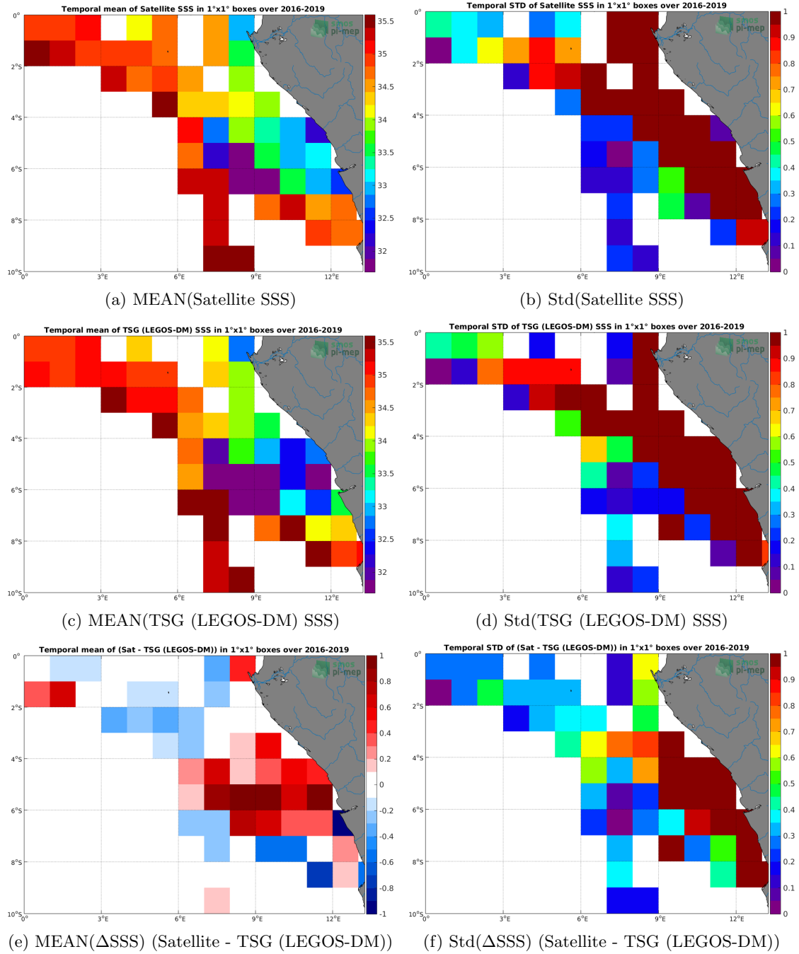
Figure 6: Temporal mean (left) and Std (right) of SSS from SMOS SSS L3 v5 - 18 Days (CATDS-CECOS-LOCEAN) (top), TSG (LEGOS-DM) (middle), and of \Delta SSS (Satellite - TSG (LEGOS-DM)). Only match-up pairs are used to generate these maps.
