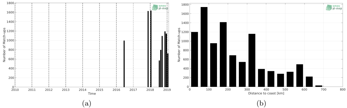
Figure 1: Number of match-ups between TSG (LEGOS-DM) and SMOS SSS L3 v5 - 18 Days (CATDS-CECOS-LOCEAN) SSS as a function of time (a) and as function of the distance to coast (b) over the Congo river plume Pi-MEP region and for the full satellite product period.
