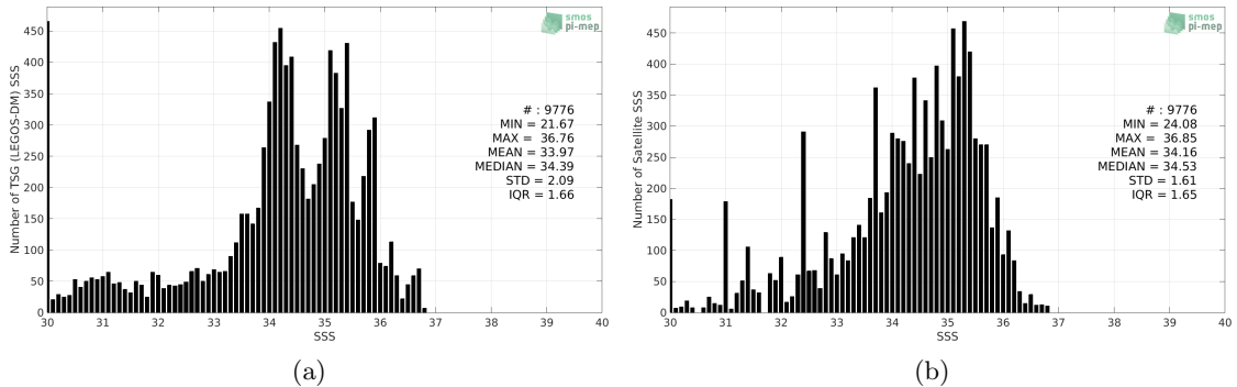
Figure 2: Histograms of SSS from TSG (LEGOS-DM) (a) and SMOS SSS L3 v5 - 18 Days (CATDS-CECOS-LOCEAN) (b) considering all match-up pairs per bins of 0.1 over the Congo river plume Pi-MEP region and for the full satellite product period.
