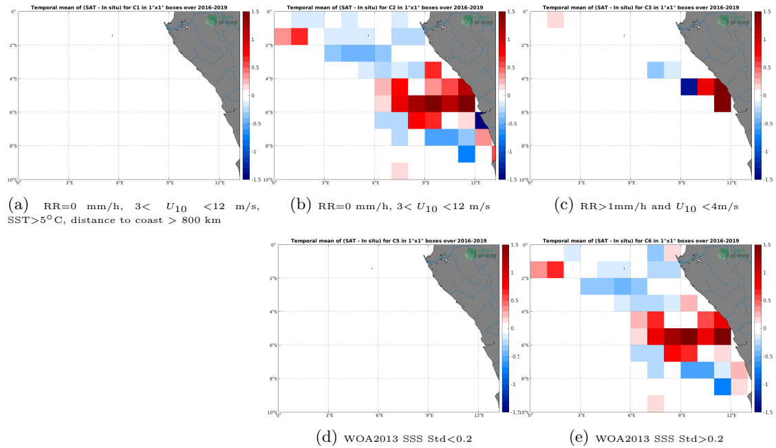
Figure 12: Temporal mean gridded over spatial boxes of size 1^{\circ}\times 1^{\circ} of \Delta\text{SSS} (SMOS SSS L3 v5 - 18 Days (CATDS-CECOS-LOCEAN) - TSG (LEGOS-DM)) for 5 different subdatasets corresponding to:RR=0 mm/h, 3 < U_{10} < 12 m/s, SST > 5^{\circ}\text{C} , distance to coast > 800 km (a), RR=0 mm/h, 3 < U_{10} < 12 m/s (b), RR > 1 mm/h and U_{10} < 4 m/s (c), WOA2013 SSS Std < 0.2 (d), WOA2013 SSS Std > 0.2 (e).
