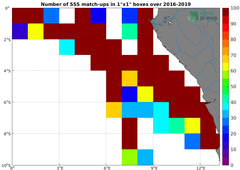
Figure 4: Number of SSS match-ups between TSG (LEGOS-DM) SSS and the SMOS SSS L3 v5 - 18 Days (CATDS-CECOS-LOCEAN) SSS product for the Congo river plume Pi-MEP region over 1^\circ \times 1^\circ boxes and for the full satellite product period.
