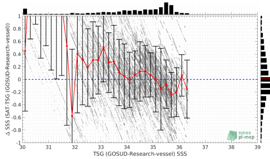
(a) TSG (GOSUD-Research-vessel) SSS
