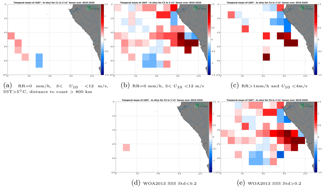
Figure 12: Temporal mean gridded over spatial boxes of size 1^\circ \times 1^\circ of \Delta SSS (SMOS SSS L3 v5 - 18 Days (CATDS-CECOS-LOCEAN) - TSG (GOSUD-Research-vessel)) for 5 different sub-datasets corresponding to:RR=0 mm/h, 3 < U_{10} < 12 m/s, SST >5^\circ\text{C} , distance to coast > 800 km (a), RR=0 mm/h, 3 < U_{10} < 12 m/s (b), RR >1 mm/h and U_{10} < 4 m/s (c), WOA2013 SSS Std <0.2 (d), WOA2013 SSS Std >0.2 (e).
