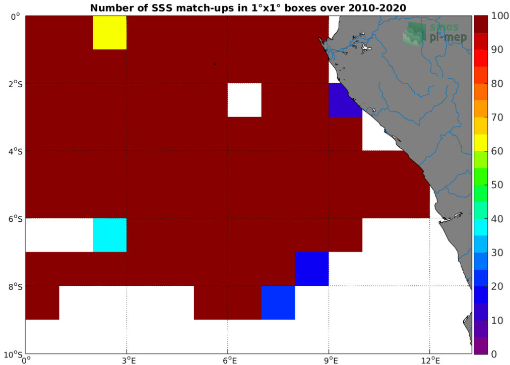
Figure 4: Number of SSS match-ups between TSG (GOSUD-Research-vessel) SSS and the SMOS SSS L3 v5 - 18 Days (CATDS-CECOS-LOCEAN) SSS product for the Congo river plume Pi-MEP region over 1^{\circ} \times 1^{\circ} boxes and for the full satellite product period.
