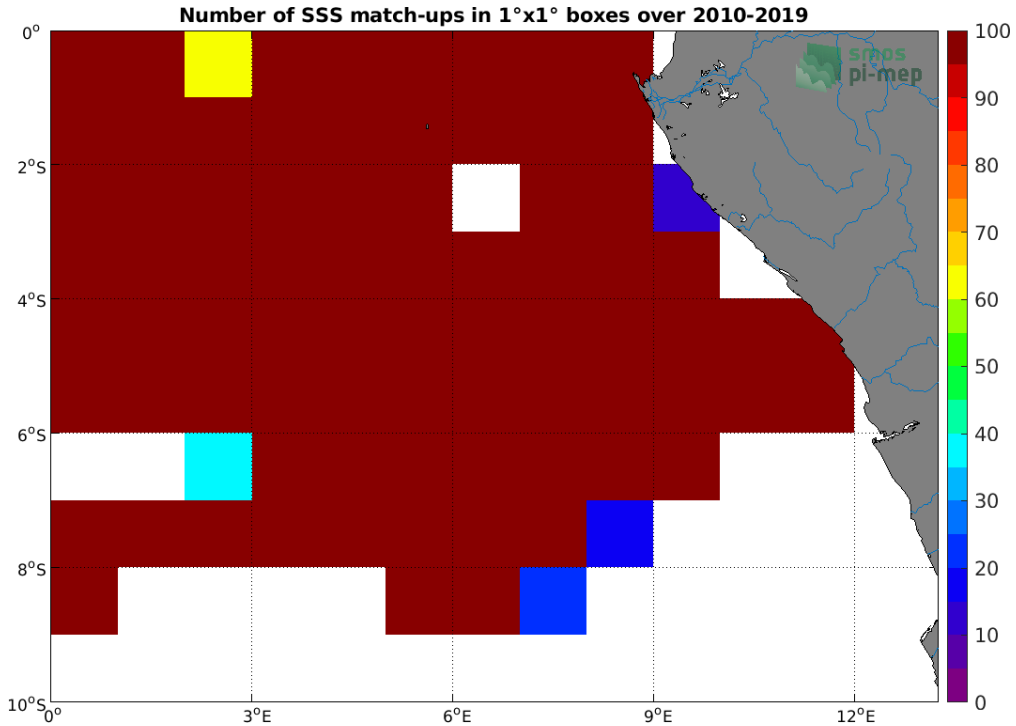
Figure 4: Number of SSS match-ups between TSG (GOSUD-Research-vessel) SSS and the SMOS SSS L3 v5 - 18 Days (CATDS-CECOS-LOCEAN) SSS product for the Congo river plume Pi-MEP region over 1^\circ \times 1^\circ boxes and for the full satellite product period.
