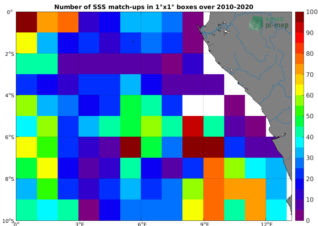
Figure 4: Number of SSS match-ups between Argo SSS and the SMOS SSS L3 v5 - 18 Days (CATDS-CECOS-LOCEAN) SSS product for the Congo river plume Pi-MEP region over 1°x1° boxes and for the full satellite product period.
