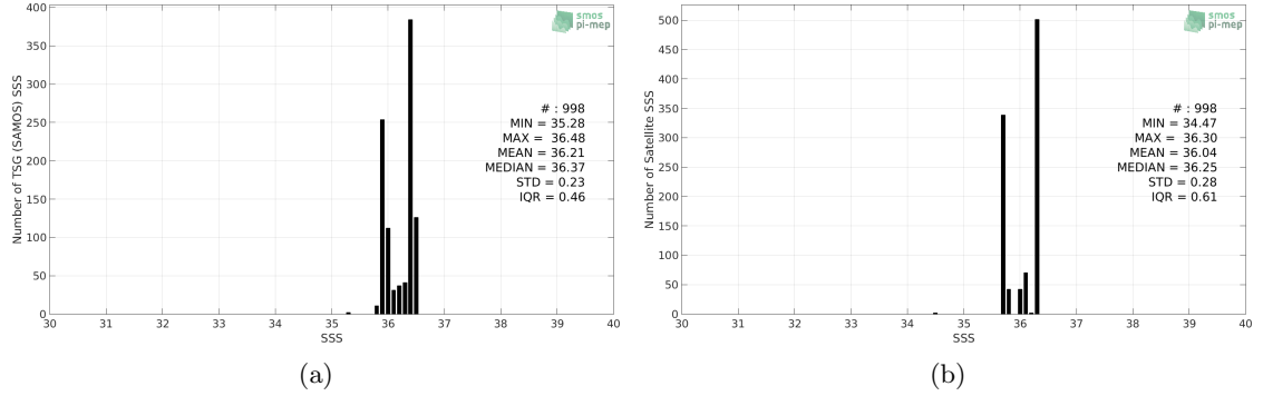
Figure 2: Histograms of SSS from TSG (SAMOS) (a) and SMOS SSS L3 v4 - 18 Days (CATDS-CECOS-LOCEAN) (b) considering all match-up pairs per bins of 0.1 over the Congo river plume Pi-MEP region and for the full satellite product period.
