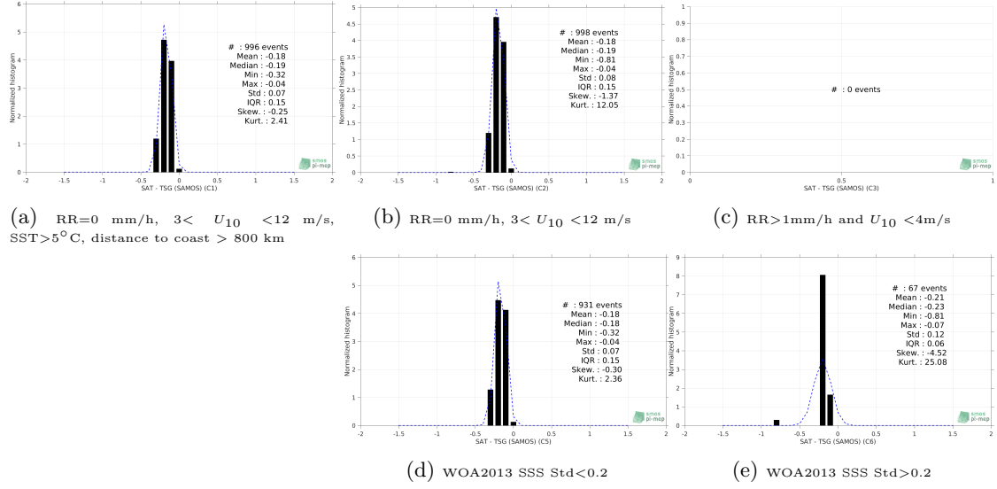
Figure 13: Normalized histogram of \Delta SSS (SMOS SSS L3 v4 - 18 Days (CATDS-CECOS-LOCEAN) - TSG (SAMOS)) for 5 different subdatasets corresponding to: RR=0 mm/h, 3 < U_{10} < 12 m/s, SST>5°C, distance to coast > 800 km (a), RR=0 mm/h, 3 < U_{10} < 12 m/s (b), RR>1mm/h and U_{10} < 4 m/s (c), WOA2013 SSS Std<0.2 (d), WOA2013 SSS Std>0.2 (e).
