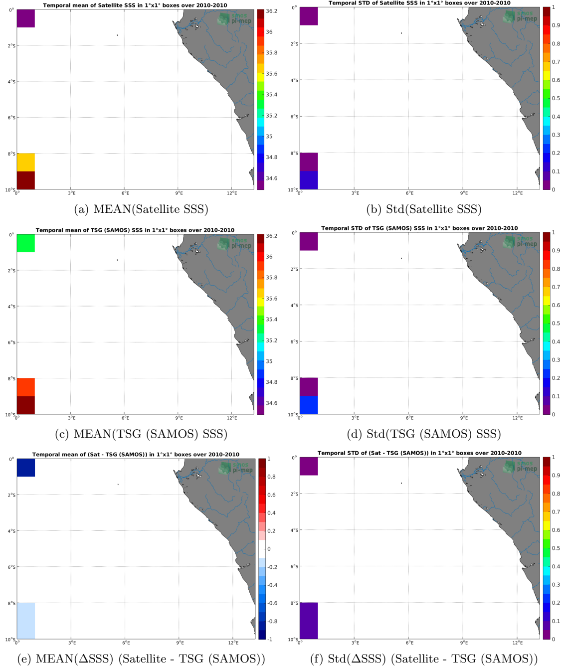
Figure 6: Temporal mean (left) and Std (right) of SSS from SMOS SSS L3 v4 - 18 Days (CATDS-CECOS-LOCEAN) (top), TSG (SAMOS) (middle), and of \Delta SSS (Satellite - TSG (SAMOS)). Only match-up pairs are used to generate these maps.
