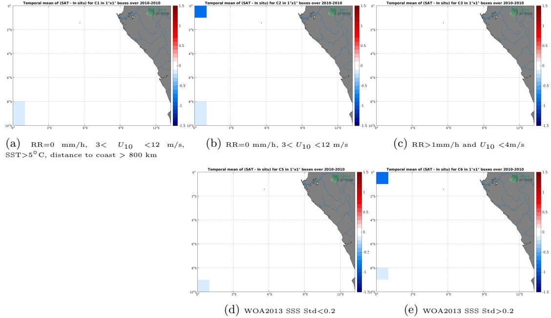
Figure 12: Temporal mean gridded over spatial boxes of size 1^{\circ}\times 1^{\circ} of \Delta\text{SSS} (SMOS SSS L3 v4 - 18 Days (CATDS-CECOS-LOCEAN) - TSG (SAMOS)) for 5 different subdatasets corresponding to:RR=0 mm/h, 3 < U_{10} < 12 m/s, SST >5^{\circ}\text{C} , distance to coast > 800 km (a), RR=0 mm/h, 3 < U_{10} < 12 m/s (b), RR >1 mm/h and U_{10} < 4 m/s (c), WOA2013 SSS Std <0.2 (d), WOA2013 SSS Std >0.2 (e).
