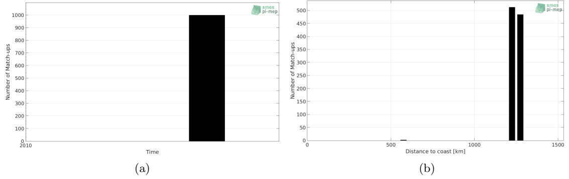
Figure 1: Number of match-ups between TSG (SAMOS) and SMOS SSS L3 v4 - 18 Days (CATDS-CECOS-LOCEAN) SSS as a function of time (a) and as function of the distance to coast (b) over the Congo river plume Pi-MEP region and for the full satellite product period.
