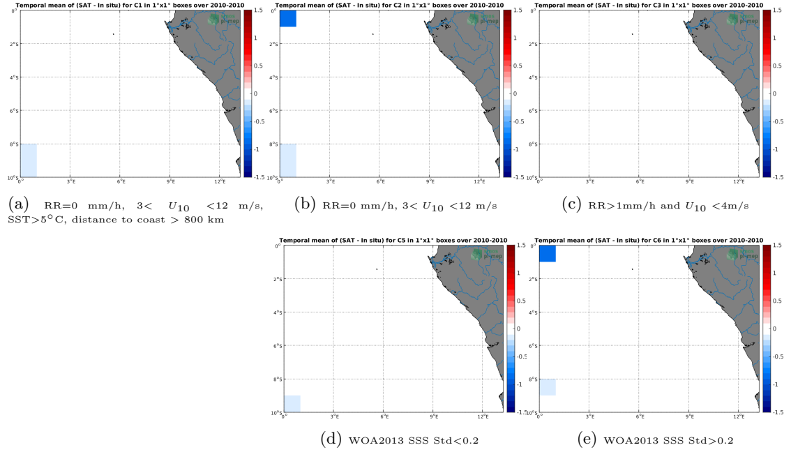
Figure 12: Temporal mean gridded over spatial boxes of size 1^\circ \times 1^\circ of \Delta SSS (SMOS-L3-CATDS-CECOS-LOCEAN-V4-18DAYS-25KM - TSG-SAMOS) for 5 different subdatasets corresponding to: RR=0 mm/h, 3 < U_{10} < 12 m/s, SST >5^\circ C, distance to coast > 800 km (a), RR=0 mm/h, 3 < U_{10} < 12 m/s (b), RR >1 mm/h and U_{10} < 4 m/s (c), WOA2013 SSS Std <0.2 (d), WOA2013 SSS Std >0.2 (e).
