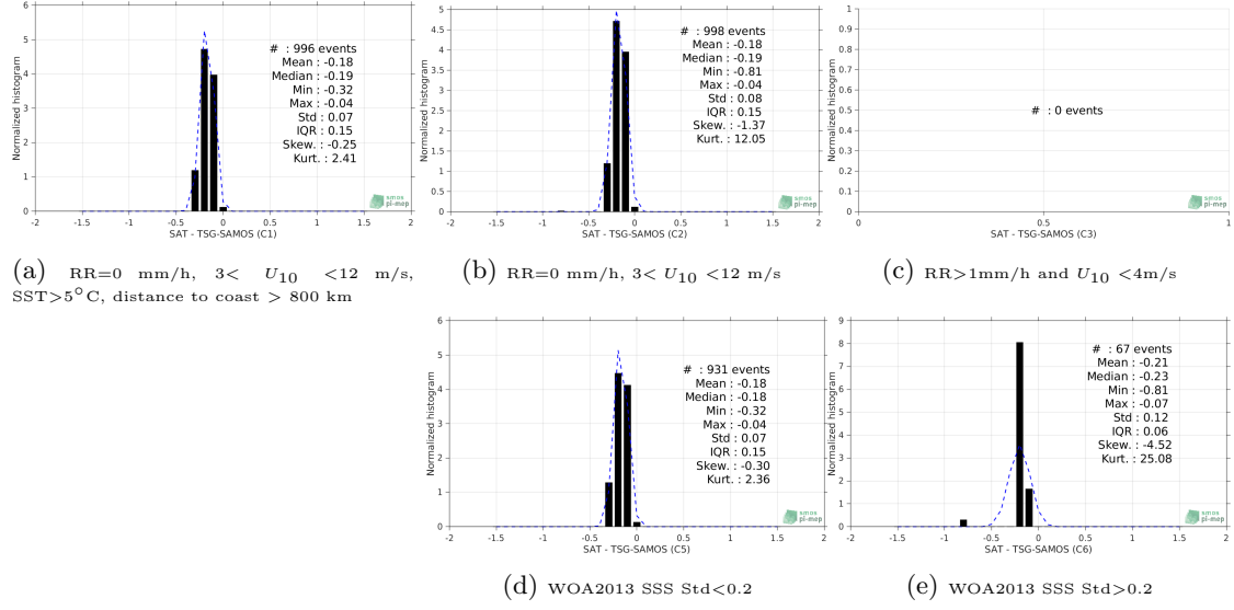
Figure 13: Normalized histogram of \Delta SSS (SMOS-L3-CATDS-CECOS-LOCEAN-V4-18DAYS-25KM - TSG-SAMOS) for 5 different subdatasets corresponding to: RR=0 mm/h, 3 < U_{10} < 12 m/s, SST > 5^\circ C , distance to coast > 800 km (a), RR=0 mm/h, 3 < U_{10} < 12 m/s (b), RR > 1 mm/h and U_{10} < 4 m/s (c), WOA2013 SSS Std < 0.2 (d), WOA2013 SSS Std > 0.2 (e).
