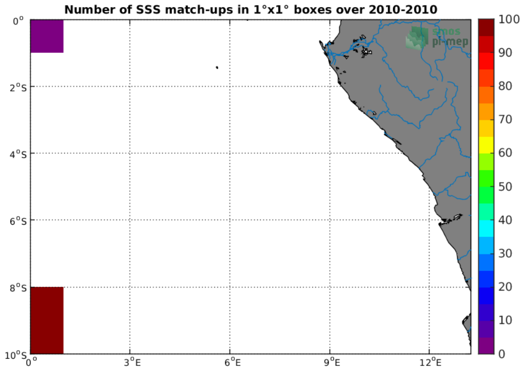
Figure 4: Number of SSS match-ups between TSG-SAMOS SSS and the SMOS-L3-CATDS-CECOS-LOCEAN-V4-18DAYS-25KM SSS product for the Congo river plume Pi-MEP region over 1°x1° boxes and for the full satellite product period.
