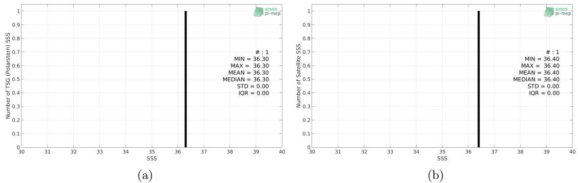
Figure 2: Histograms of SSS from TSG (Polarstern) (a) and SMOS SSS L3 v4 - 18 Days (CATDS-CECOS-LOCEAN) (b) considering all match-up pairs per bins of 0.1 over the Congo river plume Pi-MEP region and for the full satellite product period.
