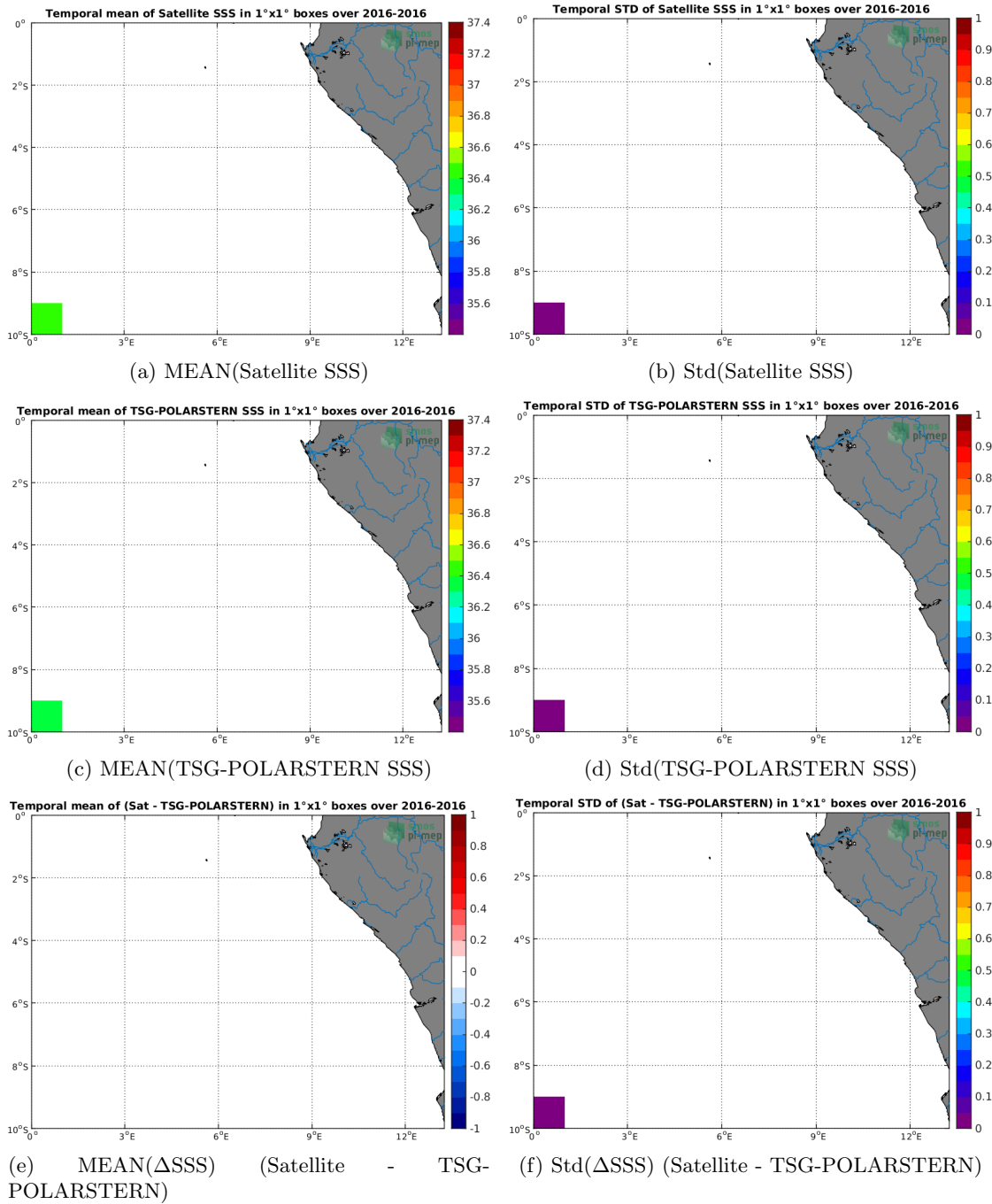
Figure 6: Temporal mean (left) and Std (right) of SSS from SMOS-L3-CATDS-CECOS-LOCEAN-V4-18DAYS-25KM (top), TSG-POLARSTERN (middle), and of \Delta SSS (Satellite - TSG-POLARSTERN). Only match-up pairs are used to generate these maps.
