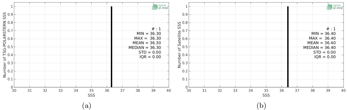
Figure 2: Histograms of SSS from TSG-POLARSTERN (a) and SMOS-L3-CATDS-CECOS-LOCEAN-V4-18DAYS-25KM (b) considering all match-up pairs per bins of 0.1 over the Congo river plume Pi-MEP region and for the full satellite product period.
