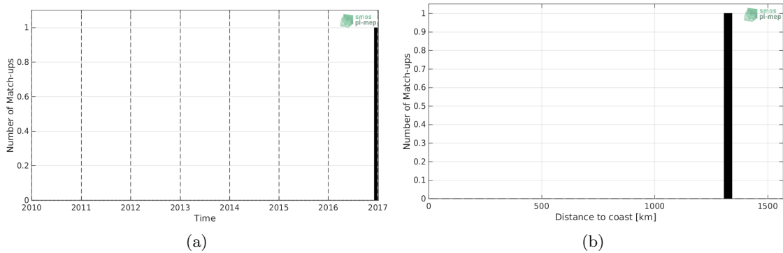
Figure 1: Number of match-ups between TSG-POLARSTERN and SMOS-L3-CATDS-CECOS-LOCEAN-V4-18DAYS-25KM SSS as a function of time (a) and as function of the distance to coast (b) over the Congo river plume Pi-MEP region and for the full satellite product period.
