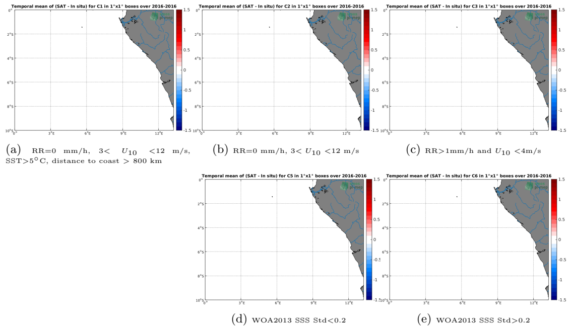
Figure 12: Temporal mean gridded over spatial boxes of size 1^\circ \times 1^\circ of \Delta SSS (SMOS-L3-CATDS-CECOS-LOCEAN-V4-18DAYS-25KM - TSG-POLARSTERN) for 5 different subdatasets corresponding to: RR=0 mm/h, 3 < U_{10} < 12 m/s, SST > 5^\circ\text{C} , distance to coast > 800 km (a), RR=0 mm/h, 3 < U_{10} < 12 m/s (b), RR > 1 mm/h and U_{10} < 4 m/s (c), WOA2013 SSS Std < 0.2 (d), WOA2013 SSS Std > 0.2 (e).
