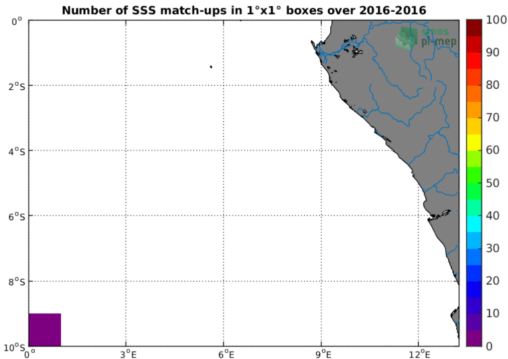
Figure 4: Number of SSS match-ups between TSG-POLARSTERN SSS and the SMOS-L3-CATDS-CECOS-LOCEAN-V4-18DAYS-25KM SSS product for the Congo river plume Pi-MEP region over 1°x1° boxes and for the full satellite product period.
