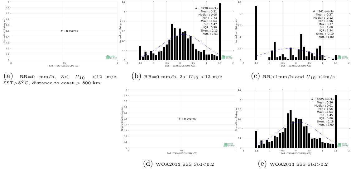
Figure 13: Normalized histogram of \Delta SSS (SMOS SSS L3 v4 - 18 Days (CATDS-CECOS-LOCEAN) - TSG (LEGOS-DM)) for 5 different subdatasets corresponding to: RR=0 mm/h, 3 < U_{10} < 12 m/s, SST > 5°C, distance to coast > 800 km (a), RR=0 mm/h, 3 < U_{10} < 12 m/s (b), RR > 1mm/h and U_{10} < 4 m/s (c), WOA2013 SSS Std < 0.2 (d), WOA2013 SSS Std > 0.2 (e).
