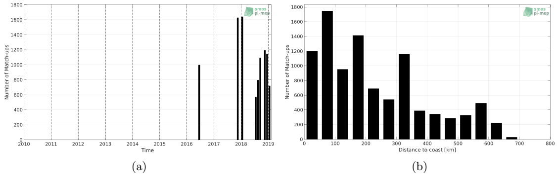
Figure 1: Number of match-ups between TSG (LEGOS-DM) and SMOS SSS L3 v4 - 18 Days (CATDS-CECOS-LOCEAN) SSS as a function of time (a) and as function of the distance to coast (b) over the Congo river plume Pi-MEP region and for the full satellite product period.
