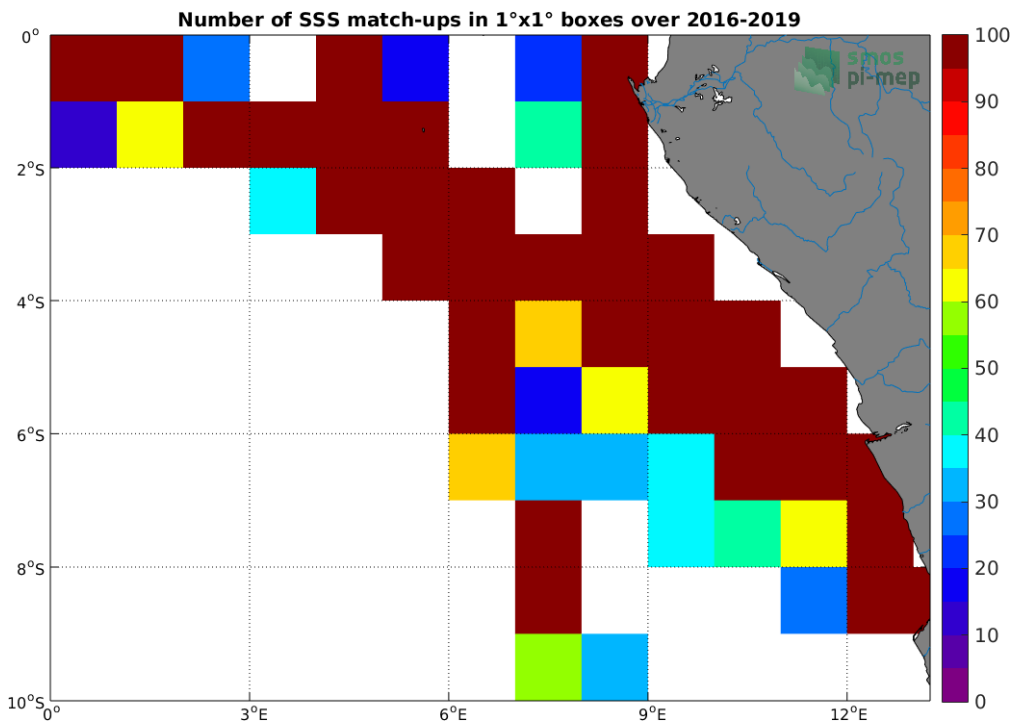
Figure 4: Number of SSS match-ups between TSG (LEGOS-DM) SSS and the SMOS SSS L3 v4 - 18 Days (CATDS-CECOS-LOCEAN) SSS product for the Congo river plume Pi-MEP region over 1^\circ \times 1^\circ boxes and for the full satellite product period.
