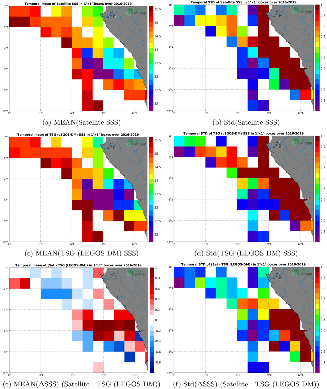
Figure 6: Temporal mean (left) and Std (right) of SSS from SMOS SSS L3 v4 - 18 Days (CATDS-CECOS-LOCEAN) (top), TSG (LEGOS-DM) (middle), and of \Delta SSS (Satellite - TSG (LEGOS-DM)). Only match-up pairs are used to generate these maps.
