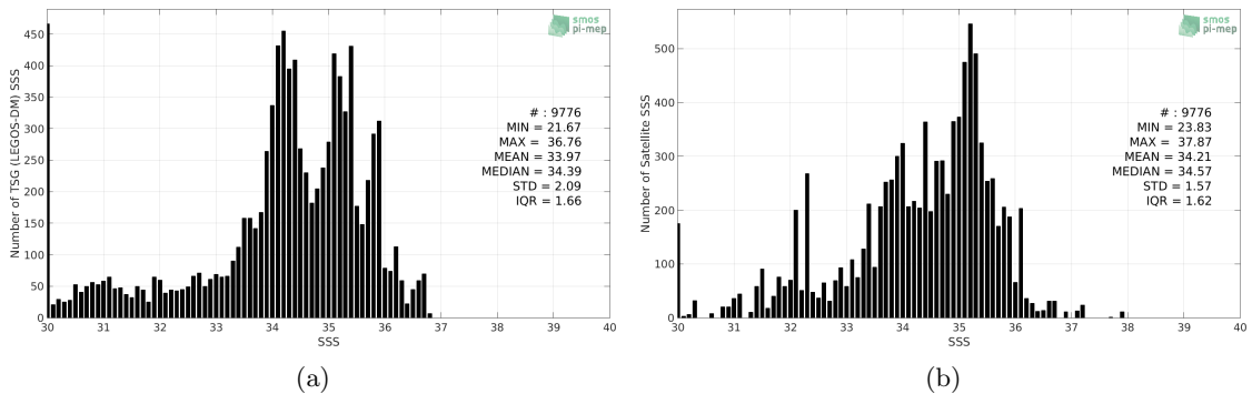
Figure 2: Histograms of SSS from TSG (LEGOS-DM) (a) and SMOS SSS L3 v4 - 18 Days (CATDS-CECOS-LOCEAN) (b) considering all match-up pairs per bins of 0.1 over the Congo river plume Pi-MEP region and for the full satellite product period.
