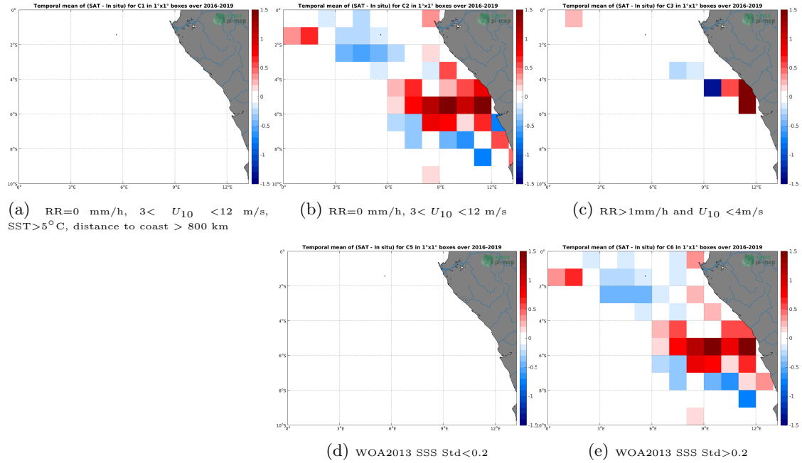
Figure 12: Temporal mean gridded over spatial boxes of size 1^{\circ}\times 1^{\circ} of \Delta\text{SSS} (SMOS SSS L3 v4 - 18 Days (CATDS-CECOS-LOCEAN) - TSG (LEGOS-DM)) for 5 different subdatasets corresponding to:RR=0 mm/h, 3 < U_{10} < 12 m/s, SST >5^{\circ}\text{C} , distance to coast > 800 km (a), RR=0 mm/h, 3 < U_{10} < 12 m/s (b), RR >1 mm/h and U_{10} < 4 m/s (c), WOA2013 SSS Std <0.2 (d), WOA2013 SSS Std >0.2 (e).
