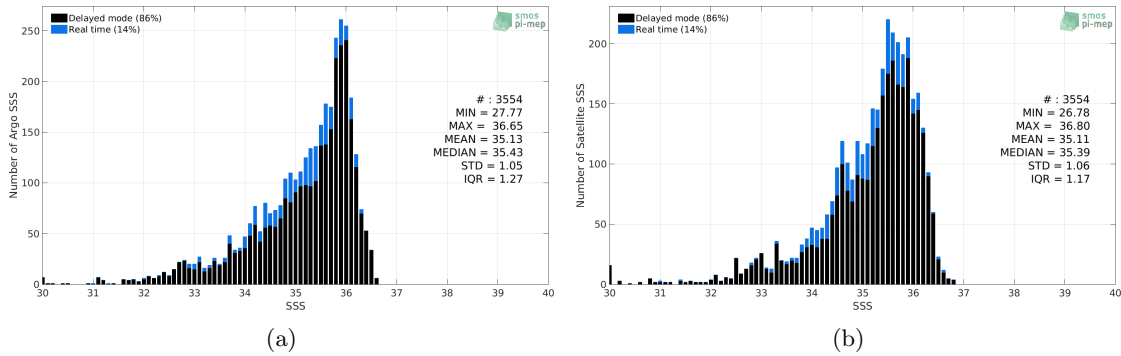
Figure 2: Histograms of SSS from Argo (a) and SMOS SSS L3 v4 - 18 Days (CATDS-CECOS-LOCEAN) (b) considering all match-up pairs per bins of 0.1 over the Congo river plume Pi-MEP region and for the full satellite product period.
