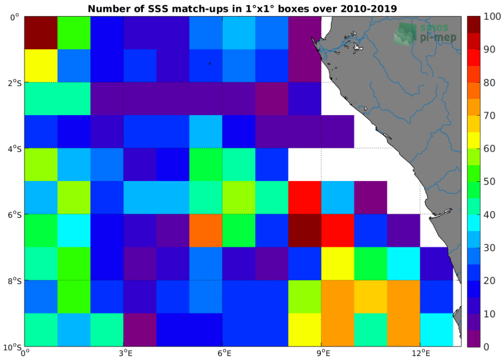
Figure 4: Number of SSS match-ups between Argo SSS and the SMOS SSS L3 v4 - 18 Days (CATDS-CECOS-LOCEAN) SSS product for the Congo river plume Pi-MEP region over 1^\circ \times 1^\circ boxes and for the full satellite product period.
