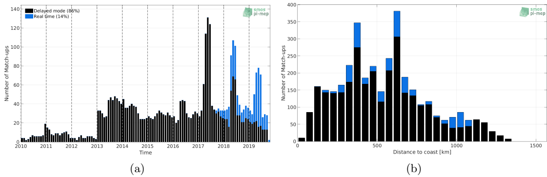
Figure 1: Number of match-ups between Argo and SMOS SSS L3 v4 - 18 Days (CATDS-CECOS-LOCEAN) SSS as a function of time (a) and as function of the distance to coast (b) over the Congo river plume Pi-MEP region and for the full satellite product period.
