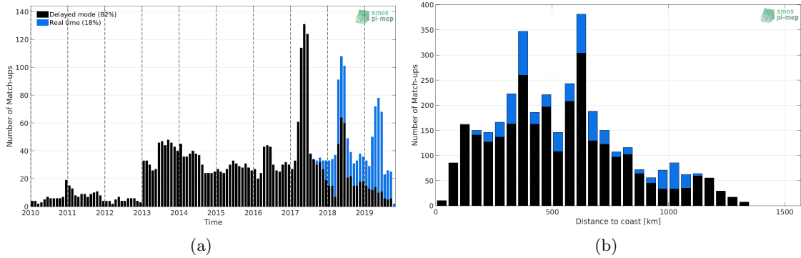
Figure 1: Number of match-ups between Argo and SMOS-L3-CATDS-CECOS-LOCEAN-V4-18DAYS-25KM SSS as a function of time (a) and as function of the distance to coast (b) over the Congo river plume Pi-MEP region and for the full satellite product period.
