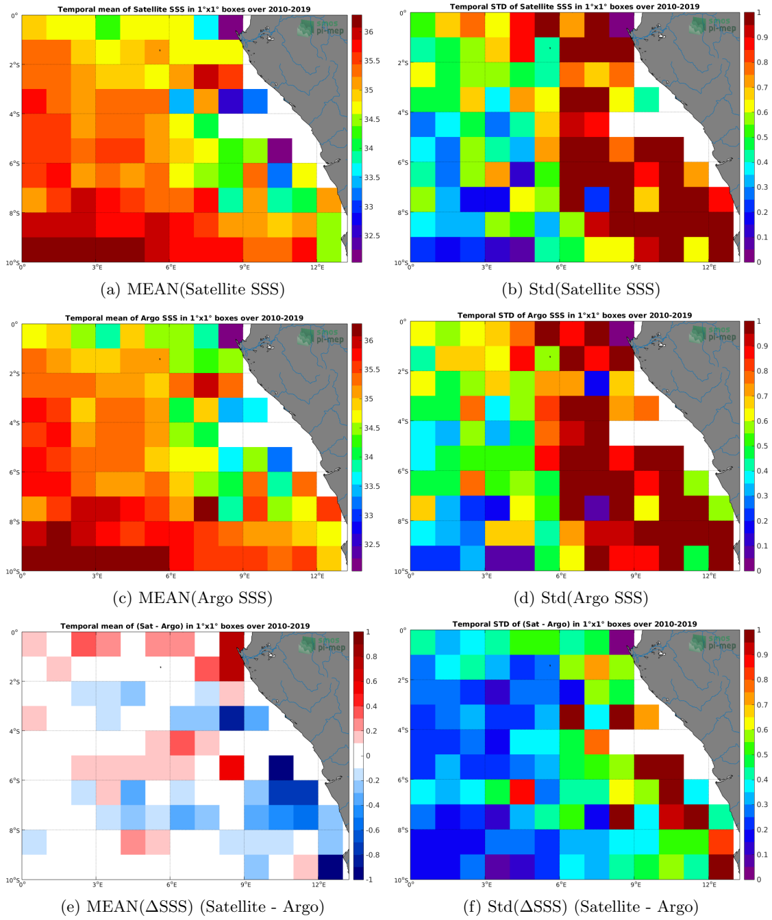
Figure 6: Temporal mean (left) and Std (right) of SSS from SMOS-L3-CATDS-CECOS-LOCEAN-V4-18DAYS-25KM (top), Argo (middle), and of \Delta SSS (Satellite - Argo). Only match-up pairs are used to generate these maps.
