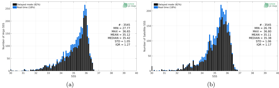
Figure 2: Histograms of SSS from Argo (a) and SMOS-L3-CATDS-CECOS-LOCEAN-V4-18DAYS-25KM (b) considering all match-up pairs per bins of 0.1 over the Congo river plume Pi-MEP region and for the full satellite product period.
