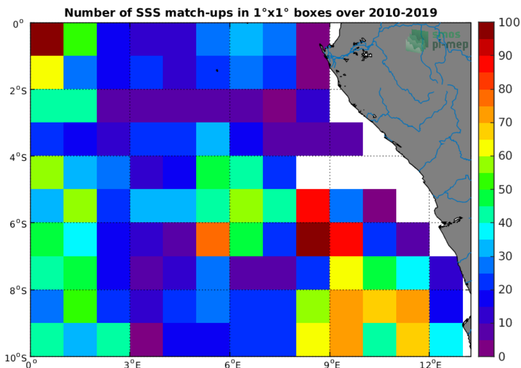
Figure 4: Number of SSS match-ups between Argo SSS and the SMOS-L3-CATDS-CECOS-LOCEAN-V4-18DAYS-25KM SSS product for the Congo river plume Pi-MEP region over 1^\circ \times 1^\circ boxes and for the full satellite product period.
